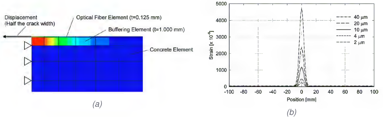
Figure 1-35: (a) Two-dimensional Finite Element model mesh used to model the optical fiber/buffering element/cracked concrete medium. (b) Strain distribution on the sensing segment of the fiber by Finite Element analysis [96].
