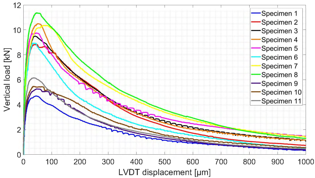
Figure 3-12: The vertical load vs COD diagram for the different Wedge splitting specimen from the two testing campaigns.
