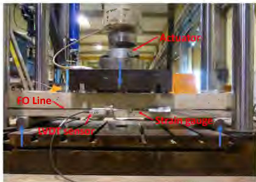
Figure 4-13: Three-point bending test setup.
