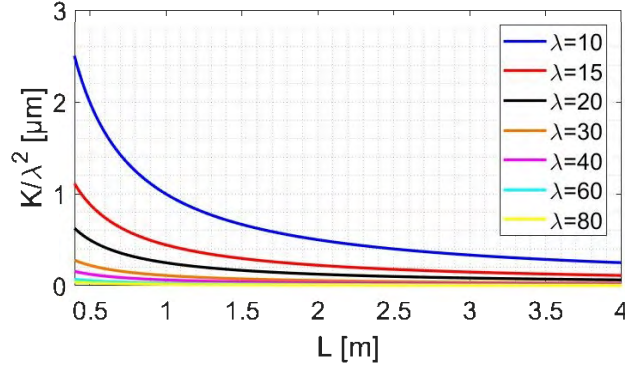
Figure 2-14: Variation of the additional term ( K/\lambda^2 ) in the crack-induced strain \epsilon_{f,crack} distribution in function of the span L for different strain lag parameter \lambda values.
