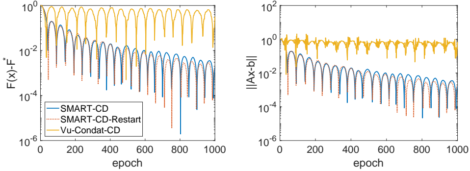
Figure 3.4: The convergence behavior of SMART-CD (Algorithm 8) and Vu-Condat-CD (Algorithm 6) for a degenerate linear program with repeated constraints. We observe that degeneracy of the problem prevents Vu-Condat-CD from making any progress towards the solution (we only proved O(1/\sqrt{k}) speed of convergence for Algorithm 6), while SMART-CD preserves O(1/k) rate as predicted by theory.
