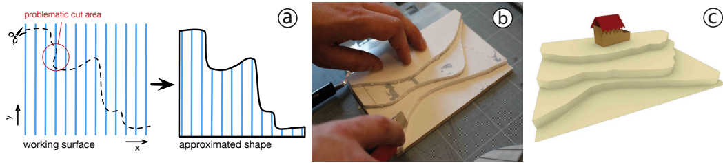
Figure 8: Overview of the ShapeMe [W TM 18] technology. We approximate 2D shape by using a grid of length-aware sensors. The red circle highlights the part of the cutting path that is not accurately captured by this sensing topology (a). The approach allows makers to craft physical models that consists of multiple shape-aware layers (b). The geometry of the model is constantly captured and rendered in 3D modeling software, such as Blender (c).
