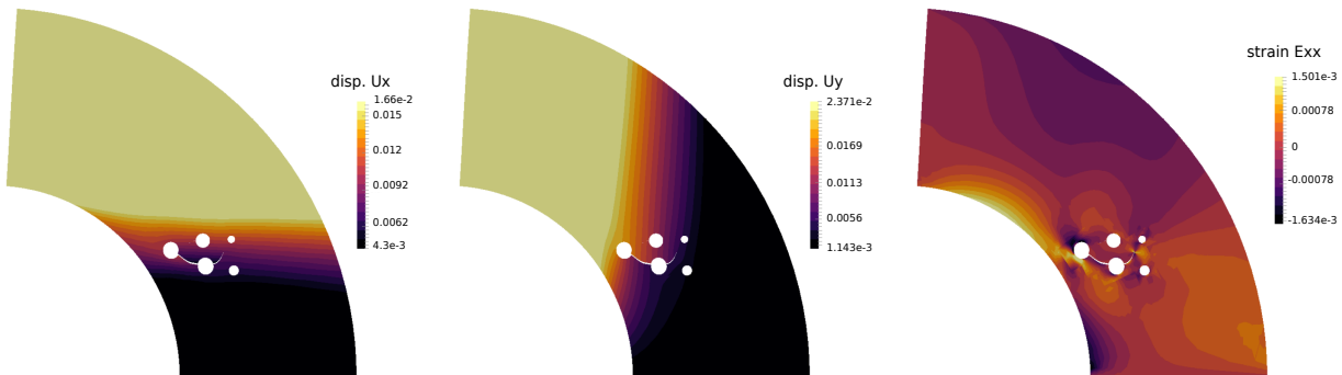
Figure 2.11 – Converged solution obtained with the hybrid IGA/FEM version of algorithm (2.20)-(2.21): (left) horizontal displacement; (middle) vertical displacement; (right) strain component \varepsilon_{xx} .
