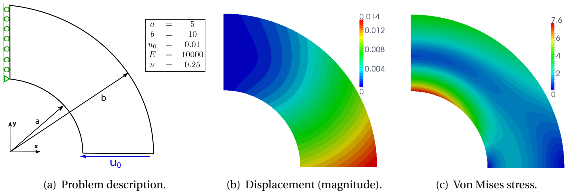
Figure 1.9 – Isogeometric simulation of the curved beam problem (NURBS mesh composed of quadratic C^1 16 \times 24 elements).
