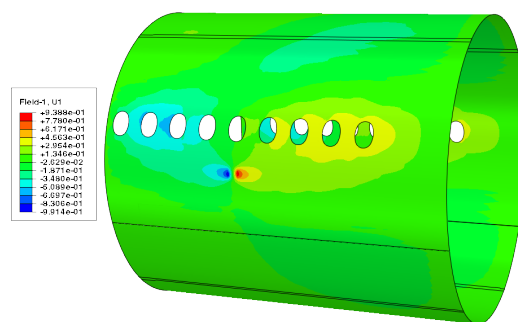
Figure 2.7 – Comparison between the submodeling and the iterative non-invasive approaches: distribution of the difference between the two global horizontal displacements (mm): \mathbf{u}_{\text{non-invasive}} - \mathbf{u}_{\text{submodeling}} ( floor, stiffeners and frames not represented for confidentiality reasons ).
