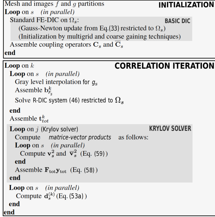
Figure 4.4 – Overview of the proposed DD R-DIC algorithm.
