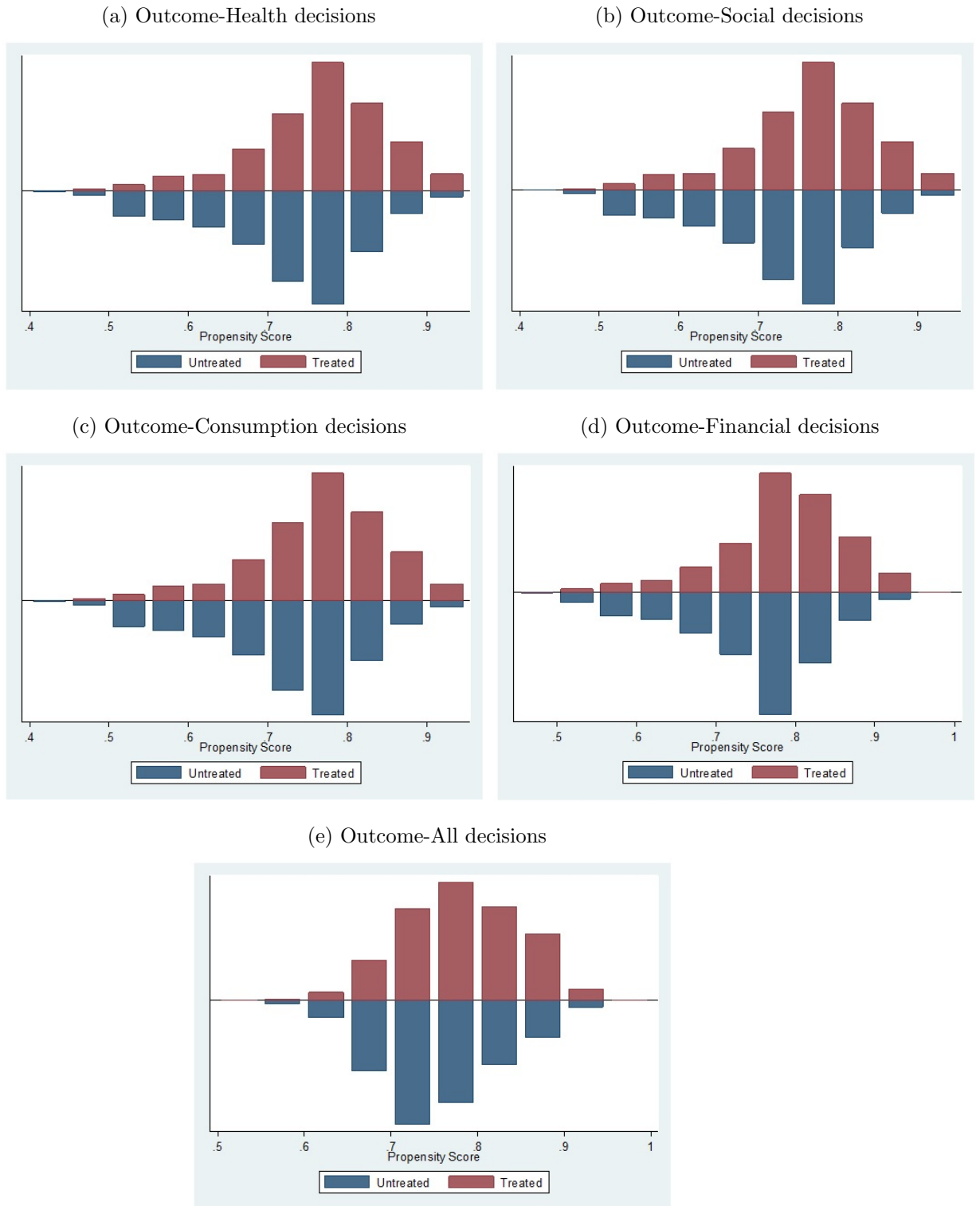
Figure B2: Density distribution for the estimated propensity scores for having no son and having at least one son (Parity \leq 3 )
