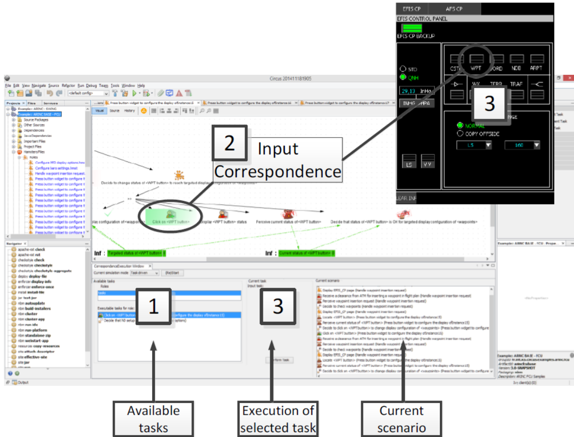
Figure 31. Illustration of a co-execution step between task models and FCU Software application from (Martinie, Navarre, Palanque, & Fayollas, 2015)
