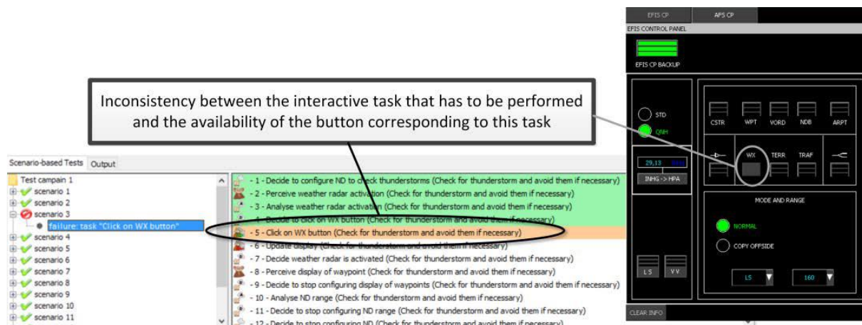
Figure 36. Screenshot of an extract of the result of a test campaign showing a task that could not be executed from (Campos J. C., et al., 2016)
