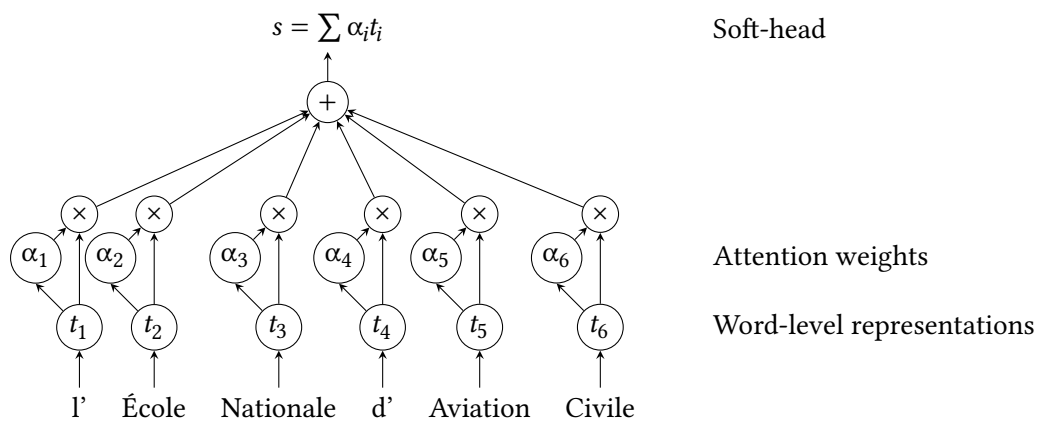
Figure 5.5: Soft-head self-attention in DeCOFre
