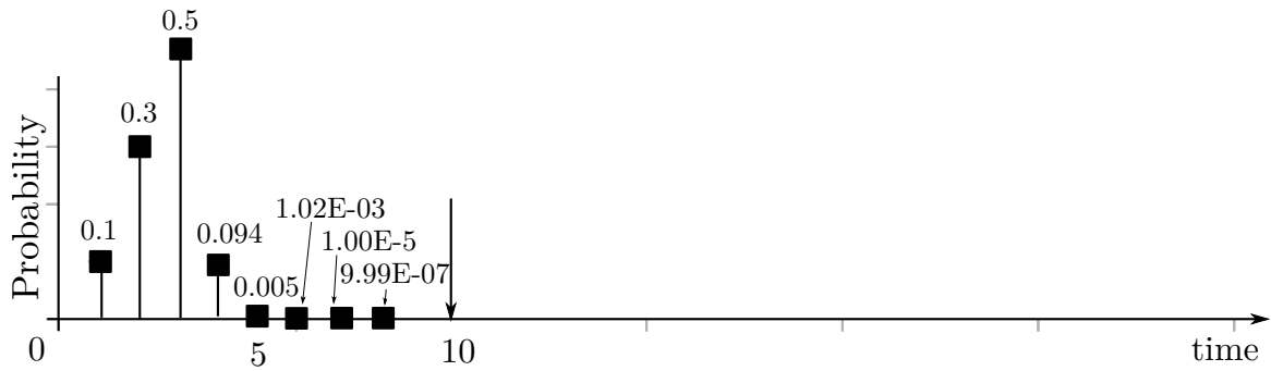
Figure 6.12: Dependent pWCRT PMF of job J_{12} in \Gamma_2 .
