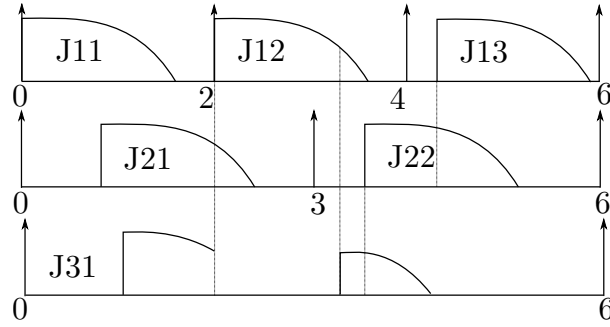
Figure 3.7: EDF scheduling
