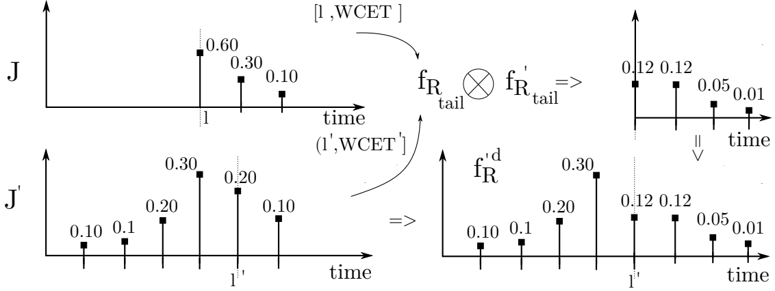
Figure 6.11: Dependence convolution.
