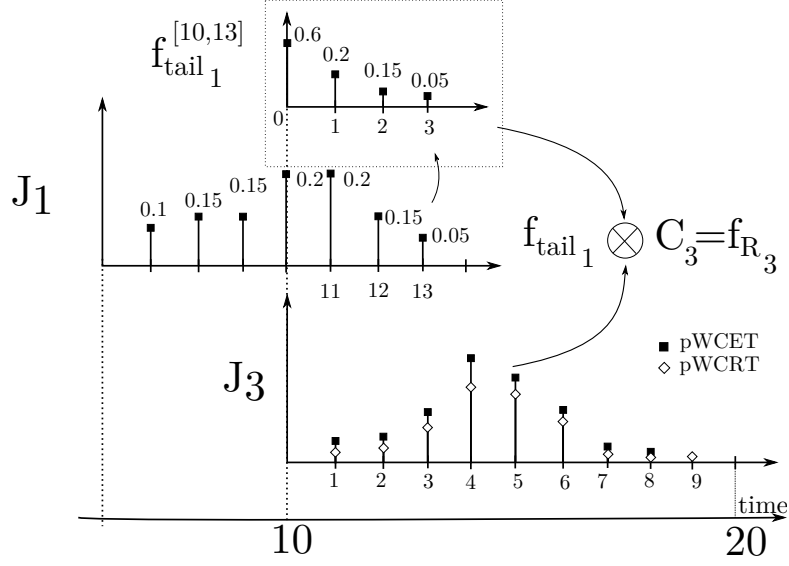
Figure 6.4: pWCRT from convolution of Tail distribution and the pWCET.
