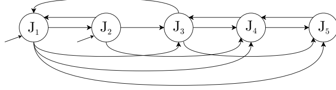
Figure 5.3: Graph for task set \Gamma_1 .
