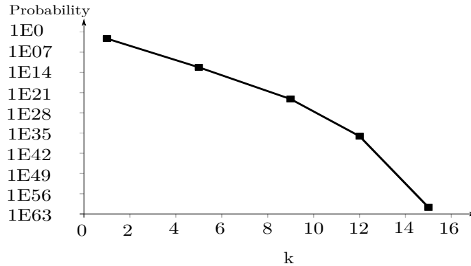
Figure 4.3: P^{kn} from (k, n) system criticality.
