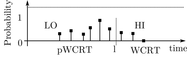
Figure 6.7: pWCRT of a job with threshold for criticality mode.
