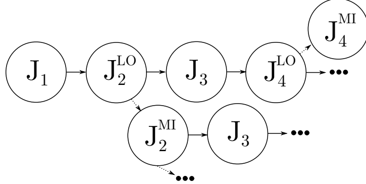
Figure 5.6: A portion of the optimized scheduling tree T_s^{sched} for task set \Gamma_1 with root node J_1 .
