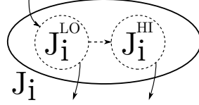
Figure 6.8: HI and LO subnodes within the node for high criticality jobs.
