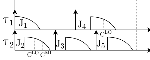
Figure 5.2: Probabilistic job executions of jobs of task set \Gamma_1 in a hyperperiod.
