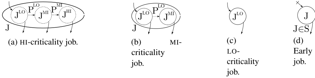
Figure 5.1: Graph nodes for jobs of various criticalities.
