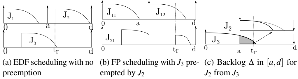
Figure 3.3: Various possible delays to the execution of a job.
