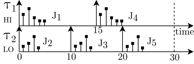
Figure 6.1: Jobs of task set \Gamma_1 .
