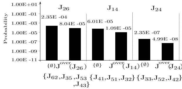
Figure 4.5: Probability of deadline miss of the job J_{14} vs when the LO-criticality jobs dropped.
