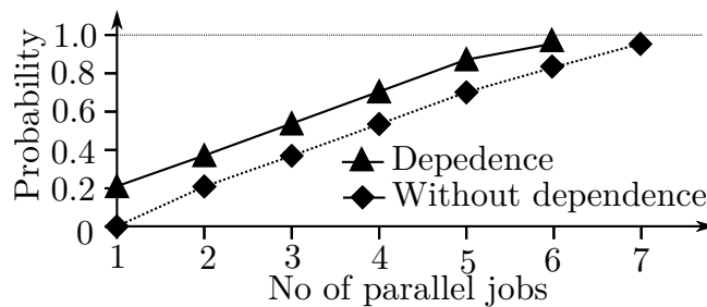
Figure 6.13: Probability of system entering high criticality
