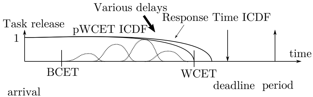
Figure 2.3: Task probabilistic execution shown as a pWCET ICDF with BCET and WCET.
