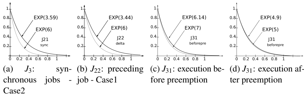
Figure 3.9: Job executions of \Gamma_1 before and after execution interference.
