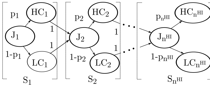
Figure 4.2: System DTMCh model M , assuming J_1, J_2, \dots, J_{n^{\text{HI}}} \in \Gamma^{\text{HI}} and such that p_1 \leq p_2 \leq \dots \leq p_{n^{\text{HI}}} .
