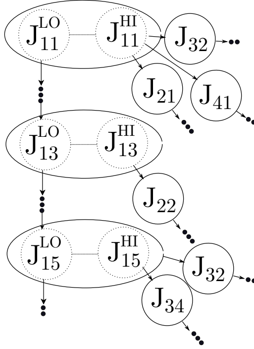
Figure 6.10: Optimal scheduling tree for the task set \Gamma_2 .
