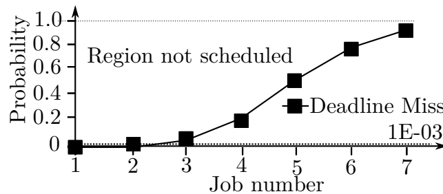
Figure 6.14: Probability of jobs missing deadline
