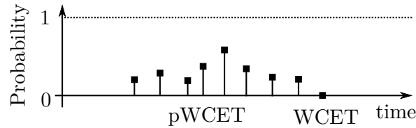
Figure 2.4: pWCET as a PMF distribution.
