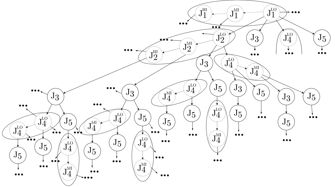
Figure 5.9: A portion of an exploration tree for task set \Gamma_2 with the root node J_1 .
