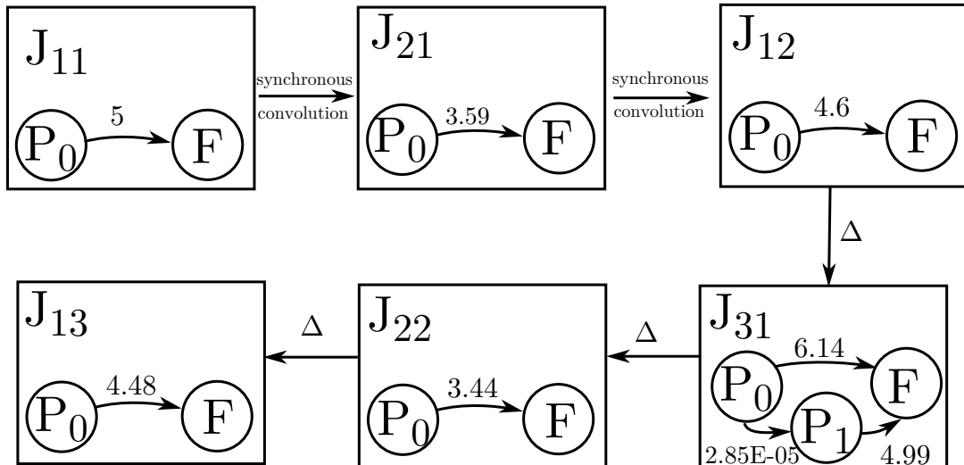
Figure 3.8: CTMCh job models
