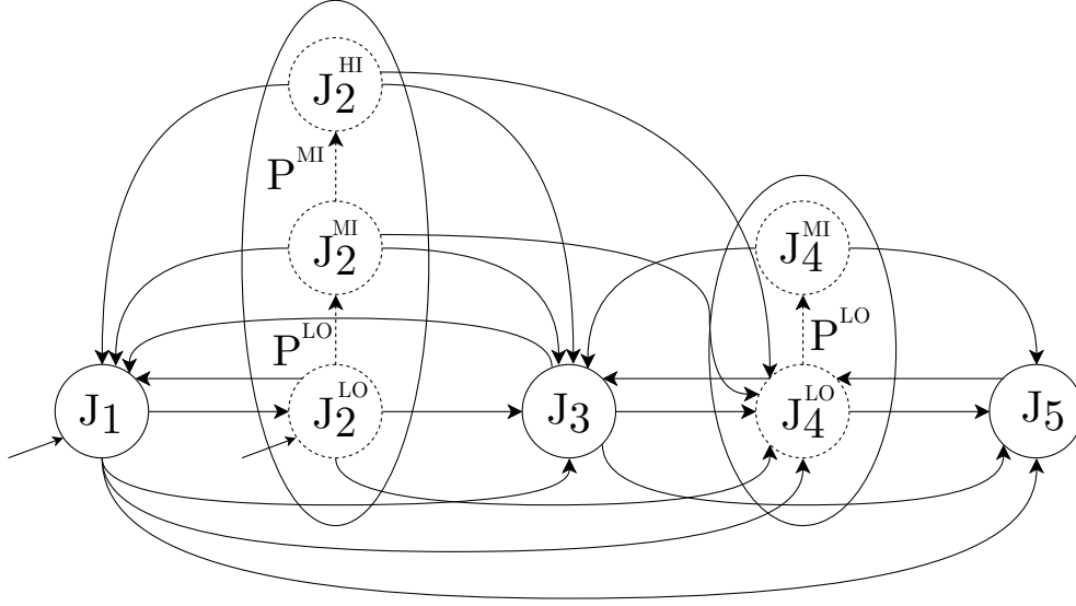
Figure 5.4: Graph with subgraphs for task set \Gamma_1 .
