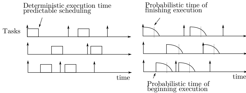
Figure 1.4: Tasks executions with WCET(left) or pWCET(right) .
