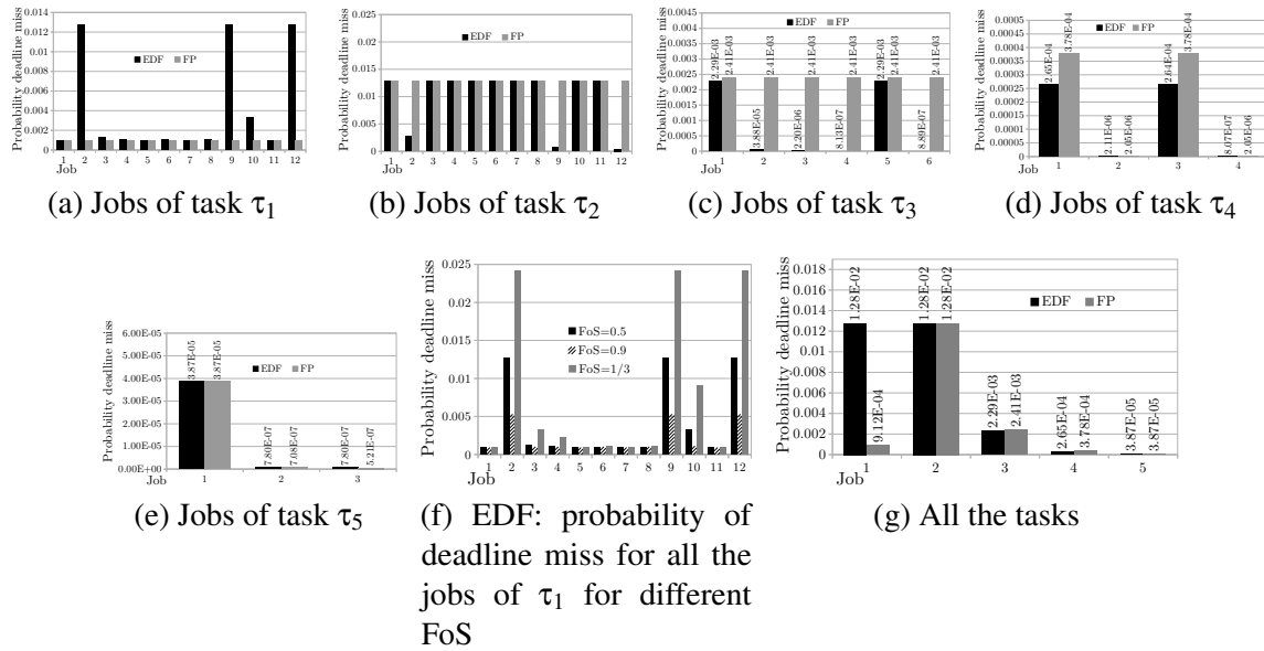
Figure 3.12: Probabilities of deadline misses for the jobs given by the task set \Gamma_4 .
