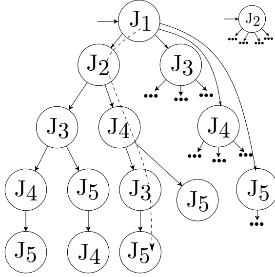
Figure 6.3: Graph unfolded into a tree for jobs of \Gamma_1 .
