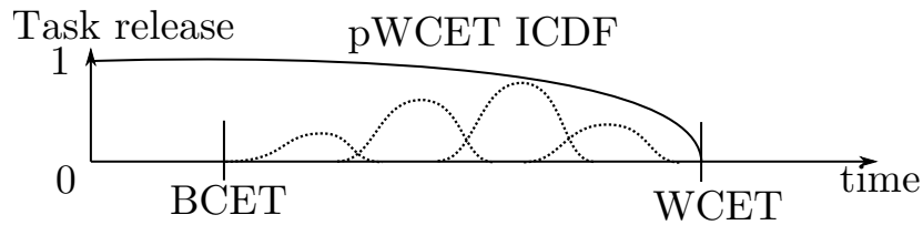
Figure 1.3: Task probabilistic execution through pWCET represented as ICDF with BCET and WCET.
