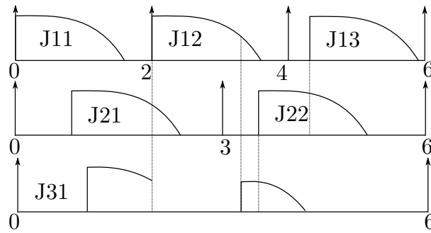
Figure 3.7: EDF scheduling
