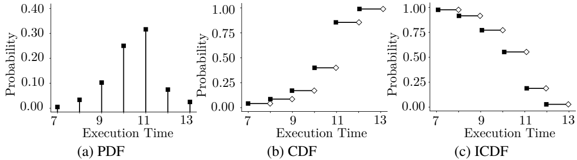
Figure 2.2: Example of PDF, discrete CDF and discrete CCDF representations of a certain distribution.
