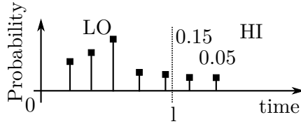
Figure 6.5: High criticality from a threshold l_1 on pWCRT of a job J_1 of \Gamma_1 .
