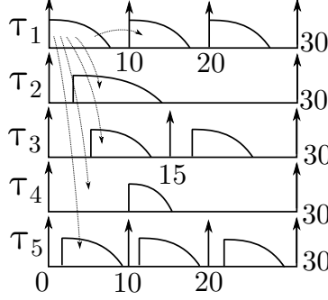
Figure 5.7: Jobs in \Gamma_2 .
