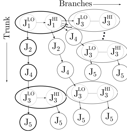
Figure 6.9: The scheduling tree T_{sched} for the schedule in P_{MC} .
