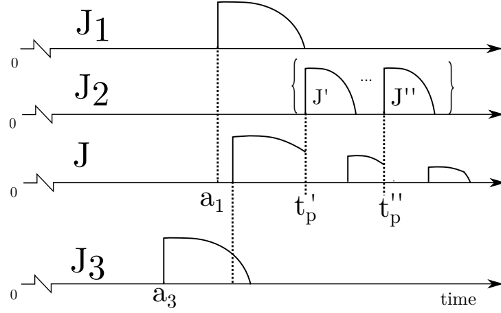
Figure 3.4: Job J , job set J^{prd}(J) , job set J^{sync}(J) , and job set J^{prm}(J) are represented with interactions between them.
