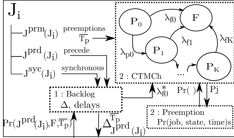
Figure 3.5: Job CMTCh model formalization with blocks and input information.
