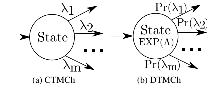
Figure 3.1: CTMCh and the corresponding embedded DTMCh.
