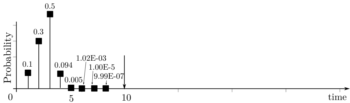
Figure 6.12: Dependent pWCRT PMF of job J_{12} in \Gamma_2 .
