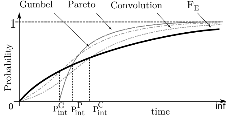
Figure 3.2: Exponential EXP upper bounding distributions with a certain rate.
