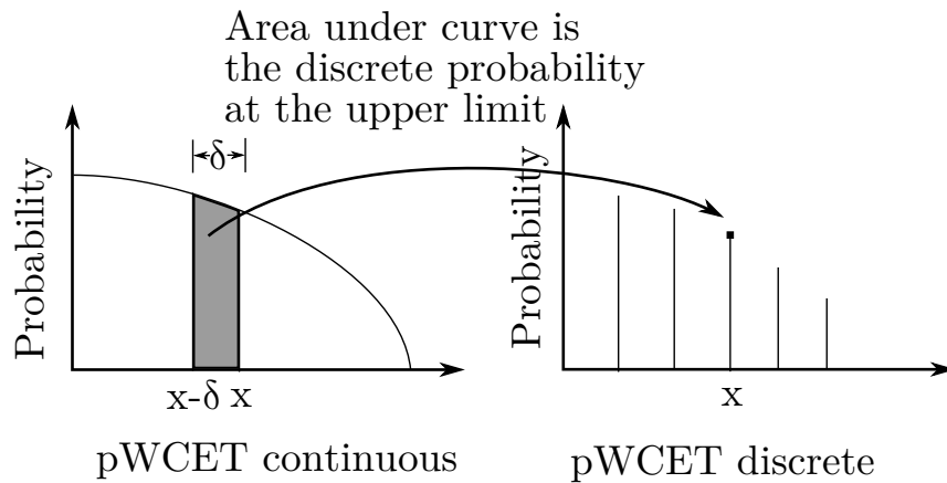
Figure 3.13: Continuous to Discrete pWCET
