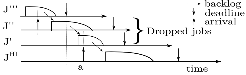
Figure 4.4: The backlog to the HI-criticality job J^{\text{HI}} reduces to zero by dropping LO-criticality jobs J' and J'' .
