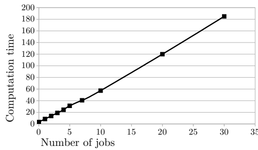
(c) Computation time for the interference from preempting jobs
