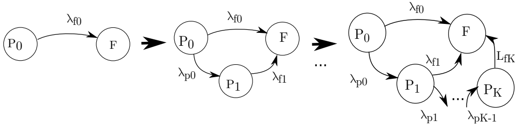
Figure 3.6: Iterative process to build a CTMCh model; the preemption effects are added and validated one preemption by one preemption.
