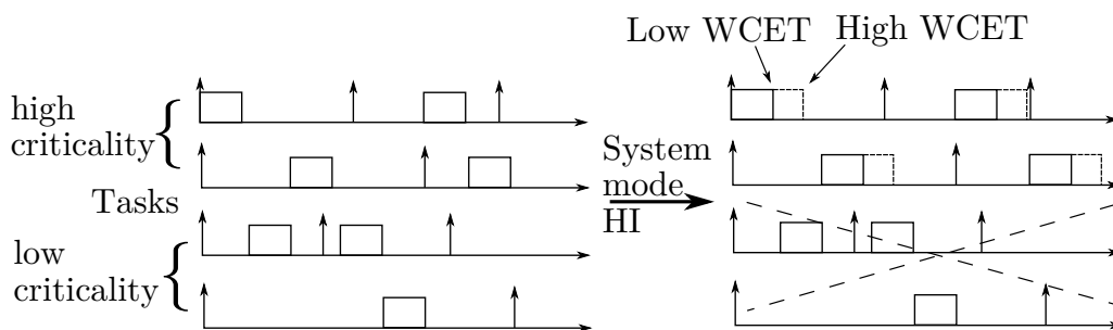
Figure 1.5: Mixed Criticality scheduling.
