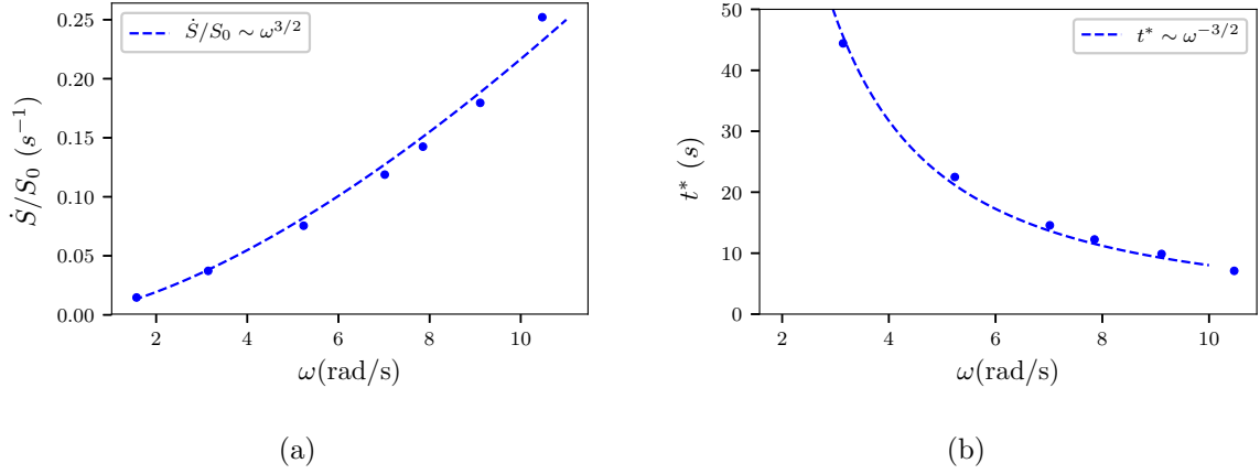
Figure 4.10 – a) Rate of increase of specific surface (dashed lines in Fig. 4.9(b)); b) Characteristic time t^* as a function of rotation speed \omega .
