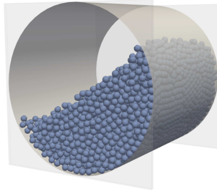
Figure B.1 – Illustration of a rotating drum with two plans closing the end walls of the cylinder.
