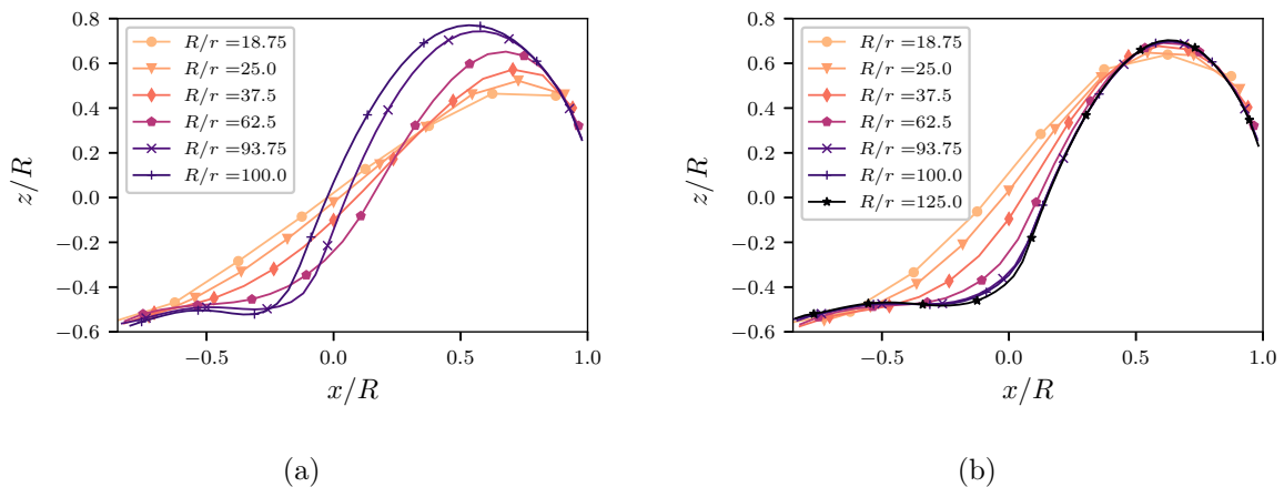
Figure 3.11 – Free surface profile for drums of different sizes at (a) \omega constant and (b) Fr constant. The position x and z are normalized by the drum radius R .
