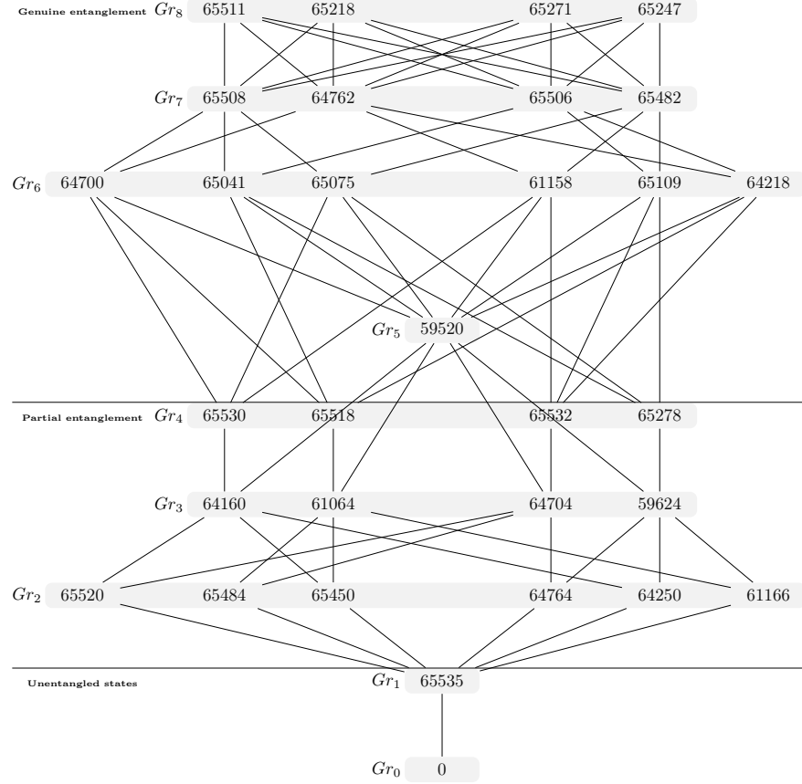
Figure 6: Varieties of the null-cone .
