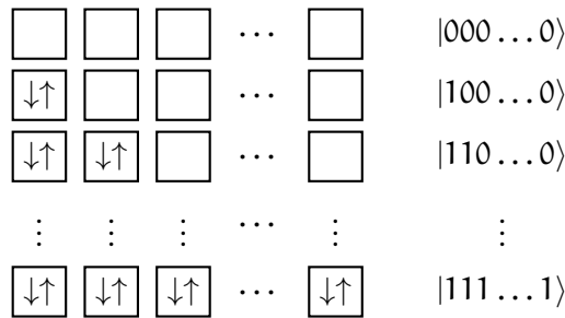
Figure 11: Double occupancy embedding of the n -qubit Hilbert space ( 2^n basis vectors) inside \mathcal{F}_+ ( n boxes and N = 2n single particle states).
