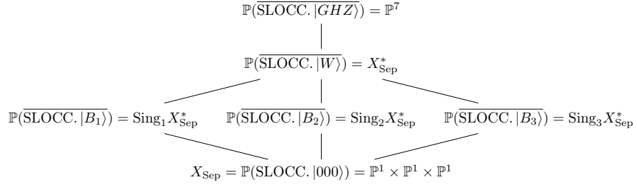
Figure 7: Stratification of the (projectivized) Hilbert space of three-qubit by SLOCC-invariant algebraic varieties (the dual and its singular locus): \text{Sing}_i X_{\text{Sep}}^* represent different components of the singular locus [89, 122] (to be compared with Figure 3).
