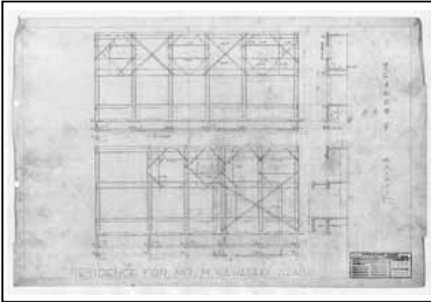
Steel bars (1:20)
