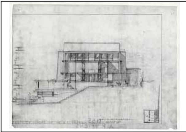
East elevation (1:50)
