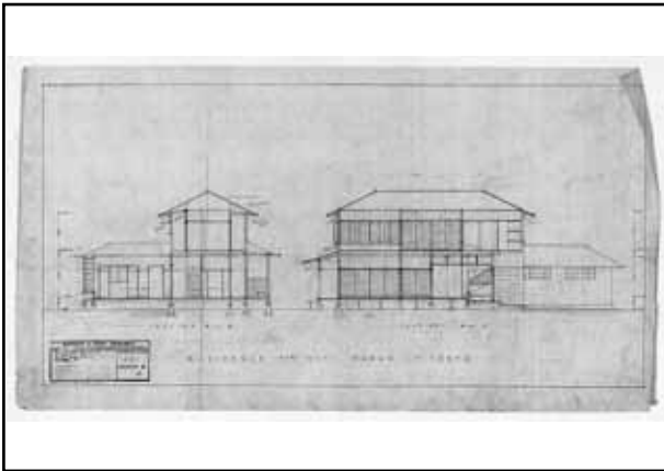
Sections: cross and longitudinal (1:50)
