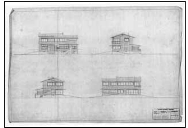
Elevations: north, east, west, south (1:100)
