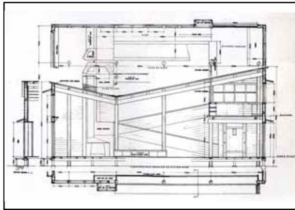
Living room section and ramp plan
