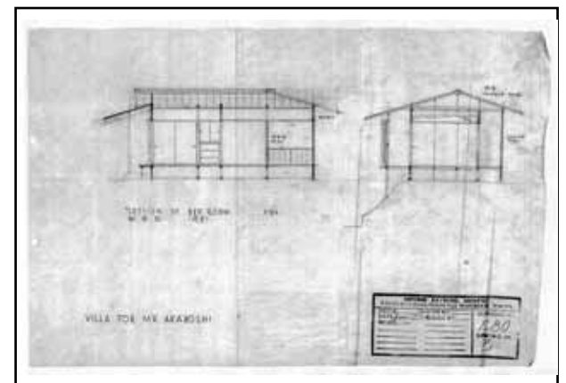
Section: bedroom
