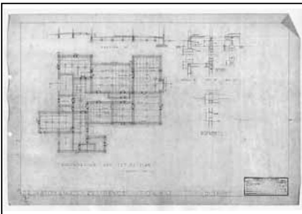
Floor plan: foundation and 1F (1:50)
