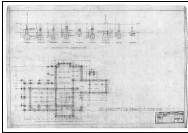
Foundation plan and details (1:50; 1:20)
