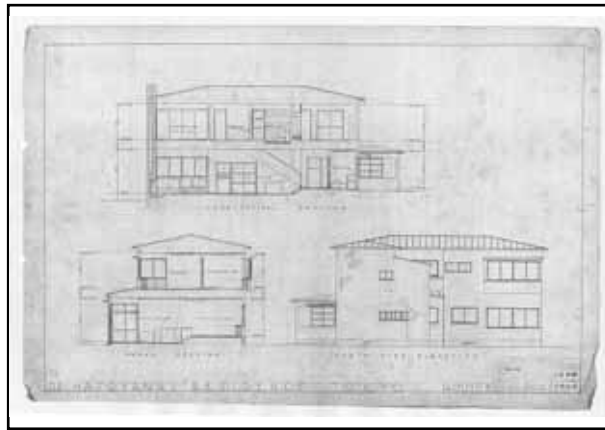
Sections: longitudinal and cross; Elevation: north (1:50)
