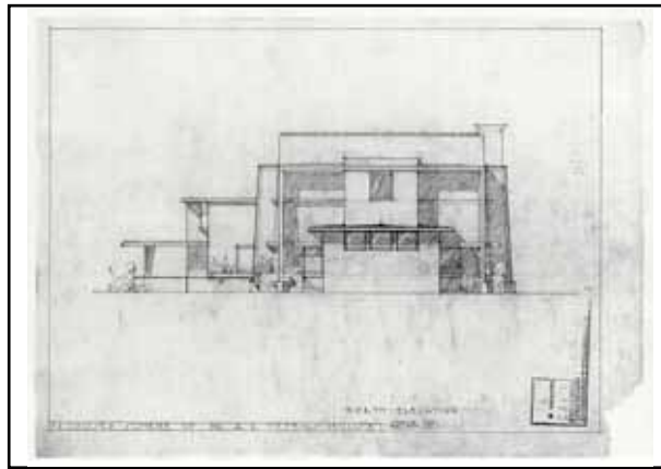
North elevation (1:50)
