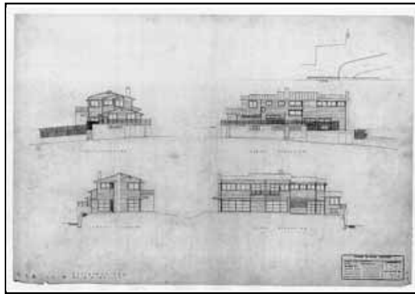
Elevations: east, north, west and south (1:100)
