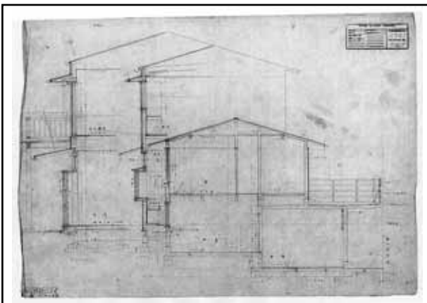
Cross section 2 (1:20)
