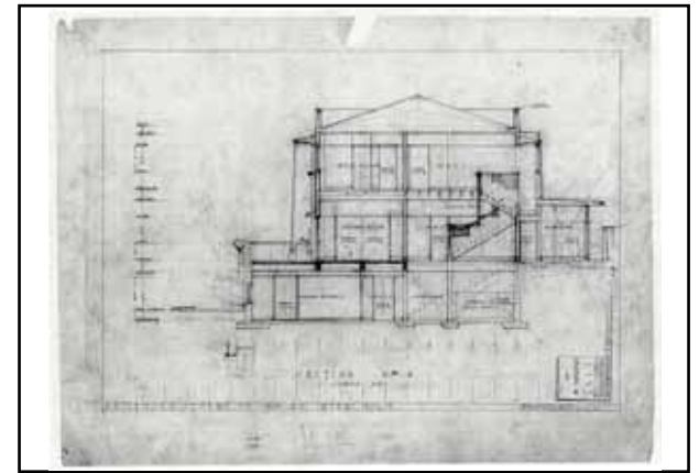
Cross section (1:50)
