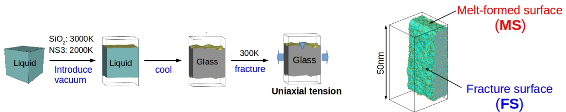
Figure 4.1: Schematics of the simulation procedure. Glass with free surfaces, i.e. melt-formed surface (MS) is fractured under uniaxial tension, resulting in fracture surfaces (FS).
