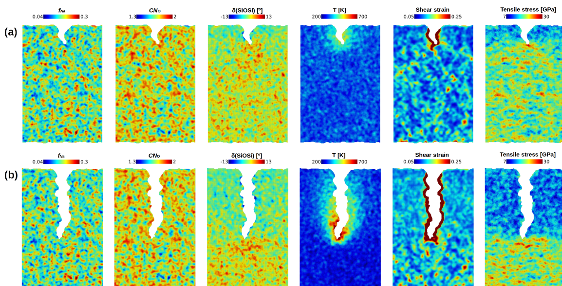
Figure 3.20: Maps of various local properties at (a) \epsilon = 0.172 and (b) \epsilon = 0.192 for the NS3 sandwich glass. See the text for the definition of each quantity. These maps are shown for the middle plane of the simulation box in the direction orthogonal to the crack front.
