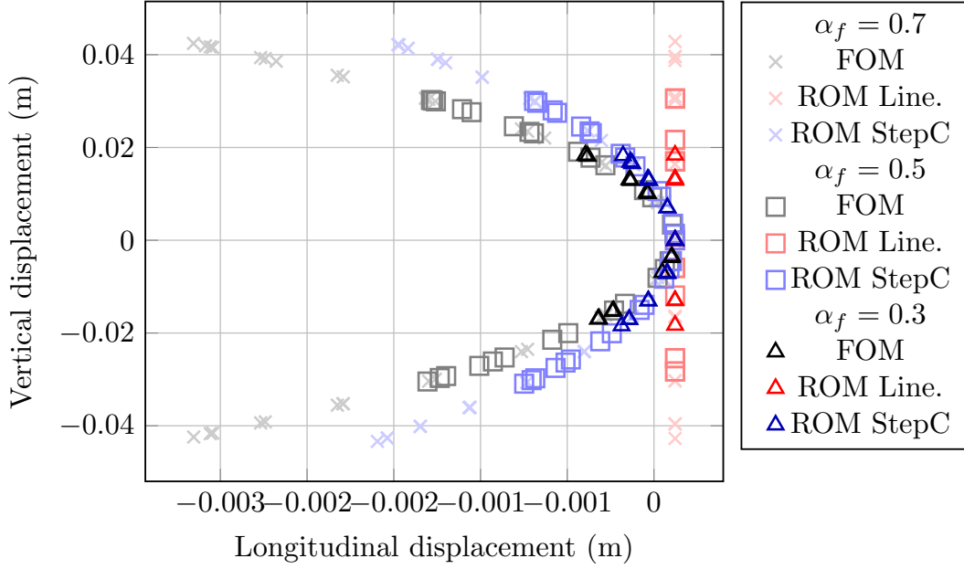
Figure 3.12: Longitudinal and/vs. vertical displacements of the tip of the beam for a rotating velocity \Omega = 4000 rpm.
