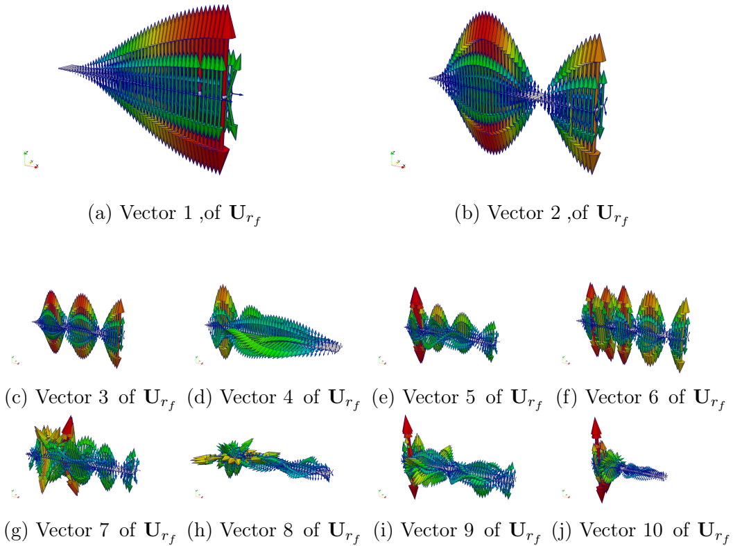
Figure 3.18: Fist 10 vectors of \mathbf{U}_{r_f} obtained with an incremental static loading at \Omega = 0 rpm.
