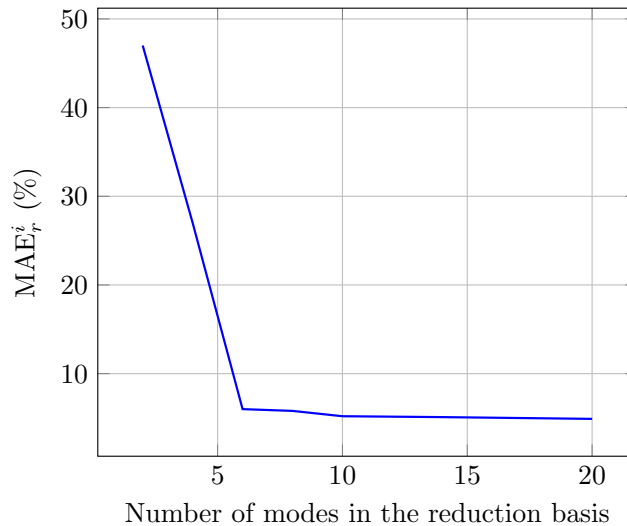
Figure 3.21: Maximum MAE_r^i of the StepC ROM with respect to the number of optimal LNM that form the reduced basis for the \alpha_{f4} loading intensity.
