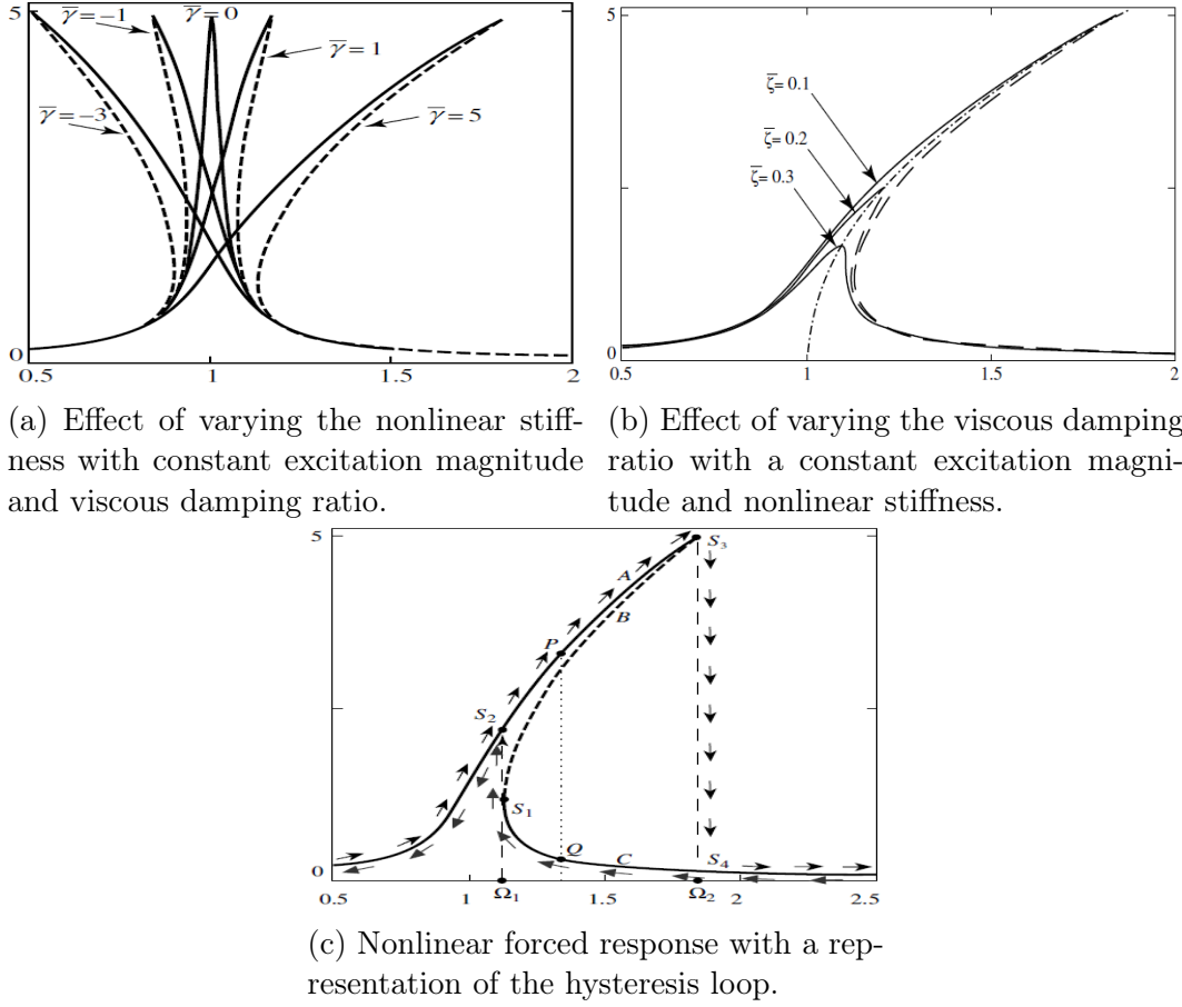
Figure 2.2: Geometrically nonlinear effect on the forced response of the structure [Kalmár-Nagy and Balachandran, 2011].
