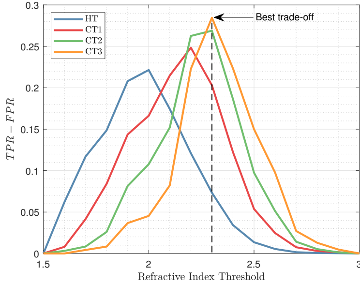
Figure III.31: TPR – FPR as a function of the refractive index threshold for HT, CT1, CT2 and CT3, at 560 GHz.
