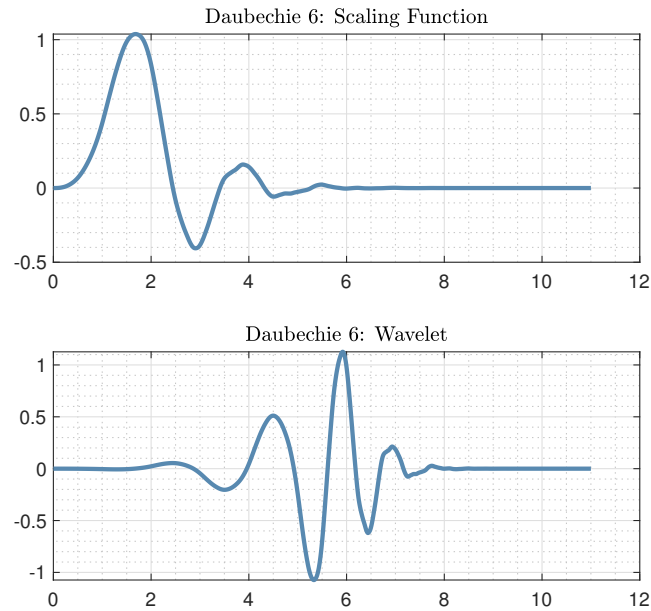
Figure III.9: Scaling function and shape of the db6 wavelet.
