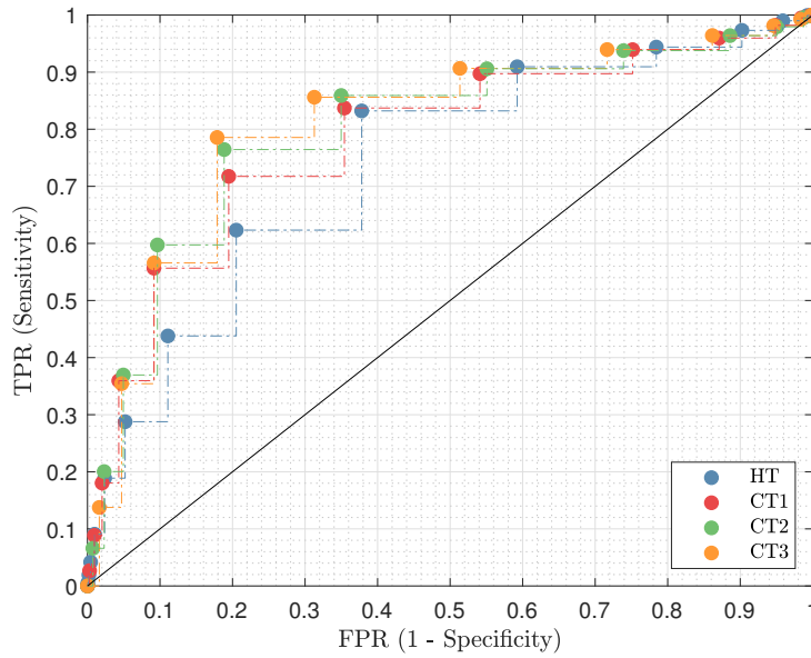
Figure III.26: Receiver operating characteristic for the different classification methods, at 560 GHz. The black line represents TPR = FPR.
