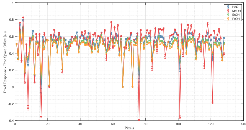
Figure IV.26: Pixel response to water (blue), methanol (red), ethanol (green) and propanol (yellow). The mean level of propanol is slightly lower than that of ethanol. The mean level of the matrix response to methanol is higher than for other liquids. Water stands in the middle as a result of the impact of its lossy part of permittivity.
