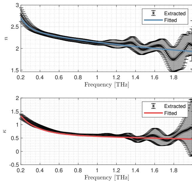
Figure II.27: Fit to 2-Debye terms model and the experimental n(\omega) and \kappa(\omega) .
