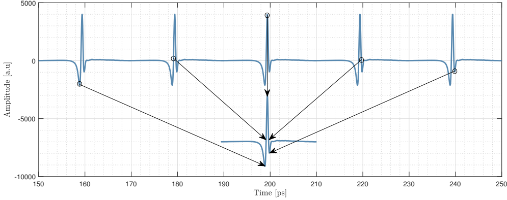
Figure II.3: Reconstruction of a terahertz pulse by means of electro-optic sampling method.
