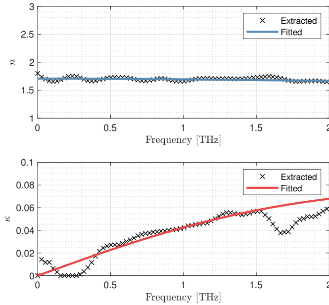
Figure II.20: 1st order Debye ( i.e. n = 1 equation I.22.) fit of the IEP extracted properties.
