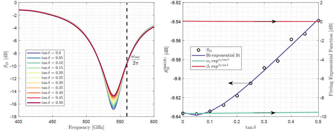
Figure IV.15: Profile of S_{21} as a function of different \epsilon'' . Left: Highlight of LC-circuit response due to the progressive increase of \epsilon'' . Right: Bi-exponential behavior of S_{21} as a function of the \tan \delta relative loss angle at 560 GHz, with \alpha_1 = -9.677 , \alpha_2 = -0.029 , \beta_1 = 0.041 and \beta_2 = -10.55 .
