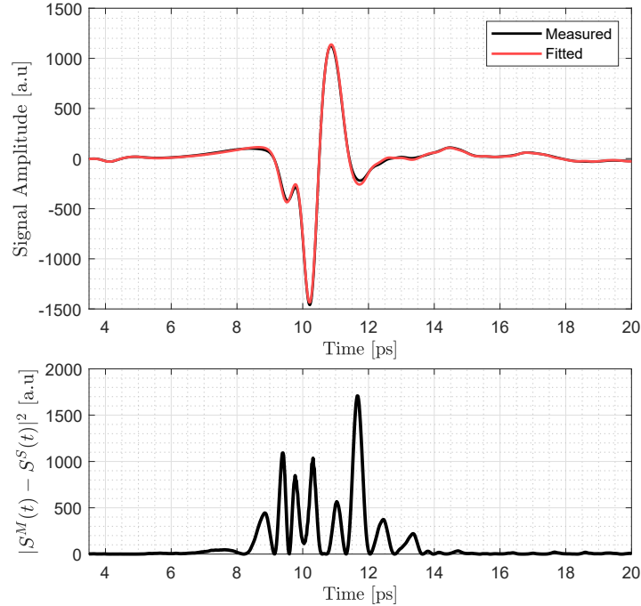
Figure II.21: Reconstructed waveform after fitting the optical properties.
