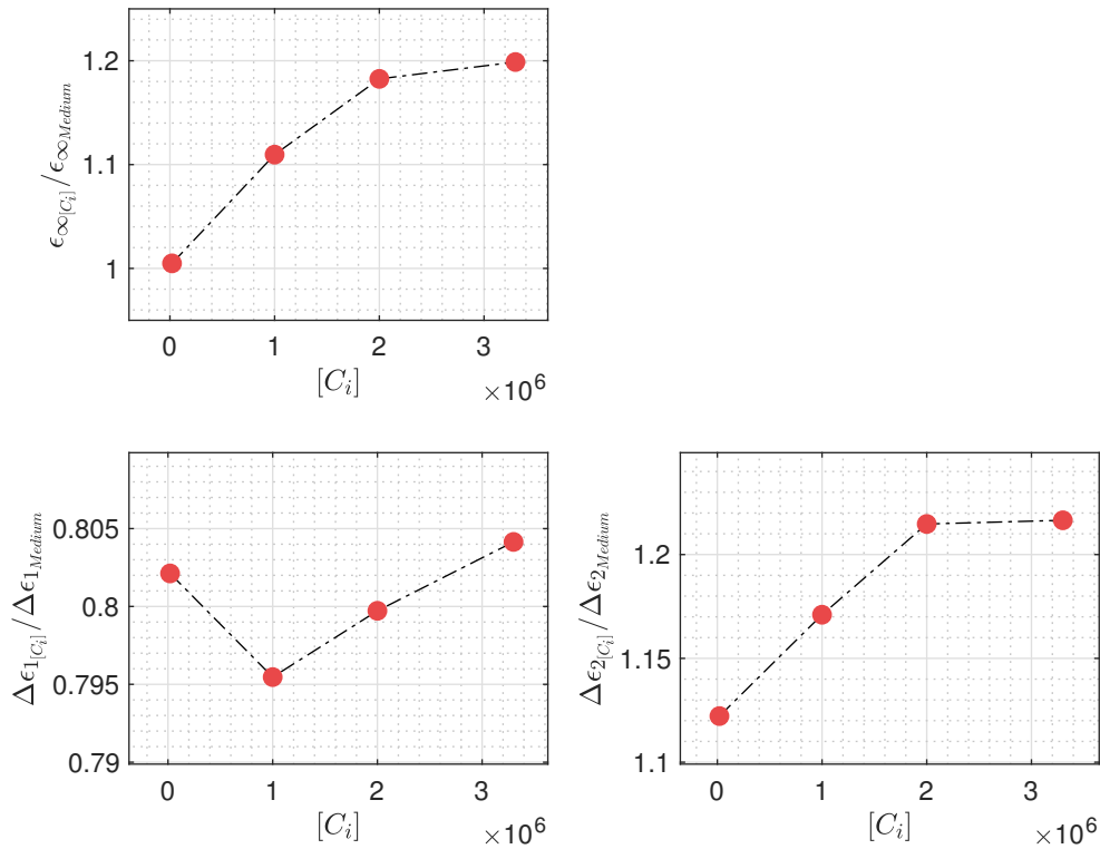
Figure II.40: Variations in \epsilon_{\infty} , \Delta \epsilon_1 and \Delta \epsilon_2 as a function of MCF7 cell concentration.
