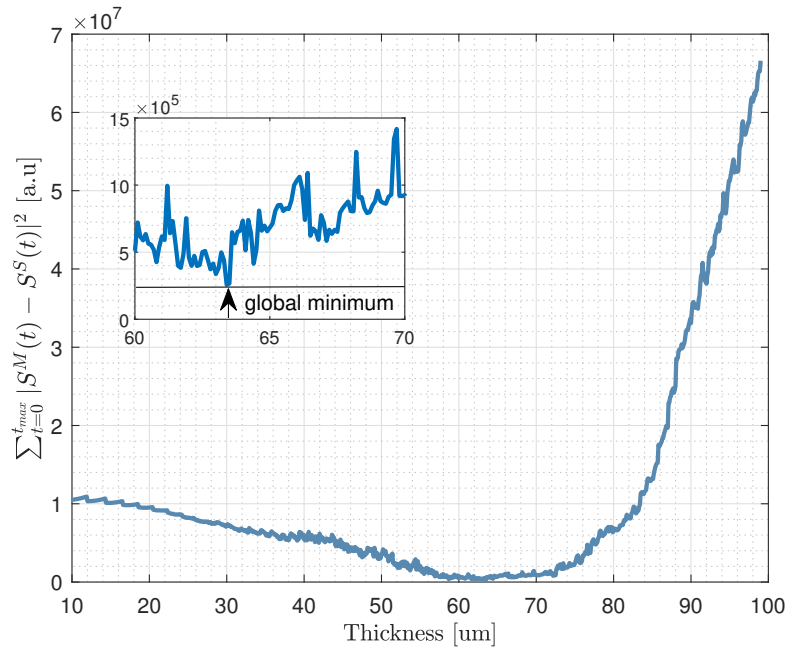
Figure II.17: \sum_{t=0}^{t_{max}} |S^M(t) - S^S(t)|^2 as a function of the tested thicknesses contained in the d vector. The global minimum was found to be 63.4 \mu m .
