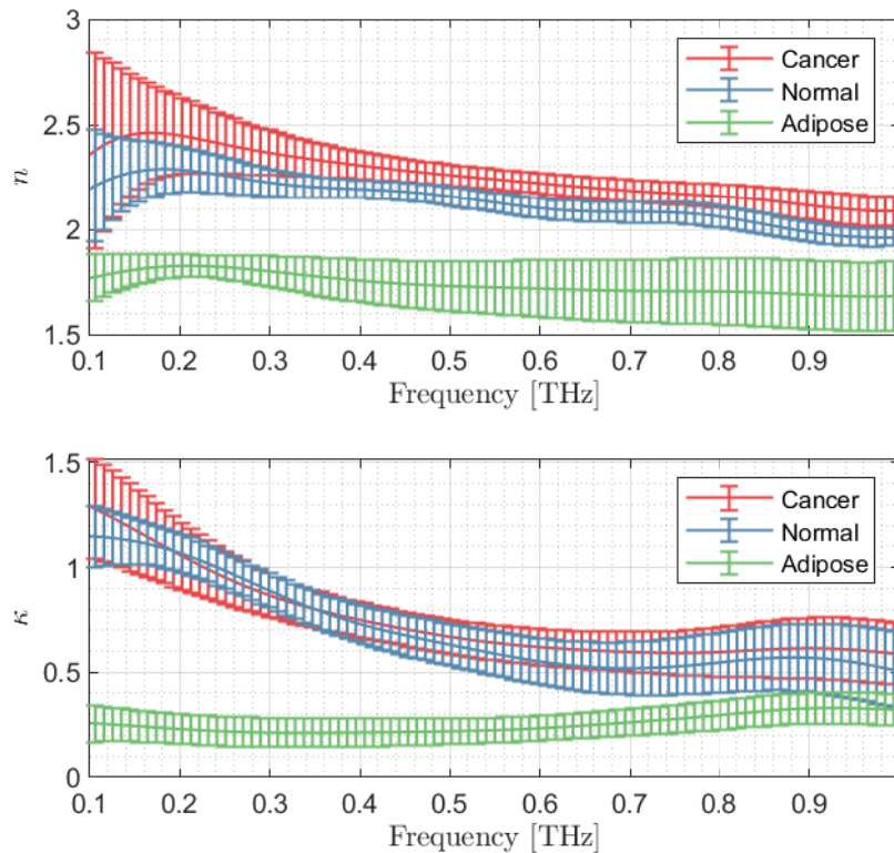
Figure II.33: Refractive index and extinction coefficient for malignant lesions, healthy fibrous and adipose tissues.
