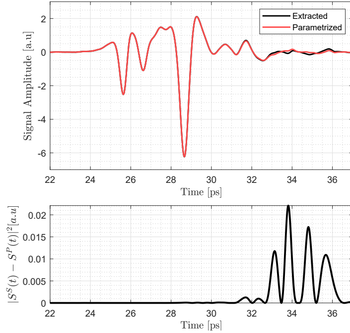
Figure II.15: Top: Reconstruction of the signal provided by the reduced iterative tree algorithm (black cross) with the 33 selected contributing paths (red). The correlation is almost perfect between the two signals over the entire time window. Bottom: \Lambda(t) metric. Differences are observed in regions where additional subdivided pulses have been ommitted (e.g. k > 17 ).
