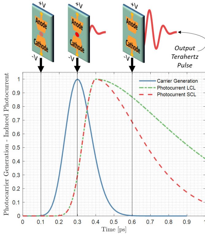
Figure II.1: Illustrative example of pulsed terahertz generation by means of a photoconductive antenna. LCL: long carrier lifetime. SCL: short carrier lifetime.
