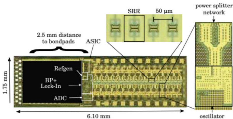
Figure IV.20: Micrograph of the near-field sensing array. The sensing strip length is 3.2 mm long. The black region contains additional circuits that are not associated to the near-field sensing. ASIC: application-specified integrated circuits. ADC: analog-to-digital converted. Refgen: reference generator. BP: bandpass.
