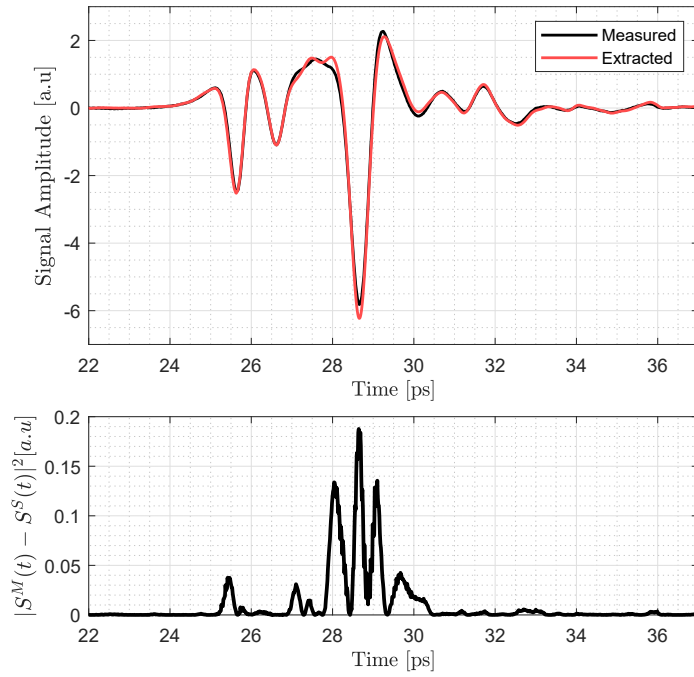
Figure II.12: Top: experimental signal of the stratified structure in reflection geometry (black) and its reconstruction via the iterative tree algorithm (red). Bottom: deviations observed from the measured signal using the \Lambda(t) metric.
