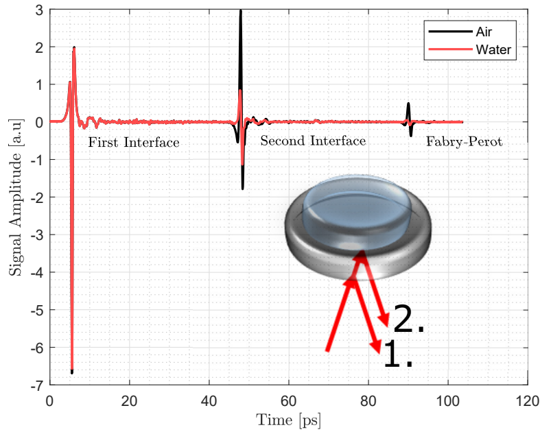
Figure II.23: Typical time-domain waveform recorded without (black) and with (red) water film on the top side on the sapphire substrate.
