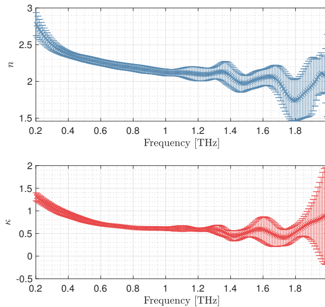
Figure II.24: Water optical properties extracted in reflection geometry, averaged over ten independent measurements.
