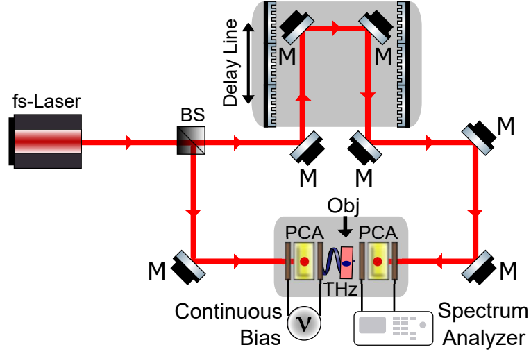
Figure II.4: Schematic details of a time-domain system for terahertz spectroscopy in transmission configuration. BS stands for beam splitter, and M depicts mirrors.
