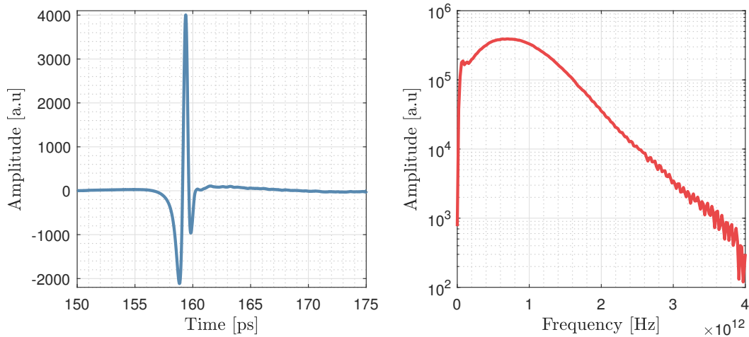
Figure II.6: Illustrative terahertz time-domain waveform (blue) and spectrum (red) recorded through the use of a TDS setup.
