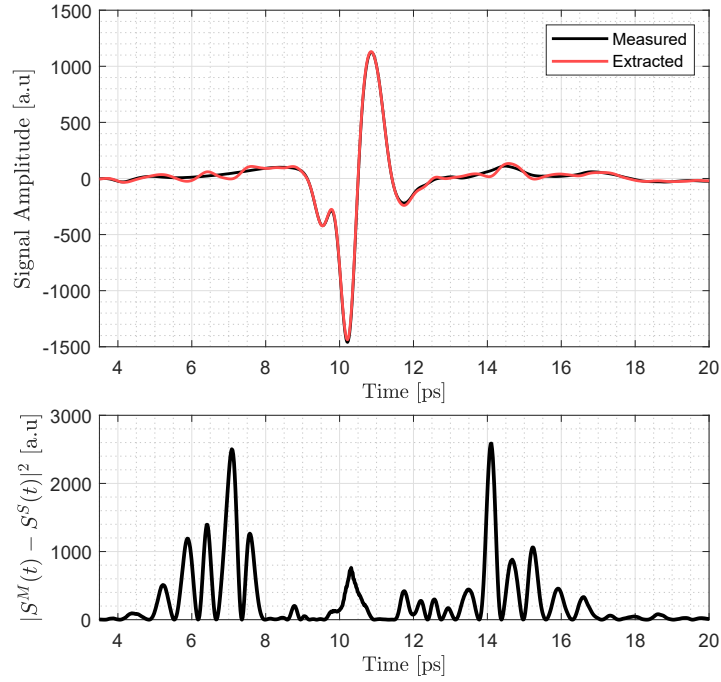
Figure II.18: Time-domain error of the thickness global minimum using the \Lambda metric.
