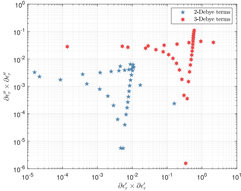
Figure II.26: Residuals at each \omega with respect to both the real and complex plane for 2-Debye terms and 3-Debye terms.
