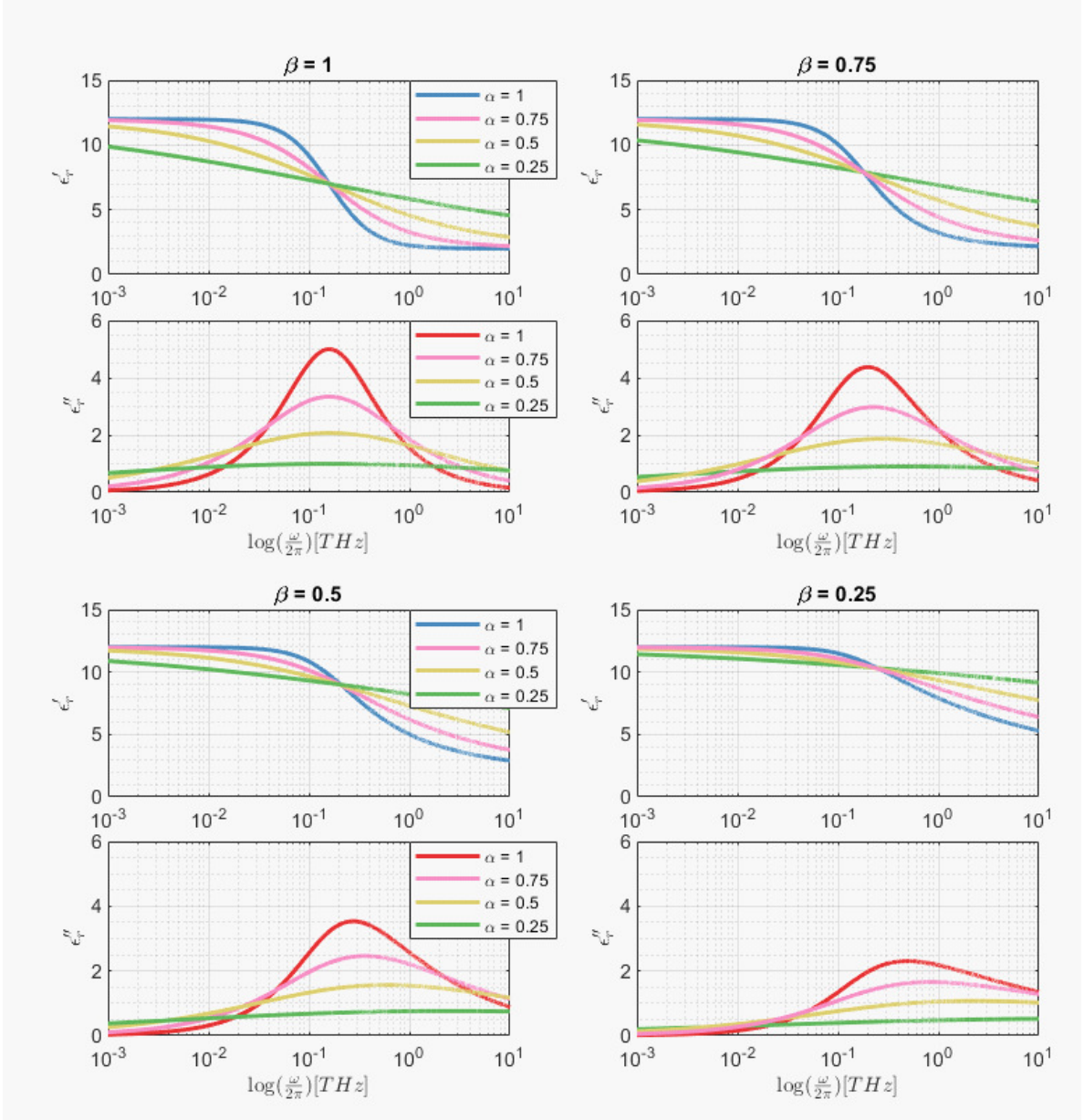
Figure I.7: Illustration of the Havriliak-Negami formulation for the Debye parameters used in Figure I.4 and for \alpha and \beta taking the successive values: 0.25, 0.50, 0.75.
