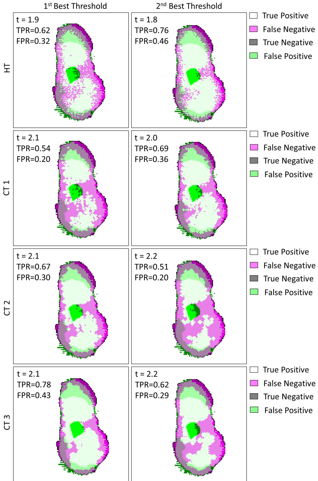
Figure III.24: NS1 tissue sample classification map at 560 GHz for HT, CT1, CT2 and CT3 and their respective first two best thresholds, at 560 GHz.
