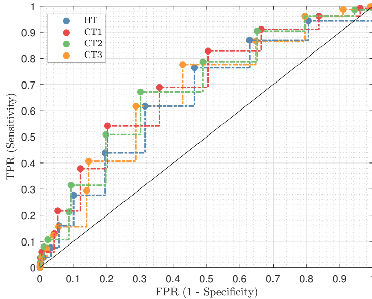
Figure III.22: Receiver operating characteristic for the different classification methods, at 560 GHz. The black line represents TPR = FPR .
