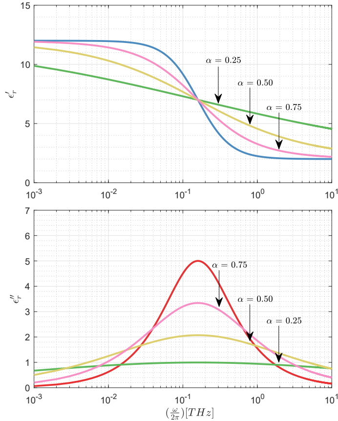
Figure I.5: Illustration of the Cole-Cole treatment for the Debye parameters used in Figure I.4 (Top: blue; Bottom: red) and for \alpha = 0.25, 0.50, 0.75 subsequently.
