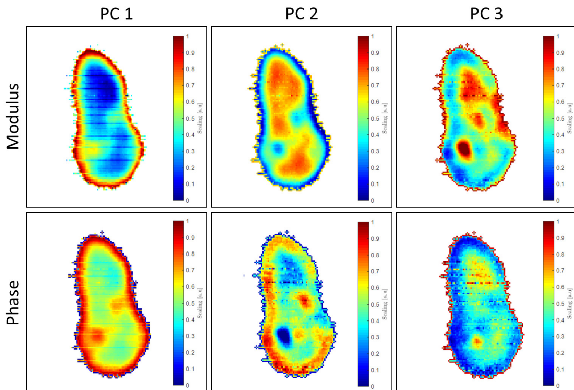
Figure III.35: Integrated loading weighted frequencies for modulus and phase data set for the first three principal components. The reader is referred to Figure III.21 for eyeball comparison.
