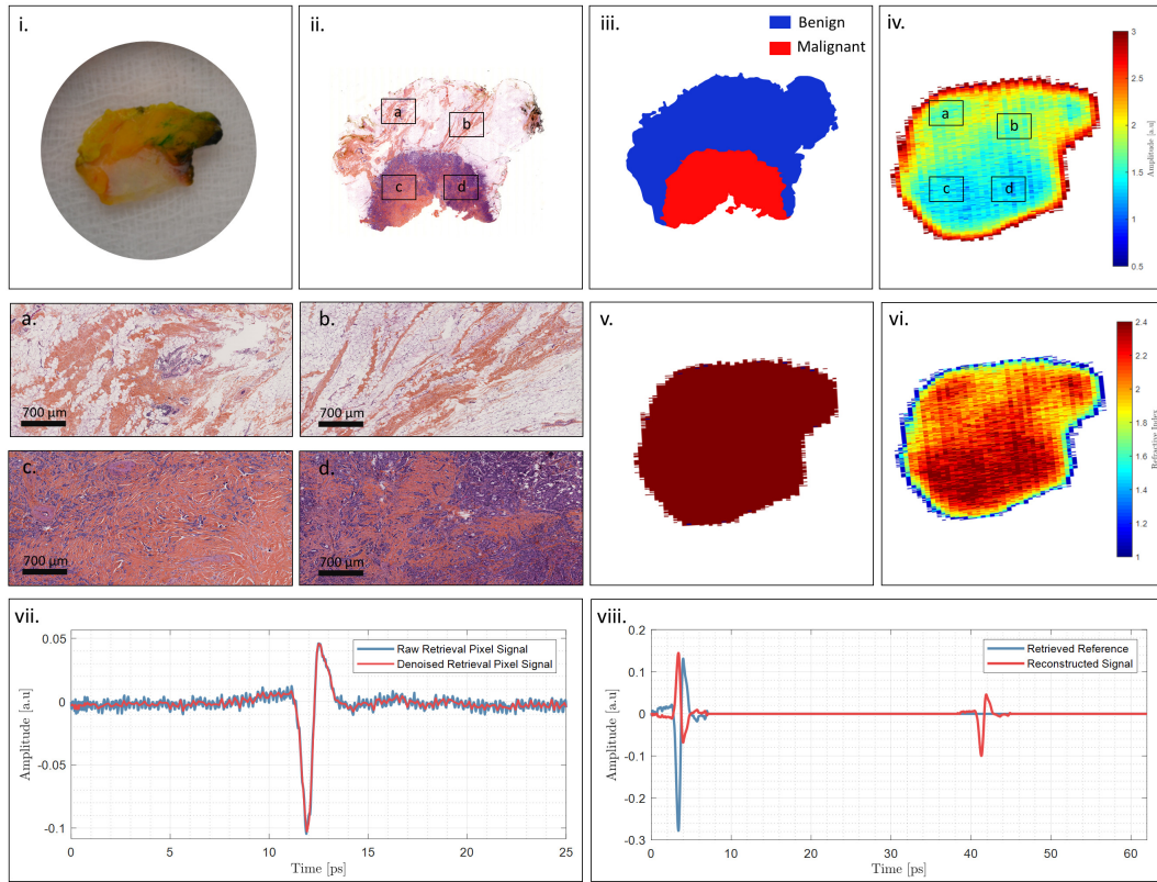
Figure III.25: Overview of the results obtained via the procedure for the NS2 sample: i. photograph; ii. pathology image with four enlightened regions. A gap is shown in the middle of the section that is due to the histology chain; iii. Pathology mask derived from the pathologist diagnosis. iv. Terahertz image of the tissue sample at 560 GHz; v. Terahertz mask derived from the 560 GHz raw image; vi. Refractive index map calculated from the self-reference procedure and the inverse electromagnetic problem; vii. Raw and denoised retrieval pixel signals used to retrieve the reference signal - relative time-scale; viii. Reconstructed signal from the retrieval denoised pixel signal - relative time-scale. a, b, c and d are pathological view of the regions related in the pathology image (ii) and the raw terahertz image (iv).
