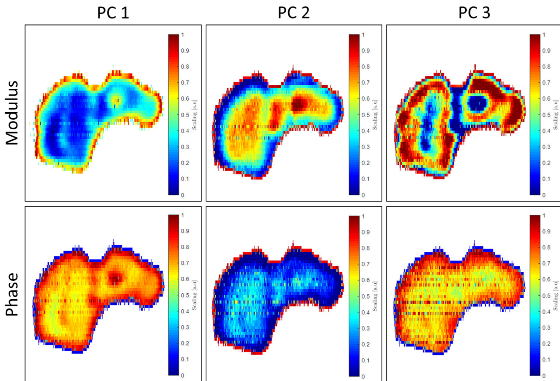
Figure III.41: Integrated loading weighted frequencies for modulus and phase data set for the first three principal components. The reader is referred to Figure III.29 for eyeball comparison.
