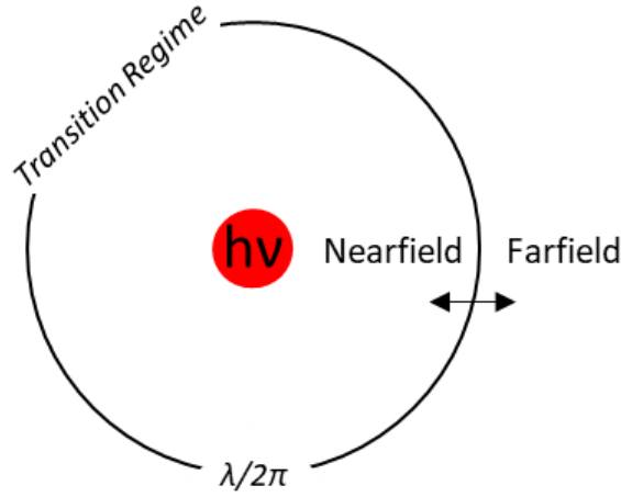
Figure IV.1: Delineation between the near-field domain and the far-field regime. The near-field regime is defined as the sphere of radius \lambda/2\pi whose center is the punctual electromagnetic source. Beyond the near-field sphere, interactions with matter should be regarded as far-field effects.
