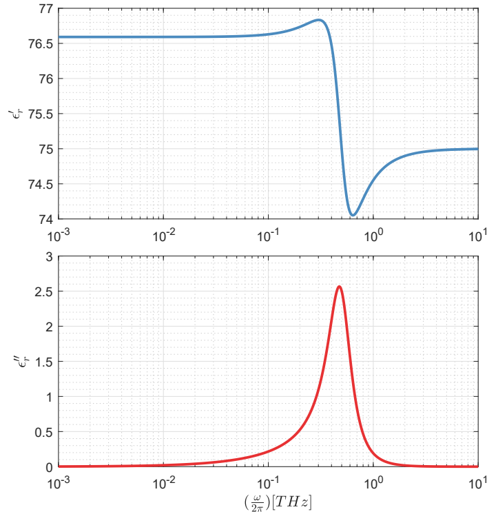
Figure I.8: Illustration of a Lorentz oscillator for \epsilon_0 = 75 , A/(2\pi)^2 = 0.25 \text{ THz}^2 , \Gamma/(2\pi) = 0.32 \text{ THz} and a characteristic frequency at \omega_0/(2\pi) = 500 \text{ GHz} .
