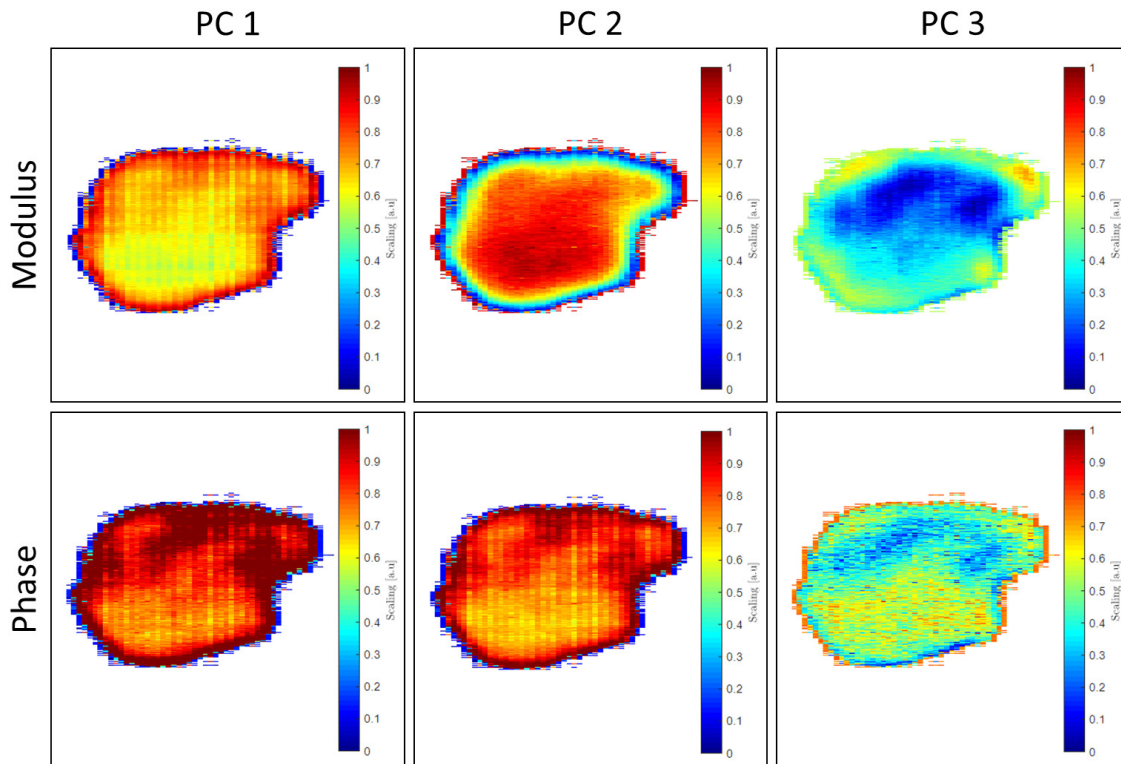
Figure III.38: Integrated loading weighted frequencies for modulus and phase data set for the first three principal components. The reader is referred to Figure III.25 for eyeball comparison.
