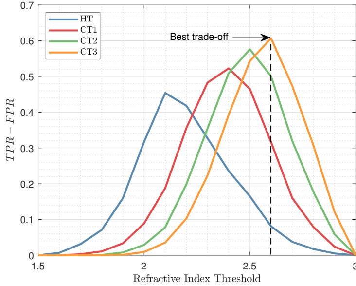
Figure III.27: TPR – FPR as a function of the refractive index threshold for HT, CT1, CT2 and CT3, at 560 GHz.
