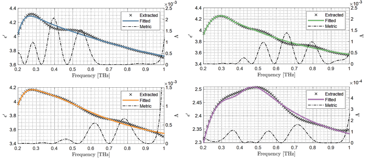
Figure II.30: Fitting of the real part of the dispersion profiles of each phantoms. Blue: #1 phantom; Green: #3 phantom; Yellow: #4 phantom; Purple: #5 phantom. Black dashed line represents the \Lambda metric.
