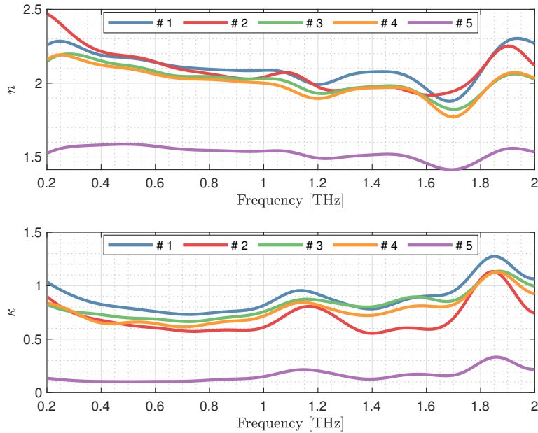
Figure II.28: Frequency dependence of the refractive index and the extinction coefficient of each samples.
