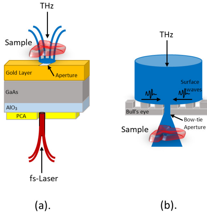
Figure IV.5: Near-field sensing with illuminated sub-wavelength aperture. Note that the sample may either be upstream or downstream the sub-wavelength aperture. a: the terahertz beam passes through the sample and subsequently through a sub-wavelength gold aperture. The electric component of the transmitted field is detected by a low temperature grown GaAs photoconducting antenna [15]. b: the incident terahertz beam is sent onto a bull's eye structure that activates surface waves. The resonant excitation of those waves allow to increase the amplitude of the electric field that is detected. Terahertz passes through a bow-tie aperture and interacts with the investigated sample [17].
