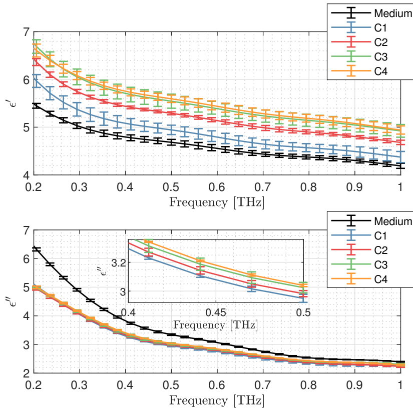
Figure II.39: Dispersion profiles of the real and imaginary part of the dielectric constant for each cell concentration.
