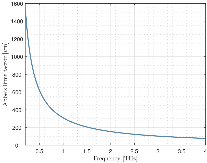
Figure III.2: Abbe's limit between 200 GHz and 1 THz in free space for \theta_0 = \frac{\pi}{6} .
