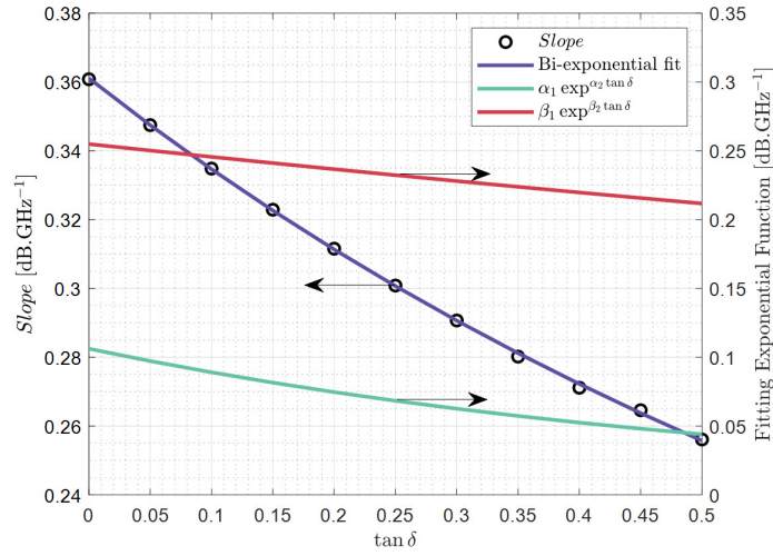
Figure IV.16: Slope as defined in equation IV.7 as a function of \tan\delta with \alpha_1 = 0.106 , \alpha_2 = -1.761 , \beta_1 = 0.255 and \beta_2 = -0.371 .
