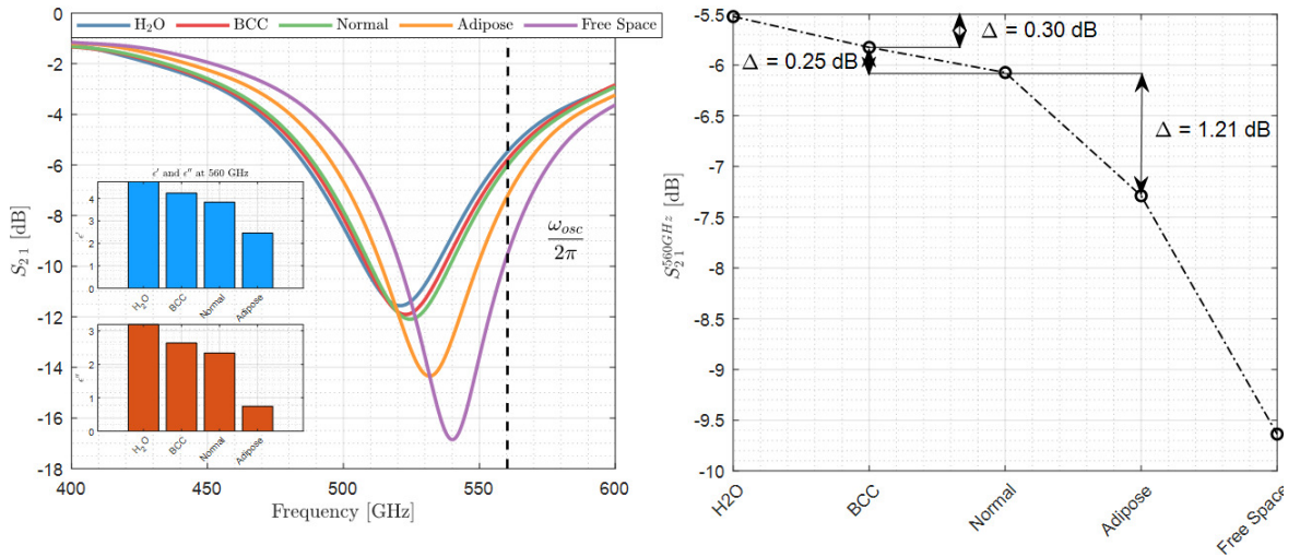
Figure IV.19: Profile of S_{21} for water, BCC, normal and adipose tissue. Left: Highlights of the LC-circuit response to biological tissues. The inset depicts the values of \epsilon' and \epsilon'' for each tissue types and water at 560 GHz as derived from the parameters in Table IV.3. Right: Behavior of S_{21} at 560 GHz as a function of the considered tissues. Simulated differences in S_{21} between the different samples are highlighted.
