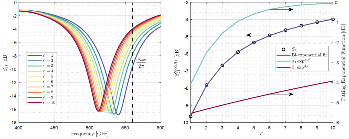
Figure IV.14: Profile of S_{21} as a function of different \epsilon' . Left: Highlight of the induced frequency shift due to the progressive increase of \epsilon' . Right: Bi-exponential behavior of S_{21} as a function of the \epsilon' relative permittivity at 560 GHz, with \alpha_1 = -6.675 , \alpha_2 = -0.488 , \beta_1 = -5.755 and \beta_2 = -0.038 .
