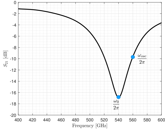
Figure IV.12: S_{21} parameter profile between 400 GHz and 600 GHz highlighting the presence of a nominal resonance frequency ( \frac{\omega_0}{2\pi} ) at 540 GHz. The sensor illumination ( \frac{\omega_{osc}}{2\pi} ) is proceeded at 560 GHz.
