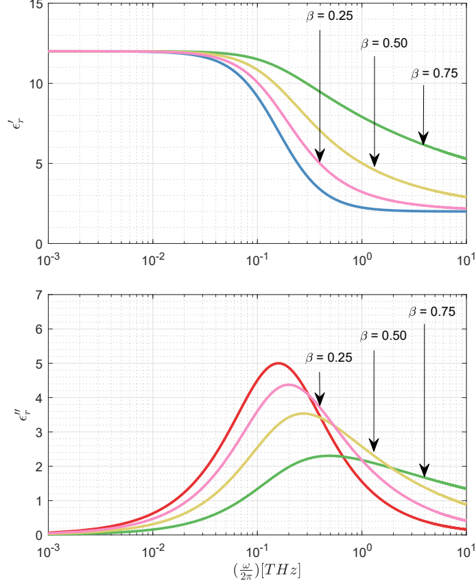
Figure I.6: Illustration of the Cole-Davidson treatment for the Debye parameters used in Figure I.4 and for \beta = 0.25, 0.50, 0.75 subsequently.
