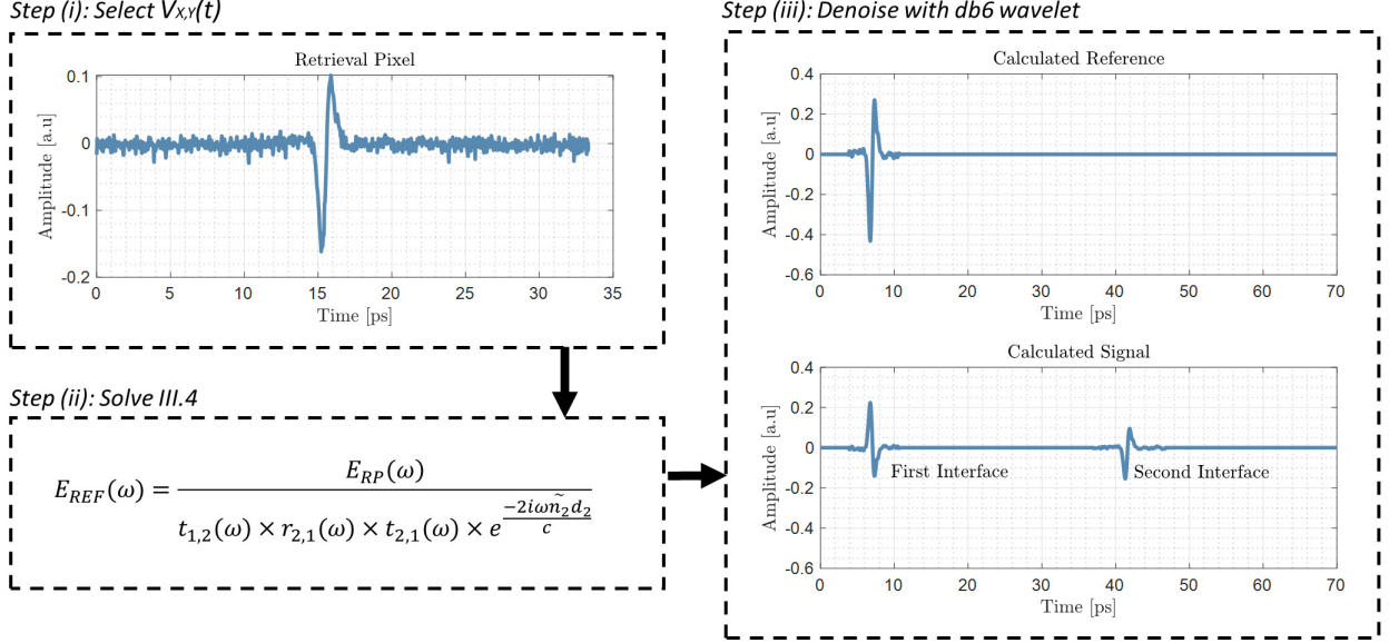
Figure III.10: Block diagram of the self-reference method. (i). A retrieval pixel is selected; (ii). Signal inversion is performed to calculate the reference signal; (iii). The reference signal is denoised by means of db6 wavelet. Eventually, the complete signal of the retrieval pixel arising from the interaction of the calculated reference with the two dielectric interfaces is retrieved. Note that the time-scale is relative rather than absolute.
