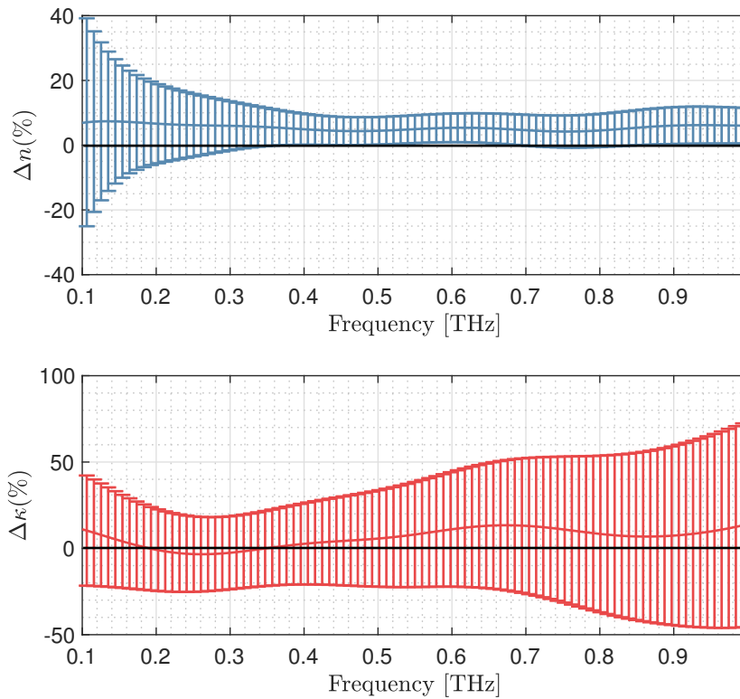
Figure II.35: Refractive index and extinction coefficient difference between healthy fibrous and cancer as a percentage of cancer characteristics.
