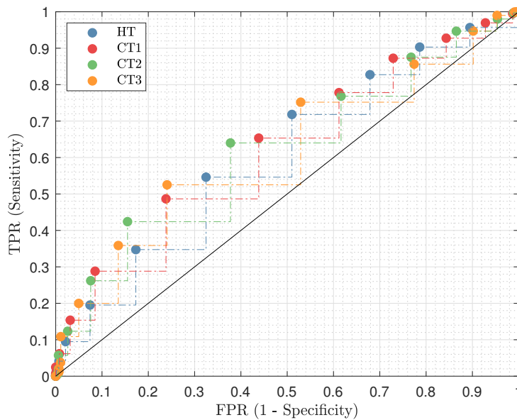
Figure III.30: Receiver operating characteristic for the different classification methods. The black line represents TPR = FPR , at 560 GHz.
