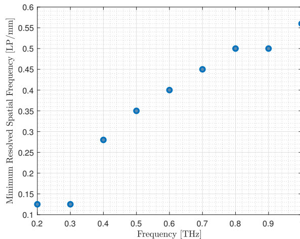
Figure III.4: Minimum resolved spatial frequency corresponding to at least a contrast of 30% as a function of the sensing terahertz frequency.
