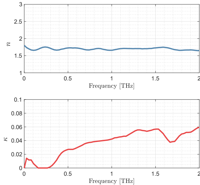
Figure II.19: Optical properties n(\omega) and \kappa(\omega) for 63.4 \mu\text{m} .
