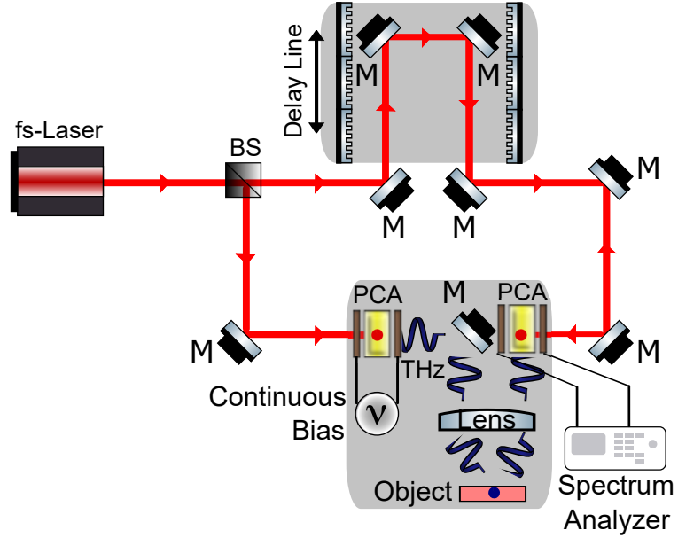
Figure II.5: Schematic details of a time-domain system for terahertz spectroscopy in reflection configuration. BS stands for beam splitter, and M depicts mirrors.
