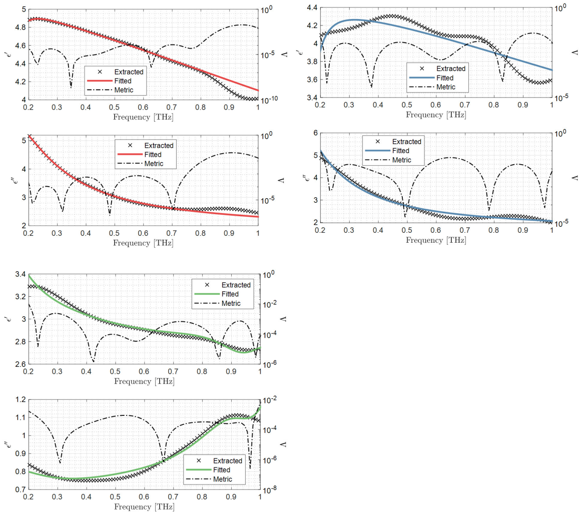
Figure II.36: Fitting of the dispersion profiles of the mean response of cancer (solid red), fibrous (solid blue) and adipose tissue (solid green). Dashed black line represents the \Delta metric between measurement and fitting.
