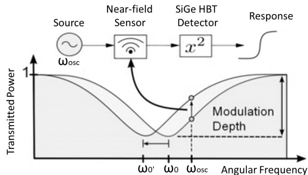
Figure IV.10: Block-diagram of the measurement operation. The resonance shift is interpreted as amplitude transmission changes from opaque to lucent at the terahertz power detector output.
