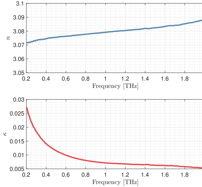
Figure II.22: Refractive index and extinction coefficient of the sapphire substrate.
