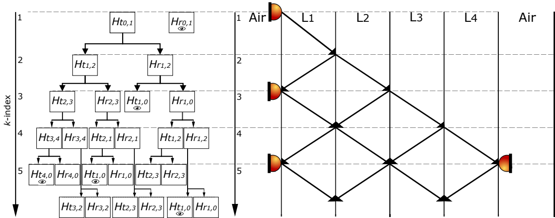
Figure II.8: Scheme of the iterative determination of S_{sam}(\omega) . Each k -incrementation gives access to further possible events based on the previous ones at k - 1 . Detected pulses have been marked with an eye in the node box. The incident angle was tilted for visual convenience.
