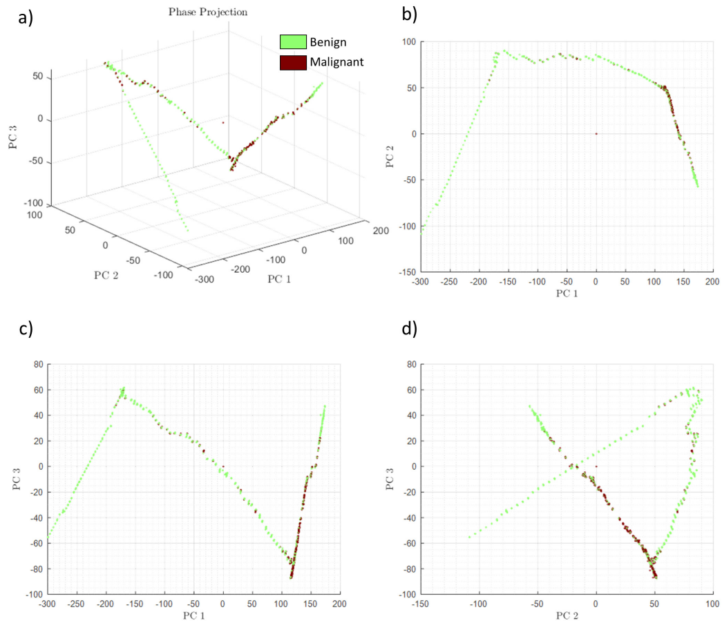
Figure III.43: Phase data set projection on the PC1-PC2-PC3 space. a) 3D projection on PC-PC2-PC3 space. b) PC2(PC1) projection. c) PC3(PC1) projection. d) PC3(PC2) projection.
