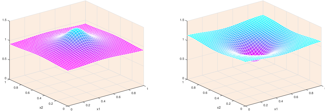
(a) Equilibrium configuration for A/B = 50
