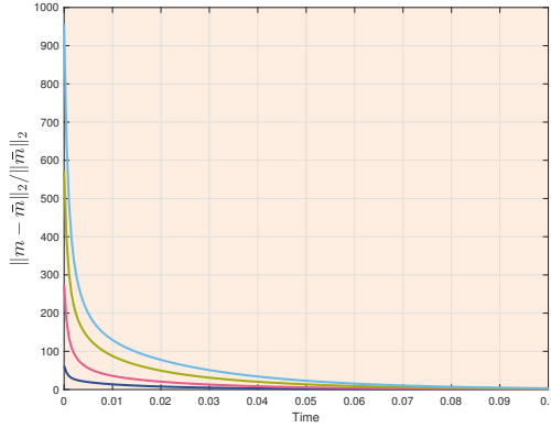
(a) H(x, p) = |p|^2/2
