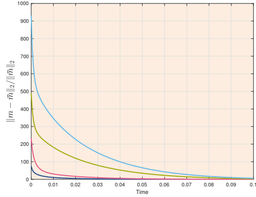
(b) H(x, p) = (\sin(2\pi x_2) + \sin(2\pi x_1) + \cos(4\pi x_1))|p|^3/3
