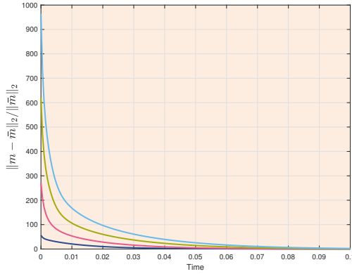
(c) H(x, p) = |p|^3/3
