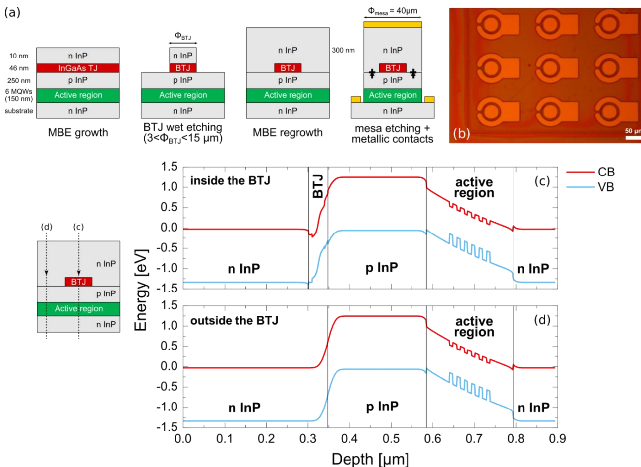
Fig. 2.24 – Sample 6195, InGaAs-BTJs: (a) realization process and (b) microscope photograph of the tested devices. Band diagrams of the structure (c) inside and (d) outside the BTJ.
