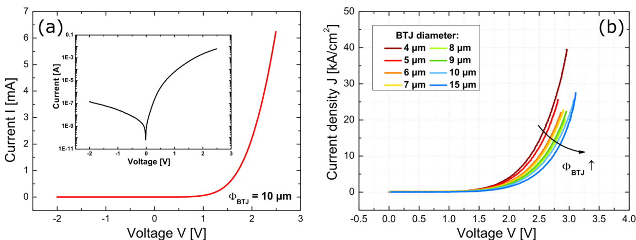
Fig. 2.25 – Electrical characterization of the BTJ-based LEDs: (a) I - V characteristic of a 10 \mu\text{m} -diameter BTJ sample (the inset shows the same curve in log scale) and (b) J - V characteristic for different diameters of the BTJ.
