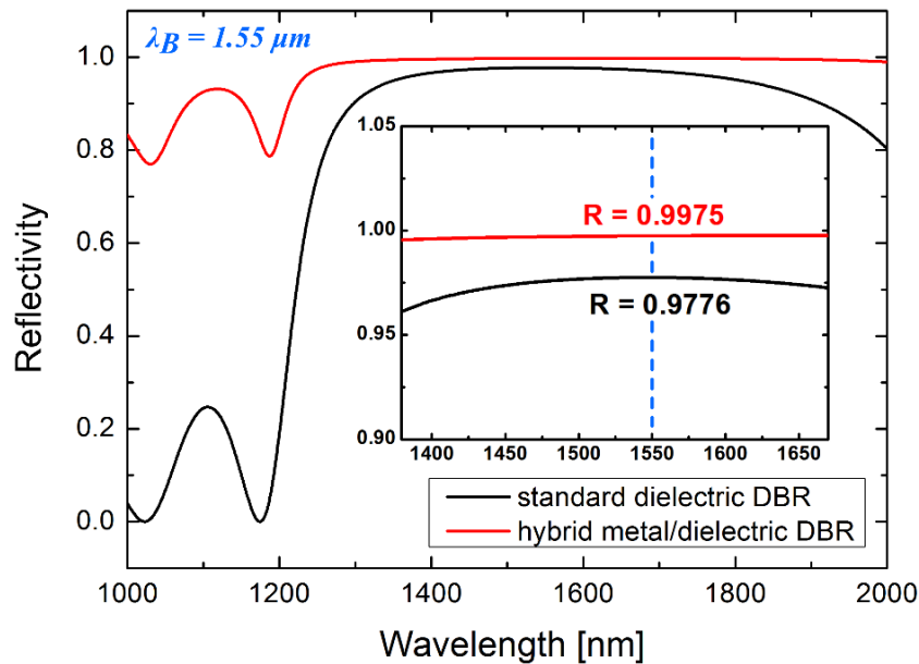
Fig. 2.5 – Comparison between a standard dielectric DBR (black) and its corresponding hybrid version (red). Both mirrors integrate 3.5 pairs of a\text{-Si}/a\text{-SiN}_x layers and have been designed at 1.55 \mu m .
