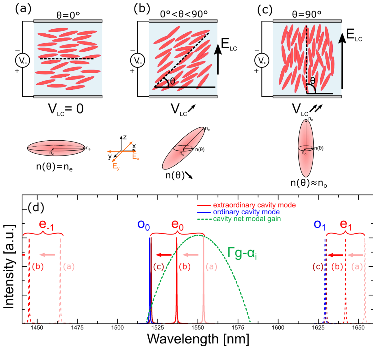
Fig. 3.4 – Optical modulation of a nematic liquid crystal under the application of an external electric field: (a) no field applied, (b) small electric field applied and (c) maximum field applied. The dashed black curve indicates the director (or optical axis) of the LC. (d) Working principle of the tuning mechanism based on the modulation of the optical response of a LC under the application of an AC voltage as the external electric field E_{LC} increases from a) to c), for a LC thickness of 5 \mu\text{m} . o =ordinary and e =extraordinary modes. Solid lines are related to the principal modes of the cavity ( e_0, o_0 ), while dashed lines to upper ( e_1, o_1 ) or lower ( e_{-1}, o_{-1} ) modes.
