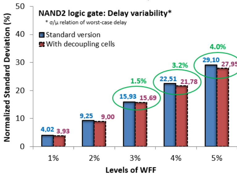
Figure 5.12: Delay variability of NAND2 gate with different levels of WFF considering the \sigma/\mu relation of worst-case delay
