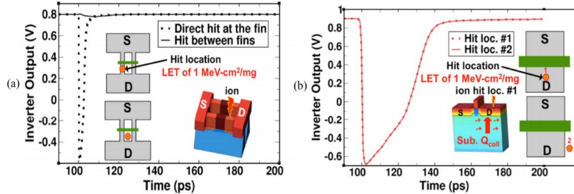
Figure 3.20: Impact of transistor structure on low-LET for (a) 16-nm FinFET and (b) 28-nm planar technologies using 3D TCAD simulations
