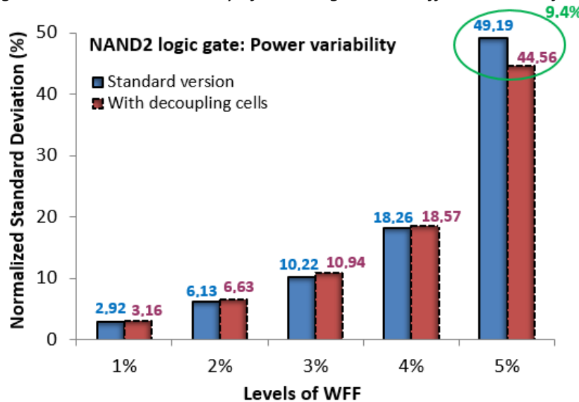
Figure 5.13: Power variability of NAND2 gate with different levels of WFF
