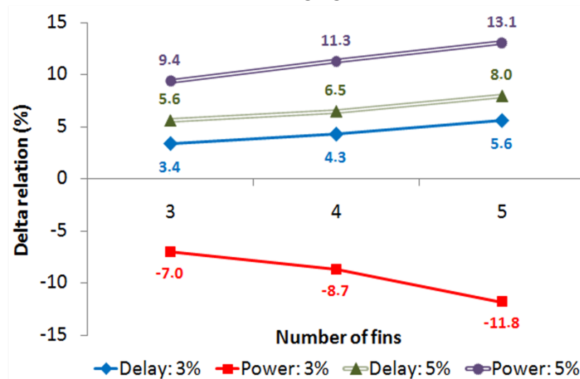
Figure 5.14: Improvements in connecting decoupling cells with different number of fins in the output of NAND2 logic gate
