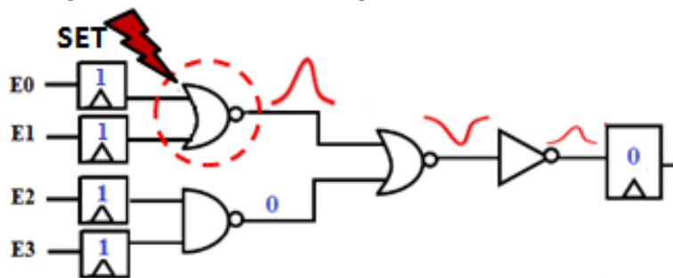
Figure 3.13: Electrical masking in a combinational circuit
