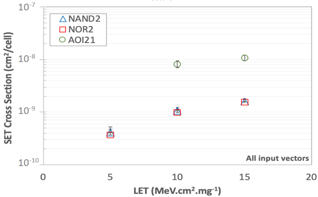
Figure 4.10: SET cross section of logic cells operating at near-threshold regime considering all input vectors
