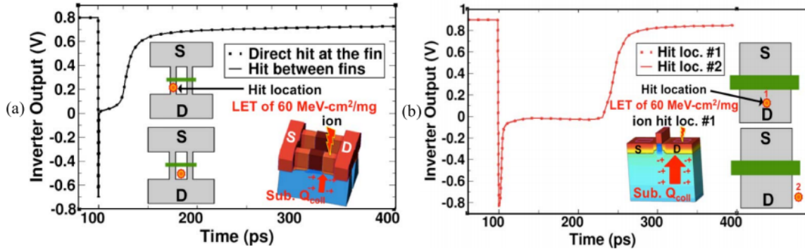
Figure 3.21: Impact of transistor structure on high-LET for (a) 16-nm FinFET and (b) 28-nm planar technologies using 3D TCAD simulations
