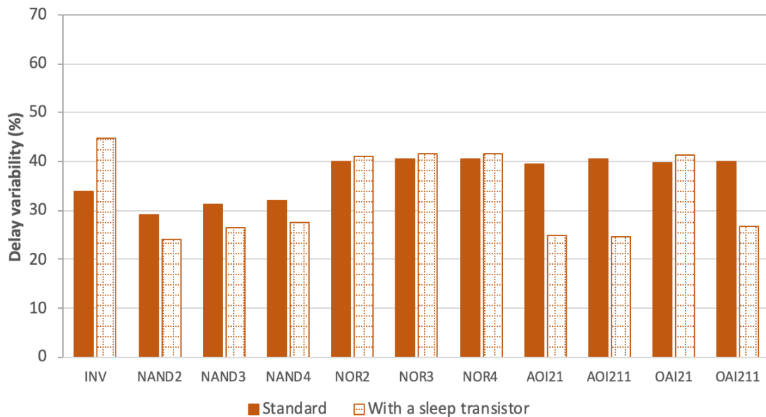
Figure 5.27: Delay variability using a sleep transistor
