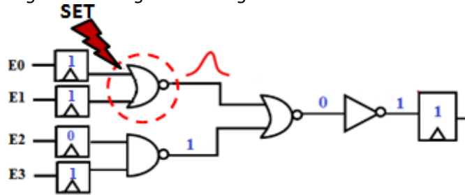
Figure 3.12: Logical masking in a combinational circuit
