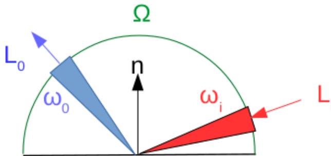
Figure 2.13 – Reflectance scheme.
