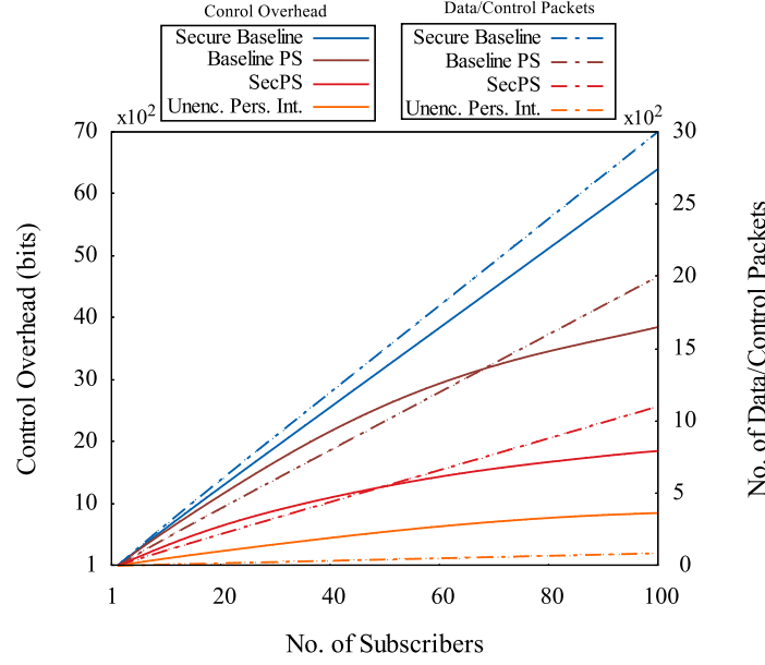
Figure 4.2 Control overhead performance.
