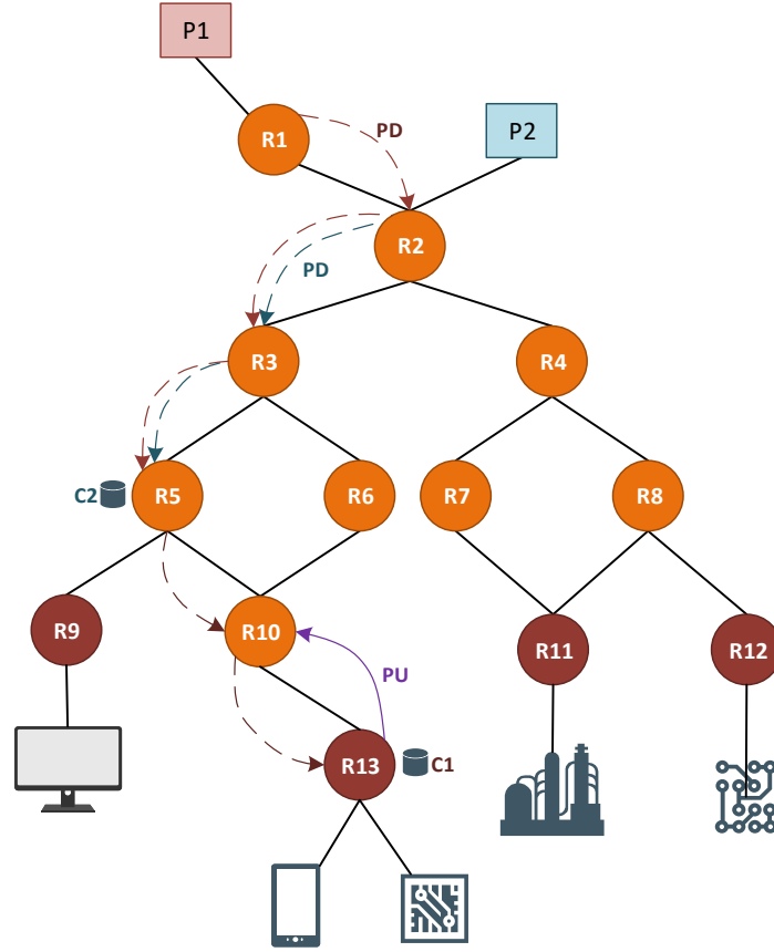
Figure 5.1 PDPU cache flow example.
