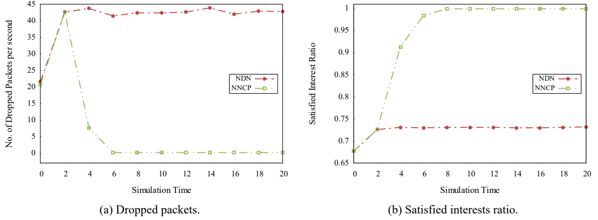
Figure 6.7 Bottleneck link simulation results.
