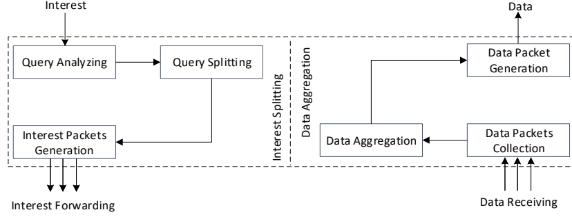
Figure 3.6 In-network function module.
