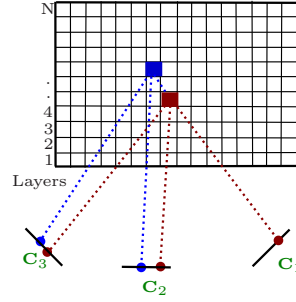
Fig. 2.20 Identifying explicitly the occluded voxel thanks to plane-sweeping from the nearest to the furthest from the cameras: in C_1 , the blue voxel is occluded by a previously validated red voxel [62].
