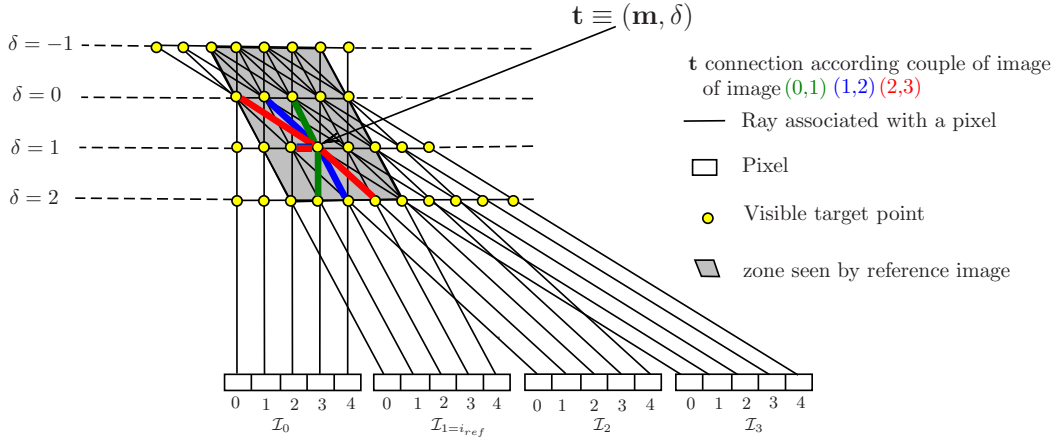
Fig. 3.17 Problem of scanline optimization in multi-stereovision. The figure is dedicated to RECOVER3D project (four cameras for each multiscopic unit) and illustrated with different possibilities to choose neighbors for a target point.
