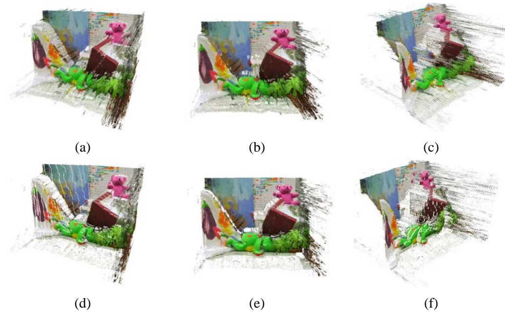
Fig. 3.23 Materiality map results: Three different views for target points extracted from adaptive scanline optimization (first row) and segmentation by graph cut (second row) using four images of Teddy dataset.
