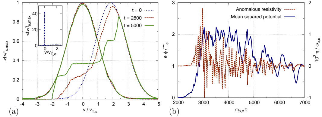
Figure 5.19 – CDIA simulation with mass ratio m_i/m_e = 1836 and system size L = 40\pi\lambda_D . (a) Snapshots of the ion (left) and electron (right) velocity distributions. Note that ion and electron distributions are not on a same scale. The inset shows them on a same scale. (b) Time-evolution of the mean square potential (left axis) and anomalous resistivity (right axis).
