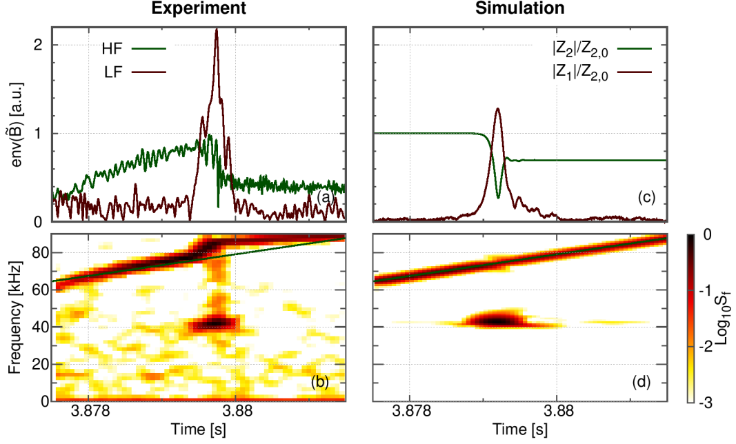
Figure 4.37 – Comparison of the evolution of perturbation between the experiment and the simulation. (a) Time evolution of magnetic perturbation, filtered into low (LF) and high frequency (HF) components. Here, "env" refers to the envelope. (b) Spectrogram of magnetic perturbation. (c) Time evolution of the amplitudes of modes 1 and 2 in the simulation. (d) Spectrogram of the total field. Superimposed curve in (b) and (d): \omega_2(t) used as input in the model.
