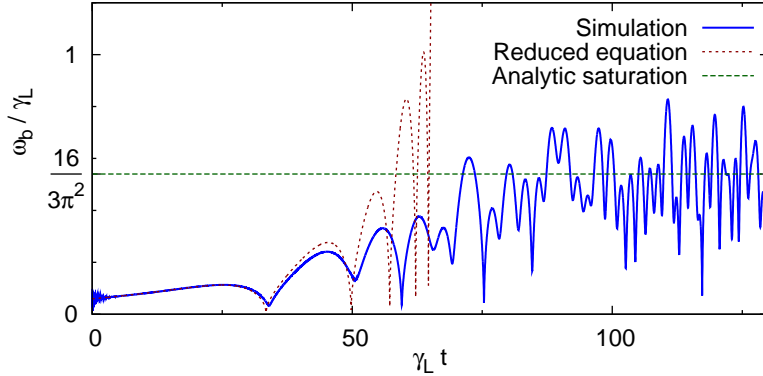
Figure 4.6 – Time evolution of the normalized field amplitude, obtained from full- f simulation and from the reduced equation (4.40), with initial distribution B, \gamma_d = 0.035 , and \nu_a = 10^{-4} .
