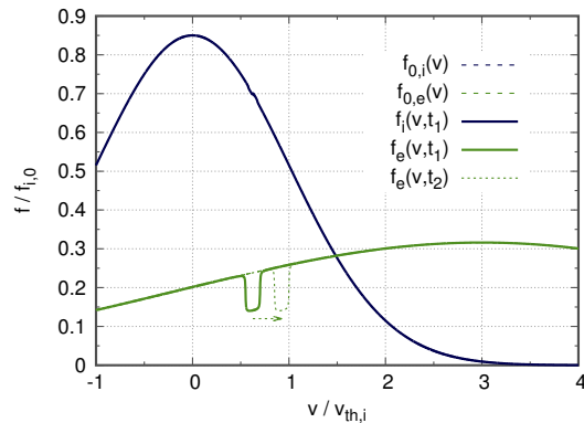
Figure 3.10 – Velocity distribution of ions and electrons in a two-species plasma, with a mean velocity drift. The equilibrium distributions are noted f_{0,i} and f_{0,e} . The ion/electron mass ratio is reduced to 10 for the sake of readability of the figure. An electron hole is drawn schematically at some arbitrary time t = t_1 . and the mechanism of its growth from t = t_1 to a later time t_2 is explained in the text as the result of a drag force due to the scattering of ions by the electron hole.
