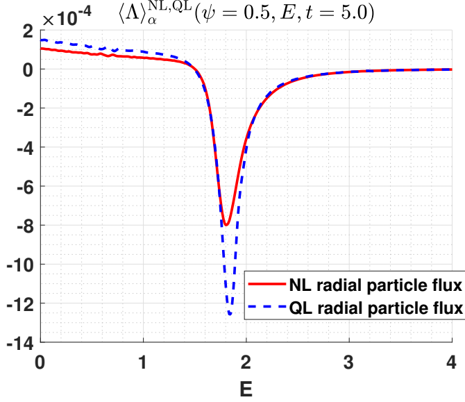
Figure 6.10 – Nonlinear and quasi-linear radial PS density fluxes against the energy (here normalized to T_i ), at t = 5 . Negative \Lambda means flux from core to edge.
