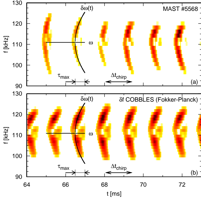
Figure 4.30 – (a) Spectrogram of magnetic fluctuations in the MAST discharge #5568, obtained with a moving Fourier window of size 2 ms. Logarithmic colour scale spanning 3 orders of magnitude. (b) Spectrogram of the electric field, obtained with a moving Fourier window of size 0.6 ms, where the input parameters of the \delta f BB model were chosen to fit (a). Solid curves show the analytic prediction for the chirping velocity and lifetime, with a non-adiabaticity correction parameter \beta = 0.65 .
