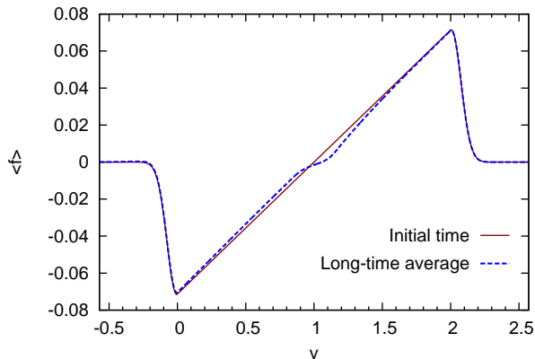
Figure 4.32 – Initial (solid line), and long-time averaged (dashed line) velocity distribution function, for the simulation shown in Fig. 4.31. Here, \langle f \rangle is the average over 20ms of the velocity distribution.
