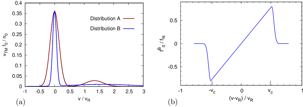
Figure 4.1 – Examples of initial distribution function. Here, velocity is re-normalized to the resonant velocity v_R . (a) Full- f case. (b) \delta f case, where f_N \equiv \gamma_{L0}/(\sqrt{2\pi}v_R) .
