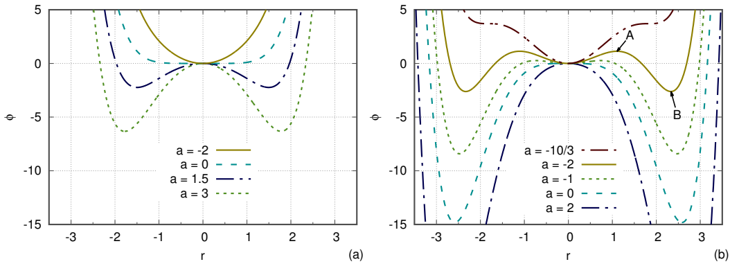
Figure 3.2 – Potential \phi(r) for various values of a . We recall that a is proportional to the square of the linear growth rate. (a) Supercritical case, b = 0 . (b) Subcritical case, b = 1 . Two points are shown by arrows: point A is the potential barrier at r = r_{\min} , and point B is the saturated value for the subcritical instability, r = r_{\max} .
