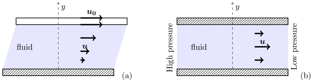
Figure 3.8 – (a) Cartoon of the plane Couette flow setup. A fluid is contained between two plates, both normal to the y -axis. The bottom plate is fixed, as illustrated by hashes. The upper plate is moving at a given velocity u_0 . (b) Cartoon of the plane Poiseuille flow setup. A fluid is contained between two plates, both normal to the y -axis, and both fixed. The pressure is higher at the inlet than at the outlet.
