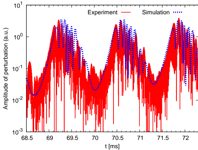
Figure 4.31 – Time-evolution of the perturbation. The signal is filtered between 90 and 130 kHz. The parameters of the simulation are shown in Tab. 4.1. For the simulation, to avoid hiding experimental data, we show the amplitude of perturbations (the envelope) instead of the perturbations themselves. Note the use of arbitrary units (we compare normalized quantities only).
