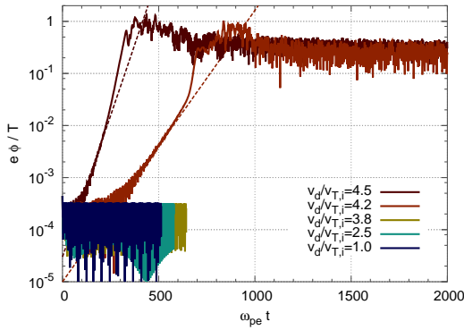
Figure 5.3 – Time-evolution of the normalized potential energy for small, incoherent initial perturbation, e\phi/T \approx 2 \times 10^{-4} . Linear theory is shown as dashed lines.
