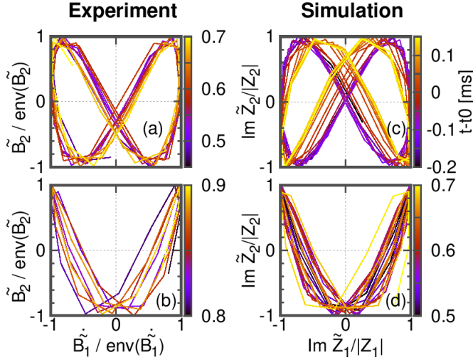
Figure 4.41 – Lissajous figure during the growth (a), and the decay (b) of daughter mode in the experiment, and (c-d) in the simulation. For the simulation, \tilde{Z}_i \equiv Z_i e^{-i\omega_i t} . Colorbars show the time shifted by t_0 = 3.879 s.
