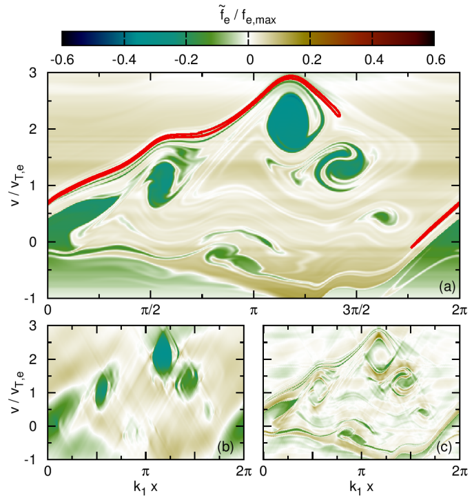
Figure 5.28 – Snapshot at \omega_{p,e}t = 10560 of the perturbed electron distribution \tilde{f}_e , normalized to f_{e,\max} = f_e(v_{0,e}) , for a driven system. The mass ratio is m_i/m_e = 4 .
