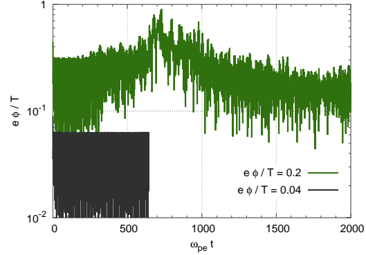
Figure 5.4 – Time-evolution of the normalized potential energy for v_d/v_{T,i} = 3.8 and various levels of incoherent initial perturbation.
