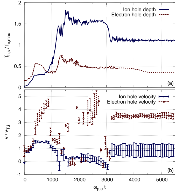
Figure 5.8 – Time-evolution of the depth (a) and velocity (b) of the deepest negative phase-space density perturbation in the reference case S. The velocity width is shown by error bars at \pm\Delta v_h .
