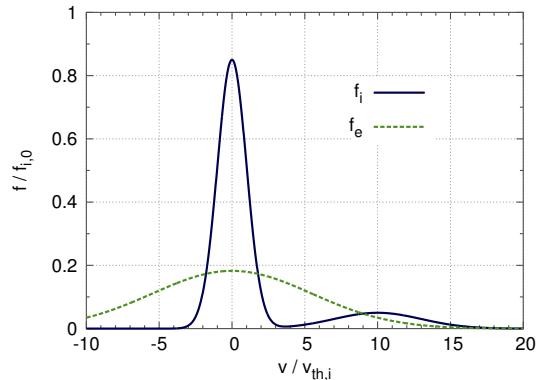
Figure 3.9 – Velocity distribution of ions (solid curve) and electrons (dotted curve) in a two-species plasma, with a population of supra-thermal particles, and equal bulk ion and electron temperatures. The ion/electron mass ratio is reduced to 30 for the sake of readability of the figure.
