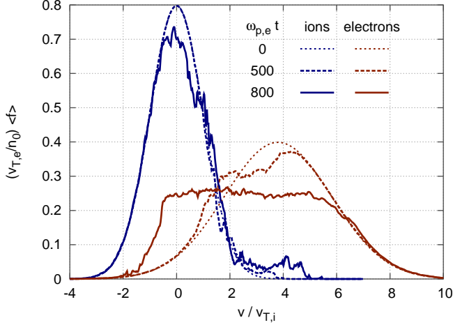
Figure 5.2 – Snapshots of the velocity distributions in a subcritical case. Simulation parameters are v_d/v_{T,i} = 3.8 , e\phi/T \approx 0.2 , and N_x \times N_v = 768 \times 8192 .
