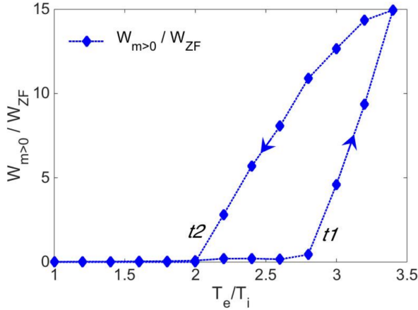
Figure 6.17 – Ratio of turbulent energy W_{m>0} over zonal flow energy W_{ZF} , against electron/ion temperature ratio. Arrows indicate the direction of time.
