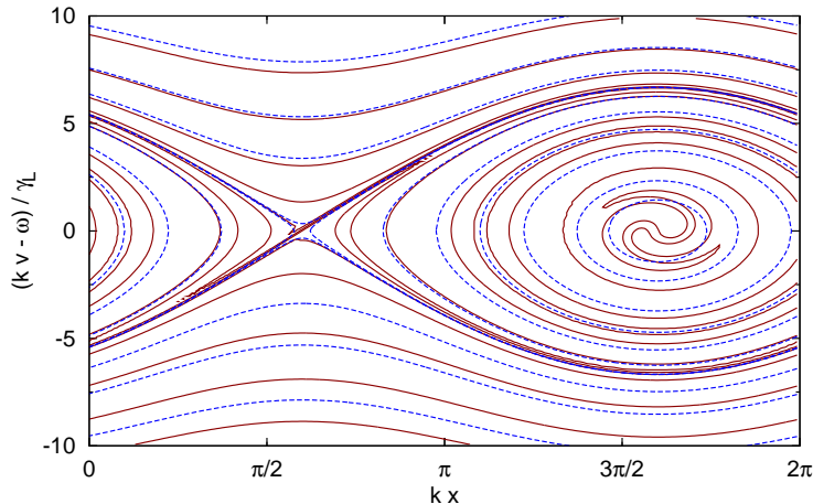
Figure 4.3 – Contour plot of the time-asymptotic distribution function (solid curves) and constant energy curves (dashed curves) for the simulation of Fig. 4.2.
