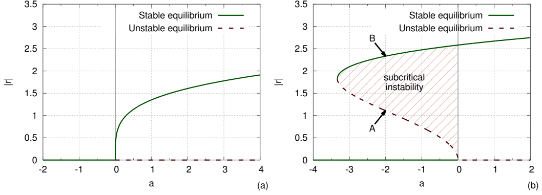
Figure 3.3 – Bifurcation diagram, which yields the nonlinear stability. The solid curves are the stable equilibria |r| = 0 and |r| = r_{\max} , which correspond to the saturation amplitude. The dashed curves are the unstable equilibria |r| = 0 and |r| = r_{\min} , which correspond to the threshold amplitude. (a) Supercritical system, b = 0 . (b) Subcritical system, b = 1 . The region of subcritical instability is shown by hashes. The same points A and B as in Fig. 3.2 are shown by arrows in this figure as well.
