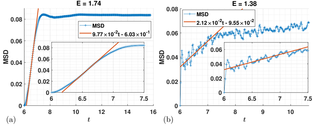
Figure 6.15 – Time-evolution of the test particles Mean Square Displacement (MSD). Here, time is normalized to the precession frequency of thermal ions, \omega_0 . (a) Simulation A, for E = 1.74T_i . (b) Simulation B, for E = 1.38T_i .
