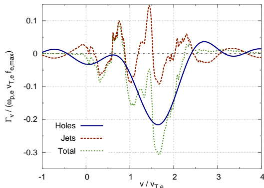
Figure 5.17 – Velocity-direction particle flux at \omega_{p,e}t = 1180 (mass ratio m_i/m_e = 4 ).
