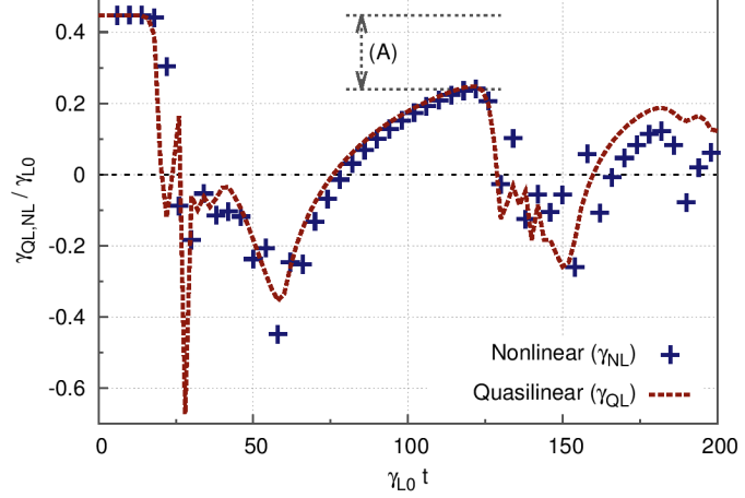
Figure 4.23 – Time-evolution of the growth rate in our reference case. Points: obtained from the time-series of electric field amplitude (Fig. 4.20, dashed curve). Dashed curve: obtained from the linearized equations and the Gaussian model for \partial\langle f \rangle/\partial v . In the absence of hole and clump, \gamma/\gamma_{L0} = 0.4476 . (A) shows the discrepancy between the latter value and the maximum growth rate reached before the second burst.
