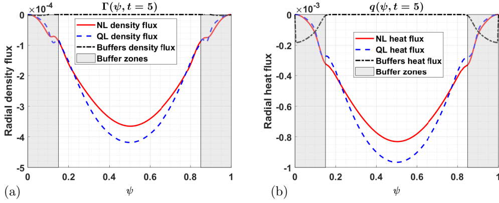
Figure 6.11 – Radial density (a) and heat (b) fluxes as a function of radius, at t = 5 .
