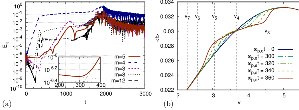
Figure 4.43 – Simulation with n_M = 0.9n_0 . (a) Time-evolution of the amplitudes of Fourier modes k = nk_1 of electric field. Inset: zoom near the time of reversal of evolution of mode n = 5 . In the inset, the two dashed lines correspond to growth rates \gamma_{5,L} = -0.0008\omega_{pe} and \gamma_{5,sec} = 0.012\omega_{pe} . (b) Spatial average of the distribution function. Vertical lines indicate the phase velocities v_n = \omega_{n,L0}/k_n of modes k_n = nk_1 .
