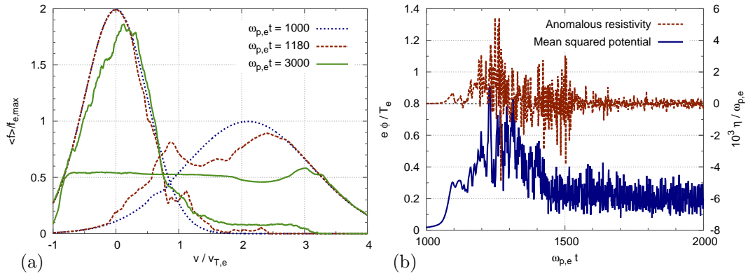
Figure 5.13 – CDIA simulation with mass ratio m_i/m_e = 4 , system size L = 10\pi\lambda_D and initial drift v_d = 4.2v_{T,i} = 2.1v_{T,e} . (a) Snapshots of the ion (left) and electron (right) velocity distributions. (b) Time-evolution of the mean square potential (left axis) and anomalous resistivity (right axis).
