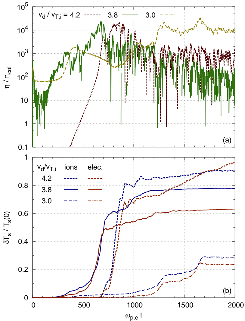
Figure 5.5 – Time-evolution of (a) anomalous resistivity, normalized to \eta_{\text{coll}} = 10^{-7} m_e \omega_{p,e} / (n_0 q_i^2) , and (b) mean thermal energy perturbation. Three cases are shown, the simulation of Fig. 5.2 ( v_d/v_{T,i} = 3.8 , solid curves), a linearly unstable case ( v_d/v_{T,i} = 4.2 , dashed curves), and the reference case S of Fig. 5.12 ( v_d/v_{T,i} = 3.0 , chained curves).
