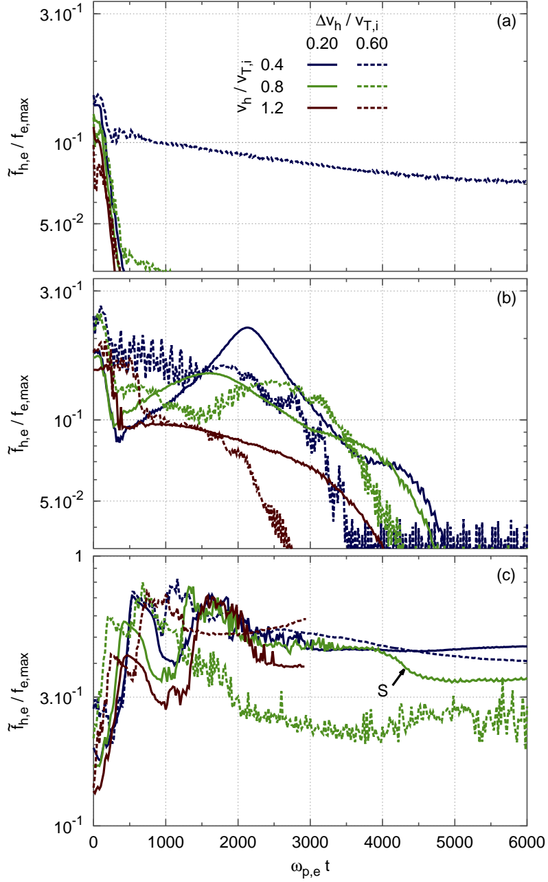
Figure 5.9 – Time-evolution of the depth of the deepest electron phase-space perturbation ( \tilde{f}_{h,e} ) with an initial electron seed with \Delta x_h / \Delta v_h = 20 / \omega_{p,e} . The initial drift v_d / v_{T,i} is (a) 0.0, (b) 1.5, and (c) 3.0. The reference simulation is marked by S in (c).
