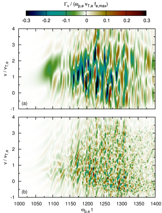
Figure 5.18 – Time-evolution of the particle flux (mass ratio m_i/m_e = 4 ). Contribution from (a) holes, (b) jets.
