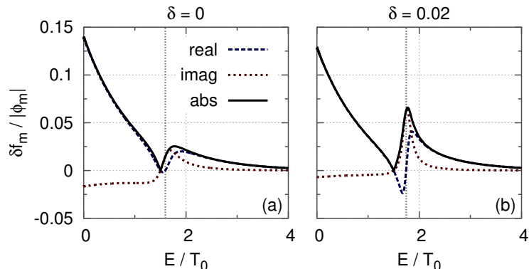
Figure 6.6 – Eigenfunction for Case 1 (flat density profile), n = 10 , at \psi = 0.5 . (a) No electron dissipation. (b) Finite electron dissipation \delta = 0.02 . A dotted vertical line corresponds to the energy such that the resonance condition \omega = n\omega_d(E) = n\Omega_d E is satisfied.
