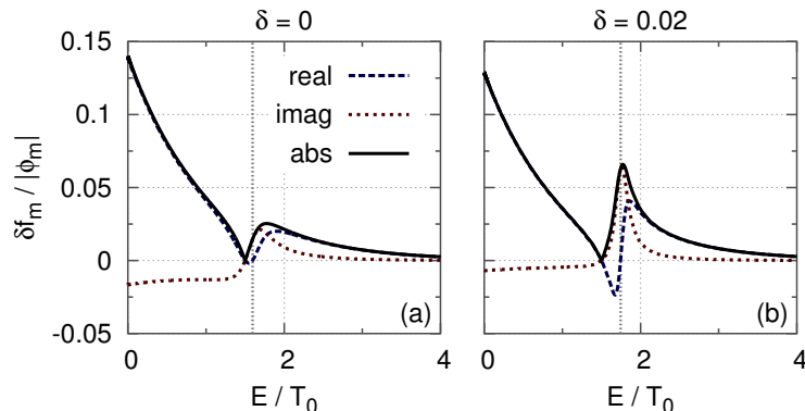
Figure 6.6 – Eigenfunction for Case 1 (flat density profile), n = 10 , at \psi = 0.5 . (a) No electron dissipation. (b) Finite electron dissipation \delta = 0.02 . A dotted vertical line corresponds to the energy such that the resonance condition \omega = n\omega_d(E) = n\Omega_d E is satisfied.
