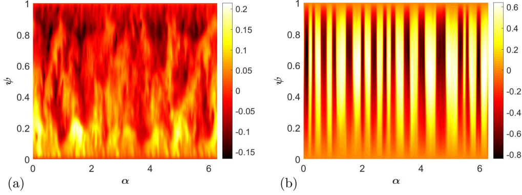
Figure 6.13 – Electric potential at t = 6 . (a) Simulation A. (b) Simulation B.
