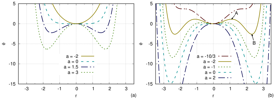
Figure 3.2 – Potential \phi(r) for various values of a . We recall that a is proportional to the square of the linear growth rate. (a) Supercritical case, b = 0 . (b) Subcritical case, b = 1 . Two points are shown by arrows: point A is the potential barrier at r = r_{\min} , and point B is the saturated value for the subcritical instability, r = r_{\max} .
