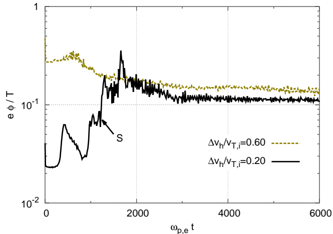
Figure 5.12 – Time-evolution of the normalized potential energy with an initial electron hole, for v_d/v_{T,i} = 3.0 , v_h/v_{T,i} = 0.8 , \Delta x_h/\Delta v_h = 20/\omega_{p,e} and varying hole velocity-width. The reference simulation is marked by S.
