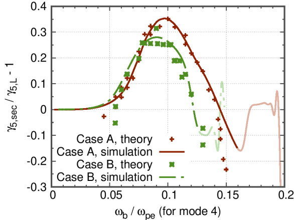
Figure 4.44 – Instantaneous growth rate of the secondary instability, versus the bounce frequency of the primary mode. Case A: n_M = 0.95n_0 , \gamma_{d,0} = 0.02\omega_{pe} ; Case B: n_M = 0.97n_0 , \gamma_{d,0} = 0.01\omega_{pe} . In both cases, v_{TM} = 0.2v_{th} , v_{TB} = 3.0v_{th} , v_B = 5.0v_{th} , n_B = n_0 - n_M , \nu_f = 0 , and \nu_d = 0.01\omega_{pe} . For each curve, the semi-transparent part corresponds to later times, where nonlinear interactions between modes appear to strongly influence the secondary mode.
