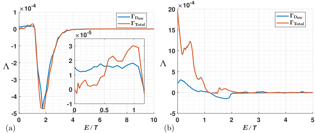
Figure 6.16 – Radial flux of phase-space density against energy. The total nonlinear flux averaged over an auto-correlation time \tau_c and a radial range \psi/L_\psi \in [0.4; 0.6] is compared with the diffusive part estimated from test-particles statistics. (a) Simulation A, \tau_c \approx \omega_0^{-1} . (b) Simulation B, \tau_c \approx 4\omega_0^{-1} .
