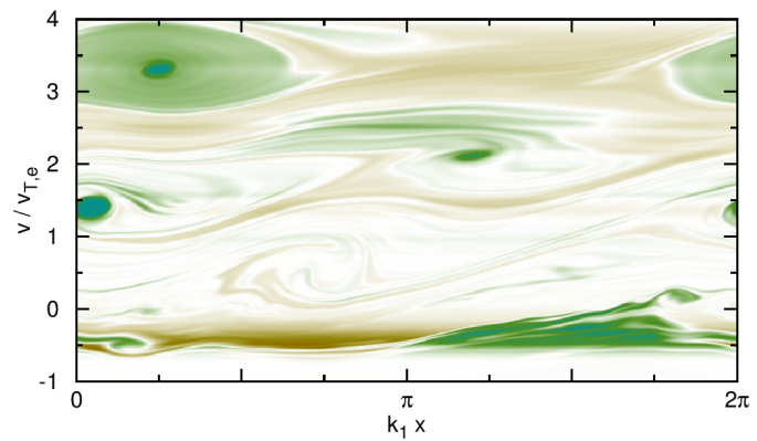
Figure 5.30 – Snapshot at \omega_{p,e}t = 20000 of the perturbed electron distribution \tilde{f}_e , normalized to f_{e,\max} = f_e(v_{0,e}) , for a driven system.
