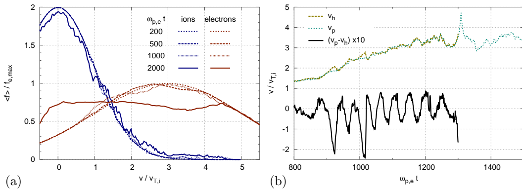
Figure 5.11 – Evolution of the reference simulation S. (a) Snapshots of velocity distributions. (b) Time-evolution of the velocity v_p of a test particle (electron) trapped in a hole with central velocity v_h(t) .
