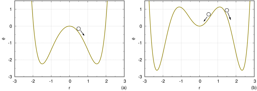
Figure 3.1 – Cartoon of the concept of supercritical and subcritical instabilities. The solid curve is a fixed potential. (a) Supercritical case, a = 1.5 , b = 0 and c = 0.1 . The equilibrium r = 0 is unstable. (b) Subcritical case, a = -2 , b = 1 and c = 0.1 . The equilibrium r = 0 is stable to small perturbations (circle and arrow at r = 0.5 ), but unstable to perturbations with an amplitude above a certain threshold (circle and arrow at r = 1.5 ).
