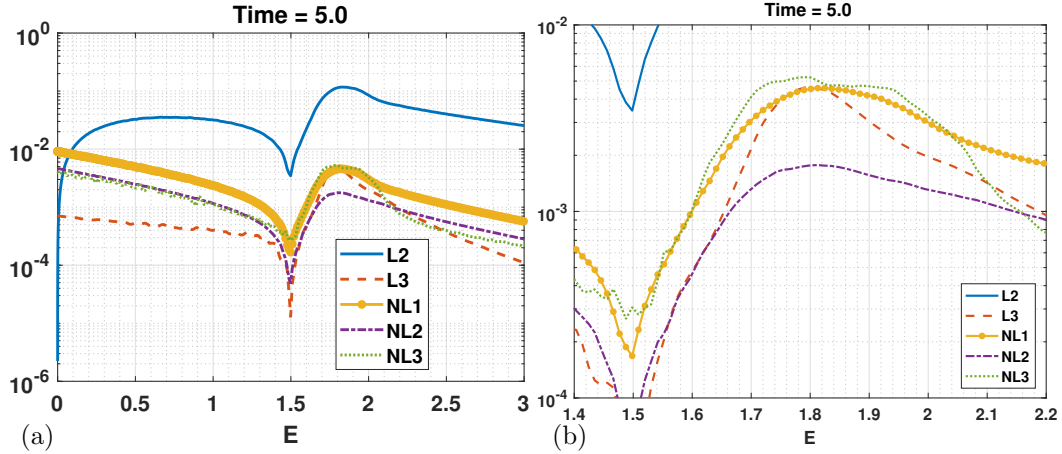
Figure 6.12 – (a) Comparison between linear and nonlinear terms of Vlasov equation. (b) Zoom around the resonance.
