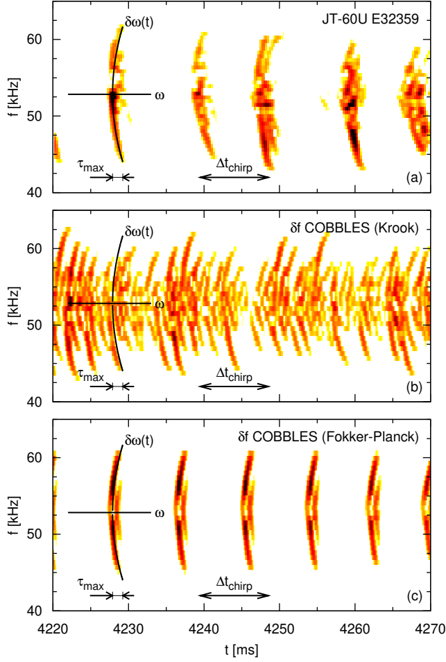
Figure 4.28 – (a) Spectrogram of magnetic fluctuations during fast-FS modes in the JT-60U discharge E32359, obtained with a moving Fourier window of size 2\text{ ms} . (b) and (c) Spectrogram of the electric field, where the kinetic parameters of the \delta f BB model were chosen to fit the magnetic spectrogram for JT-60U discharge E32359. The solid curve shows the analytic prediction for the chirping velocity. (b) Krook collisions, correction parameter \beta = 0.65 . (c) Friction-diffusion collisions, correction parameter \beta = 0.75 .
