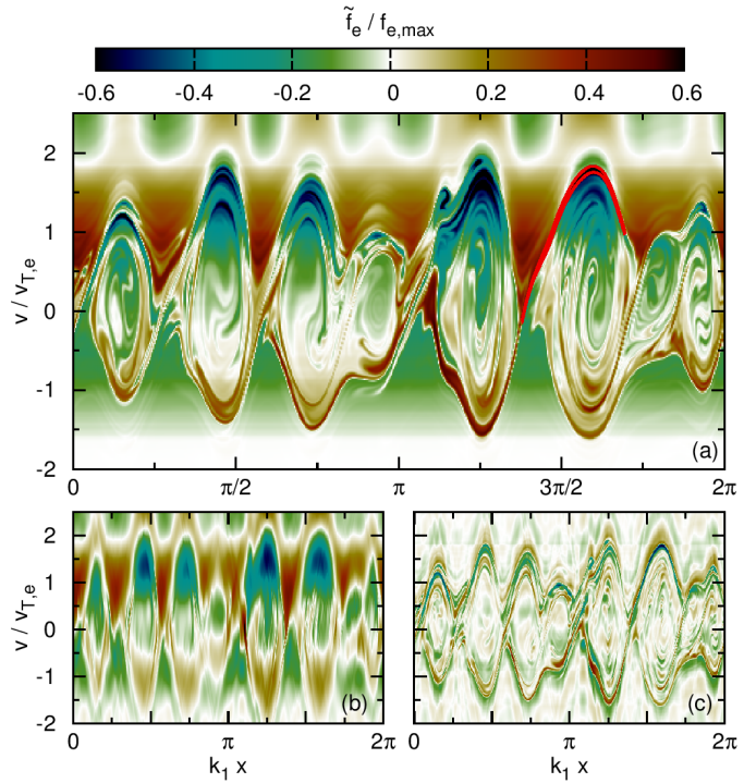
Figure 5.20 – (a) Snapshot at \omega_{p,e} t = 2800 of the perturbed electron distribution \tilde{f}_e , normalized to f_{e,max} = f_e(v_{0,e}) . Solid curve: contour of constant f_e/f_{e,max} = 0.08 . (b) Low-pass filtered \tilde{f}_{e,holes} . (c) High-pass filtered \tilde{f}_{e,jets} . The mass ratio is m_i/m_e = 1836 . The system size is 40\pi\lambda_D .
