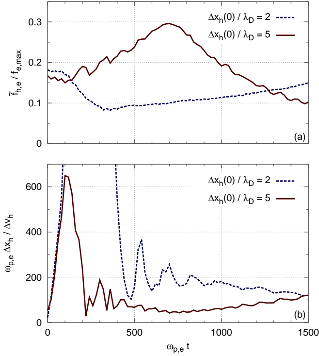
Figure 5.10 – Time-evolution of (a) the height of the largest electron hole and (b) the ratio \Delta x_h/\Delta v_h with an initial electron hole with \Delta v_h(0)/v_{T,i} = 0.2 , for v_d/v_{T,i} = 1.5 and v_h(0)/v_{T,i} = 0.4 .
