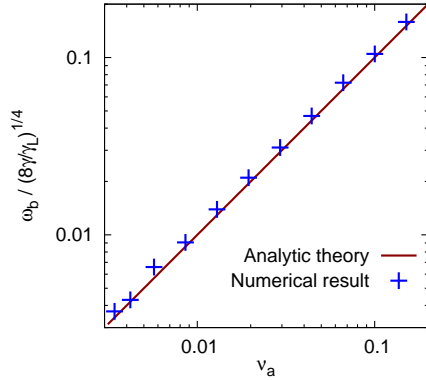
Figure 4.5 – Saturation level near marginal stability. Measured in full- f simulations for distribution B.
