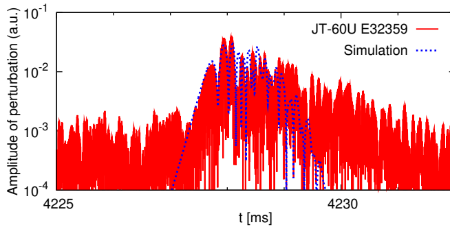
Figure 4.29 – Evolution of the amplitude of perturbations during a single chirping event. The signal is filtered between 40 and 65 kHz. In these arbitrary units, 10^{-3} roughly corresponds to a noise level. The parameters of the simulation are shown in Tab. 4.1.
