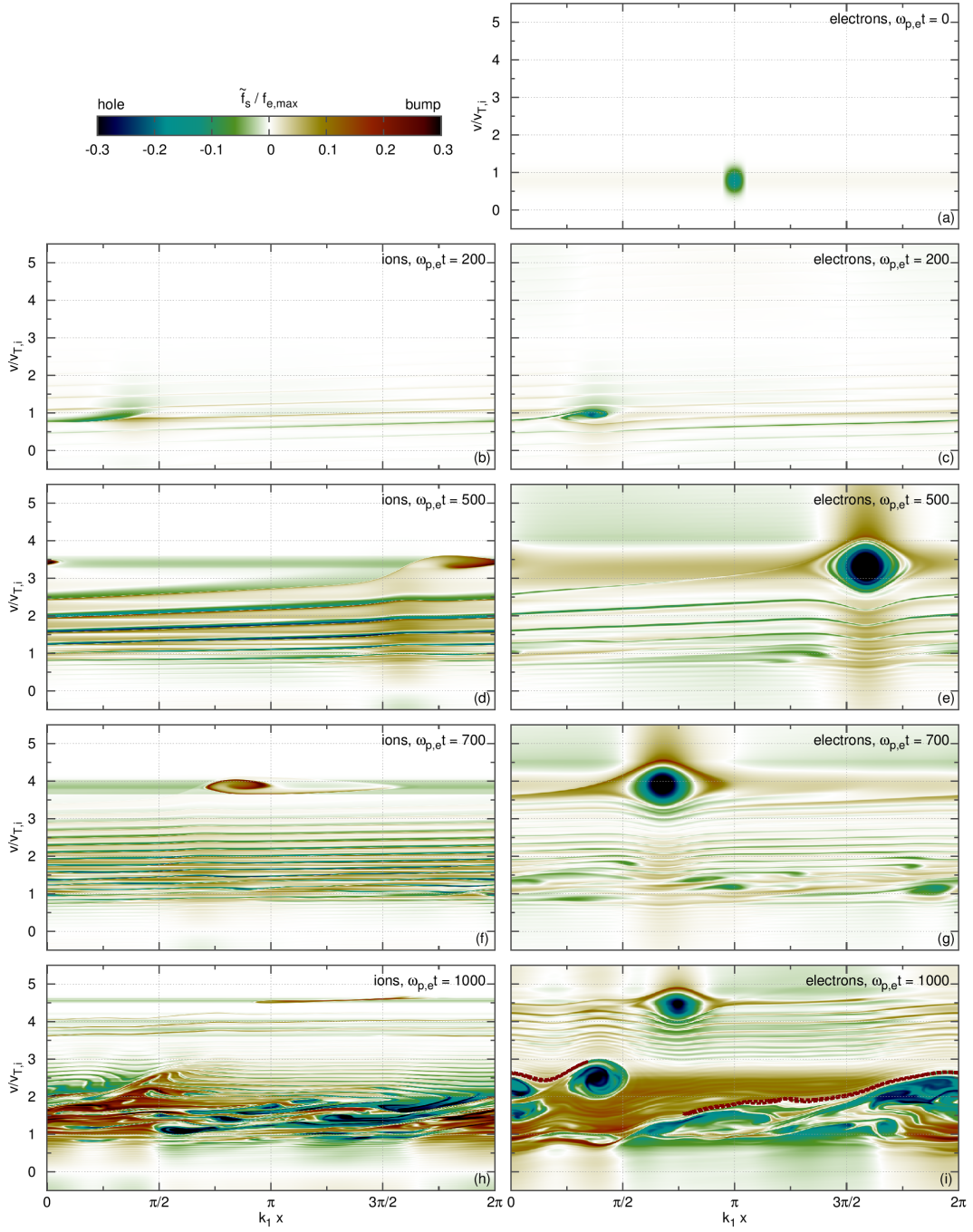
Figure 5.6 – Snapshots of ion (left) and electron (right) perturbed distribution in the reference simulation S ( v_d/v_{T,i} = 3.0 , v_h(0)/v_{T,i} = 0.8 , \Delta v_h/v_{T,i} = 0.2 , and \Delta x_h/\lambda_D = 2 ). Values of \omega_{p,e}t from top to bottom are 0, 200, 500, 700 and 1000. A contour of constant f_e is dashed in (i).
