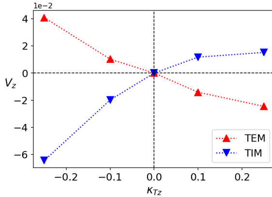
Figure 6.20 – Thermodiffusion velocity V_Z plotted against the impurity temperature gradient, for both TEM and TIM turbulent cases.
