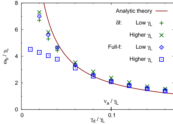
Figure 4.4 – Saturation level far above marginal stability. Here \nu_a / \gamma_L = 0.1 . Results are shown for both distribution B (Low- \gamma_L case), and a distribution with higher beam density and lower beam temperature (Higher- \gamma_L case).
