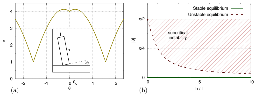
Figure 3.4 – Case of a box on a plane with height h = 4l . (a) Potential energy (normalized). Inset: cartoon of the setup, where the box is tilted by an angle \theta . (b) Corresponding bifurcation diagram. The dashed curve is the unstable equilibrium |\theta| = \tan^{-1}(l/h) , which correspond to the threshold amplitude. The region of subcritical instability is shown by hashes: it spans the whole range of finite values of the control parameter h/l .
