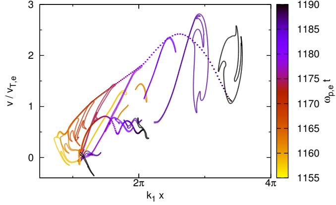
Figure 5.16 – Time-evolution of a jet. Solid: constant f_e/f_{e,max} = 0.375 contours. Dashed: orbits of two test particles. The mass ratio is m_i/m_e = 4 .
