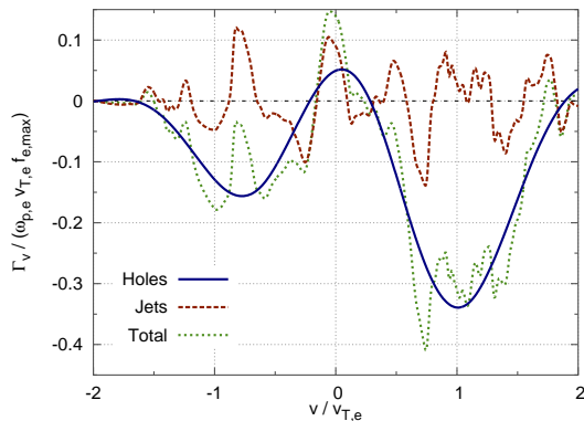
Figure 5.21 – Velocity-direction particle flux at \omega_{p,e}t = 2800 (mass ratio m_i/m_e = 1836 ).
