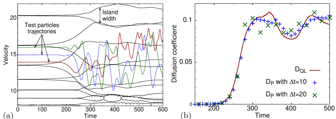
Figure 4.42 – Many waves in the Vlasov-Poisson model. (a) Evolution and overlapping of multiple islands. Dashed and dotted lines are trajectories of three test-particles. (b) Time-evolution of the quasi-linear diffusion coefficient estimated by quasi-linear theory (solid line), and by following test particles trajectories (pluses and crosses).
