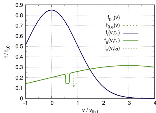
Figure 3.10 – Velocity distribution of ions and electrons in a two-species plasma, with a mean velocity drift. The equilibrium distributions are noted f_{0,i} and f_{0,e} . The ion/electron mass ratio is reduced to 10 for the sake of readability of the figure. An electron hole is drawn schematically at some arbitrary time t = t_1 . and the mechanism of its growth from t = t_1 to a later time t_2 is explained in the text as the result of a drag force due to the scattering of ions by the electron hole.
