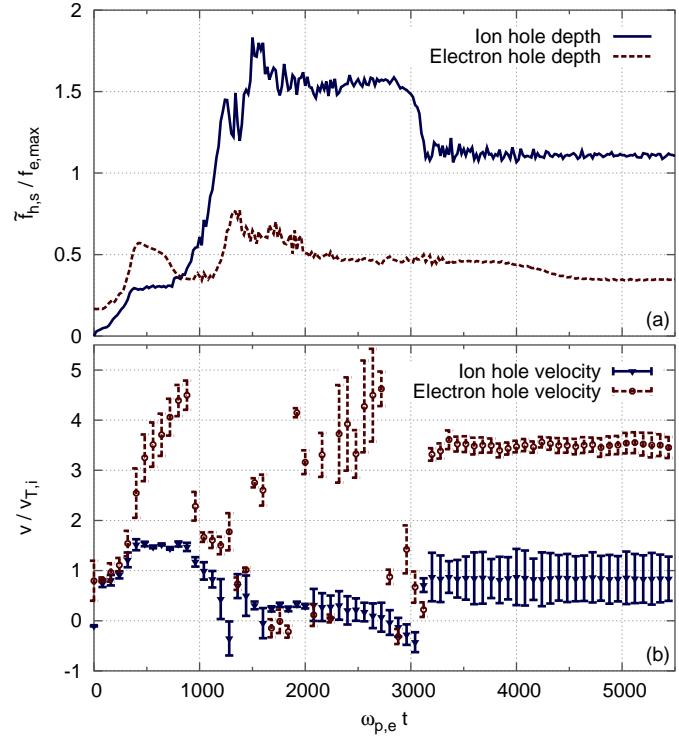
Figure 5.8 – Time-evolution of the depth (a) and velocity (b) of the deepest negative phase-space density perturbation in the reference case S. The velocity width is shown by error bars at \pm \Delta v_h .
