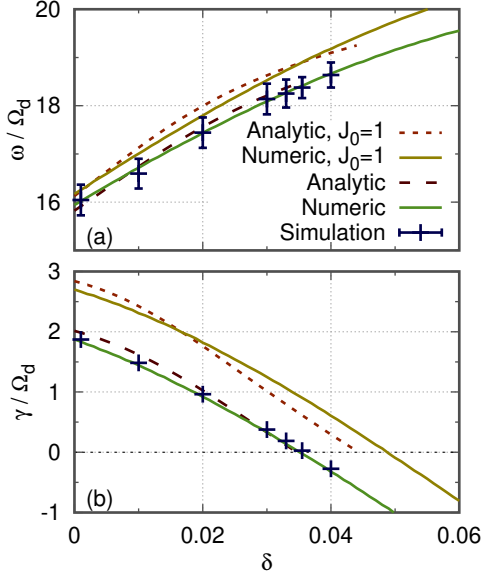
Figure 6.2 – Linear frequency (a) and growth rate (b) as a function of electron dissipation, for Case 1 (flat density profile), for a given mode ( n = 10 , k = \pi/L_\psi ). The legend is shared. ‘Analytic’, ‘Numeric’ and ‘Simulation’ refer to the analytic approximate solution of the dispersion relation, the numerical solution of the dispersion relation, and TERESA simulation.
