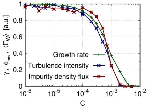
Figure 6.18 – Linear growth-rate, turbulence intensity (rms of the potential), and density flux, all versus tungsten concentration.
