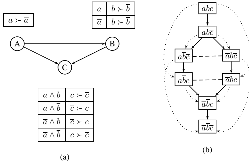
Figure 4.7: For player 1: CP-net and associated preordering for the game G^* (equivalent by rewriting of G )
