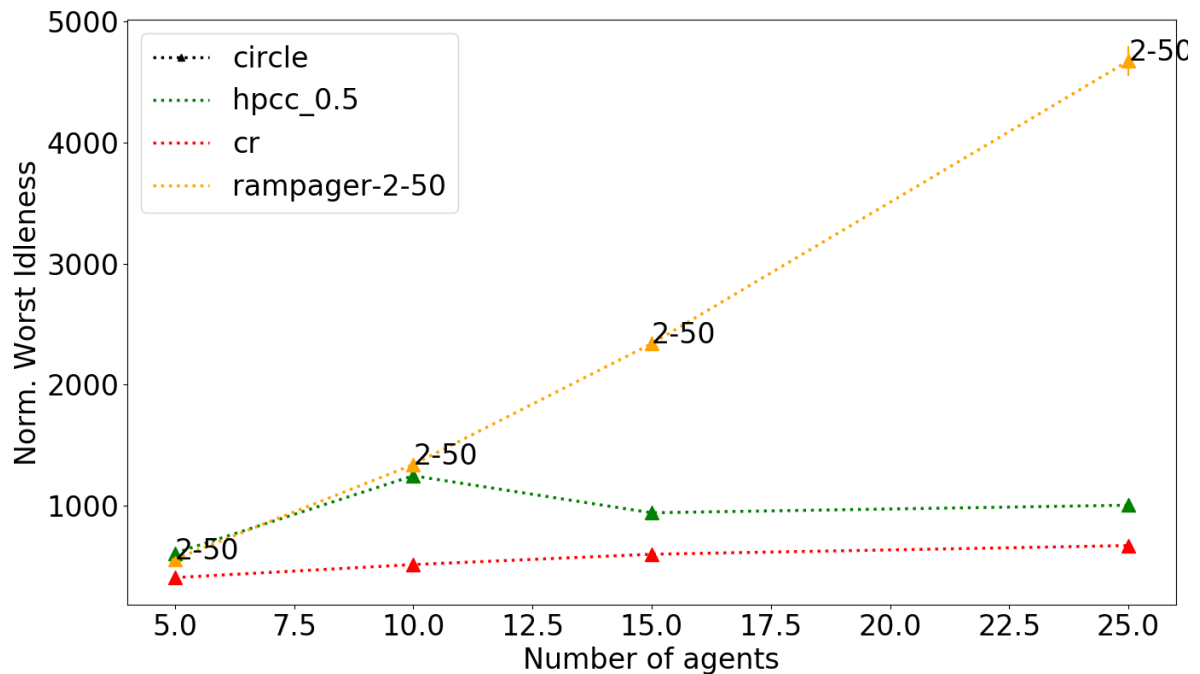
Fig. 5.19 Normalised WI of RAMPAGER 2-50 averaged over 100 execution w.r.t. the number of agents on Circle.
