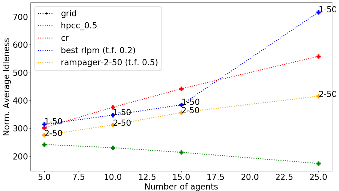
Fig. 5.16 Normalised Iav, averaged over 100 execution, of the RAMPAGER 2-50 and the best variant of RLPM w.r.t. the number of agents on Grid.
