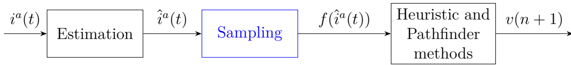
Fig. 6.2 Random Heuristic Pathfinder Idleness Estimator (RHPIE) strategy, with v(n) being the n th visited node.
