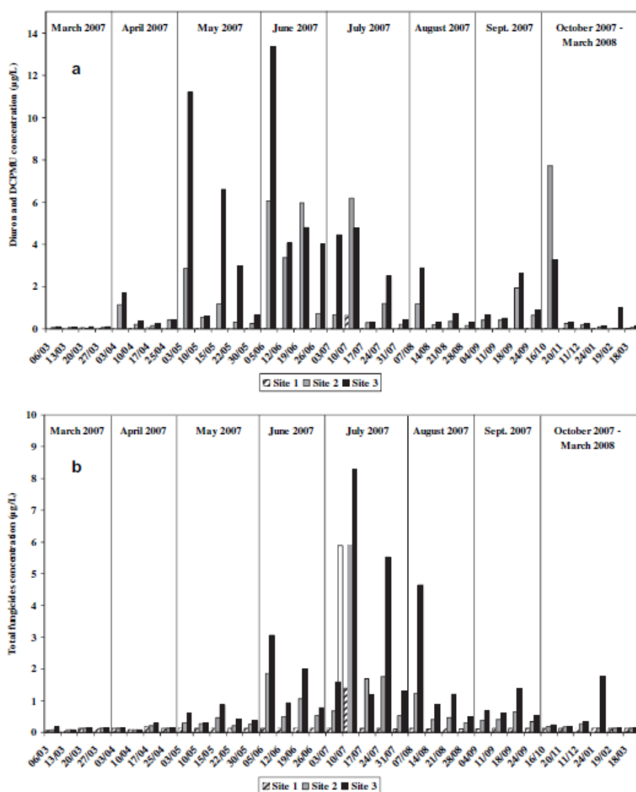
Figure 4 : Pesticides concentrations (in µg/L) along the Morcilles stream from March 2007 to March 2008; a: diuron and DCPME; b: total fungicide (sum of the five fungicides monitored).(Rabiet et al. 2010)
