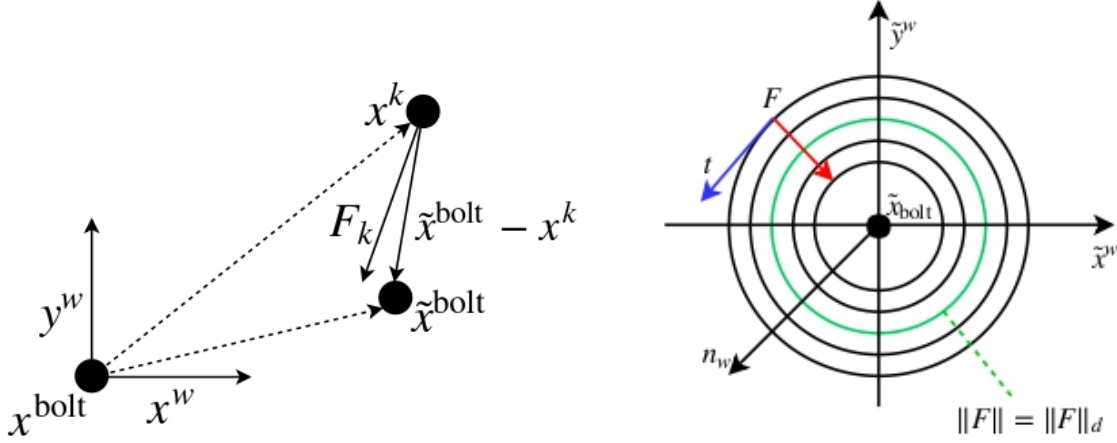
Fig. 3.3. Vectors \mathbf{F}^{(k)} and \mathbf{x}_{\text{bolt}} - \mathbf{x}^{(k)} at instant k used for the calculation of the force field characteristic FFC. \mathbf{x}^{(0)} is the current tool position at k = 0 in the world reference system. It is the origin of the wall reference system where the bolt position \mathbf{x}_{\text{bolt}} is regressed.
