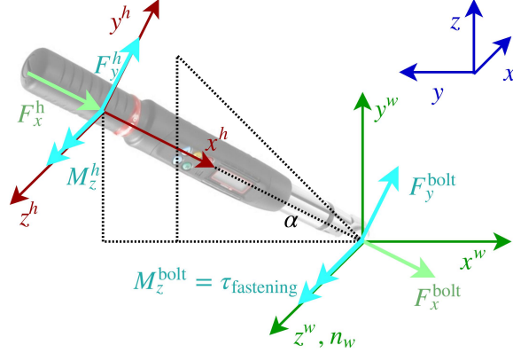
Fig. 3.1. Free body diagram of the wrench tool: world (dark blue), wall (w, dark green) and hand (h, red) reference systems; torques and forces which are dependent of each other are colored the same: F_x^h = -F_x^{\text{bolt}} , F_y^h = -F_y^{\text{bolt}} , M_z^h = -\tau_{\text{fastening}} - L_{\text{wrench}}F_y^{\text{bolt}} , ( \tau_{\text{fastening}} = -M_z^h + L_{\text{wrench}}F_y^h )
