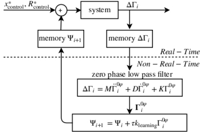
Fig. 3.2. The trajectory learning control diagram: The system is unknown and outlines the robot's dynamics and its interaction with the environment. Its input are the desired trajectories for the end-effector x^d and R^d and its output is the measured wrench error \Delta\Gamma .
