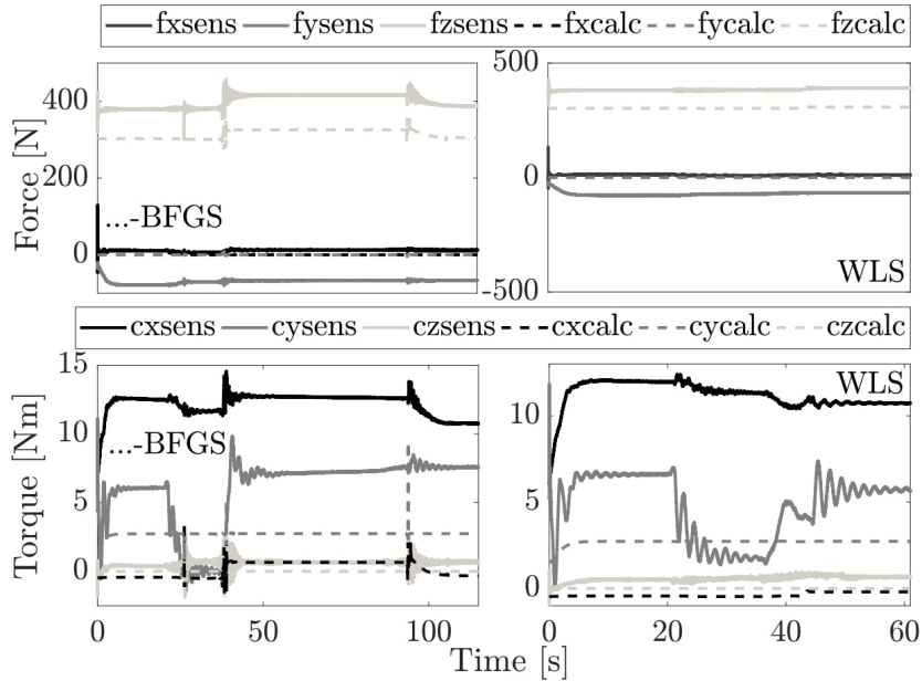
Fig. 5.32. Exp. 1 , comparison of the ground reaction forces (top) and torques (bottom) of the left foot between LexLSAug2BFGS (left column) and WLS (right column), measured ( sens ) and computed ( calc ). They are of similar magnitude.
