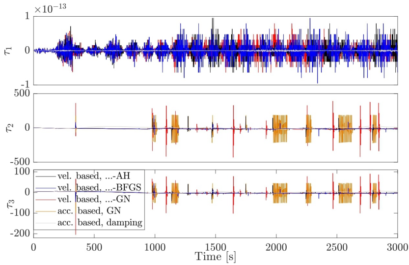
Fig. 5.15. Example 3, joint torques. The acc. and vel. based GN algorithm leads to instabilities in the joint torques of joint 2 and 3. LexLSAug2AH and LexLSAug2BFGS are stable.
