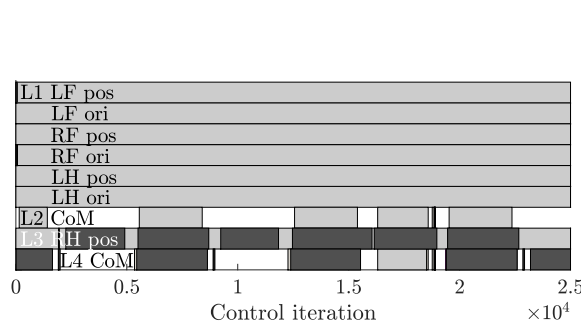
Fig. 4.22. T20, map of activity (light gray) and Newton's method (dark gray) for LexLSAug2BFGS .
