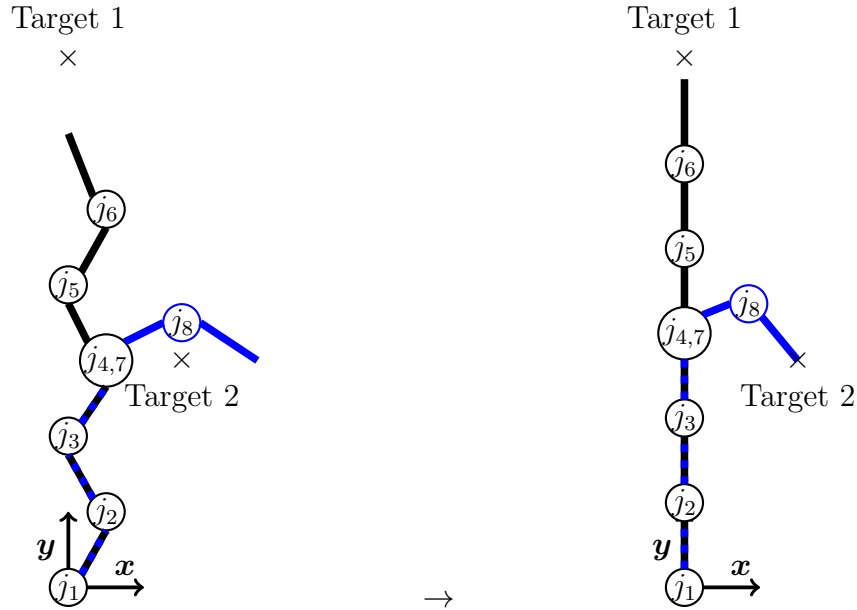
Fig. B.1. Left: the robot in initial configuration. The level 1 target is out of reach (black kinematic chain), the level 2 target is in reach (blue and dashed blue kinematic chain). Right: the robot in converged configuration. The black kinematic chain is fully dedicated to the level 1 task. The full rank augmentation \mathbf{I}_1^*(\mathbf{j} \setminus j_7, j_8) does not influence the joints j_7 and j_8 which is the only one left for controlling the level 2 end-effector.
