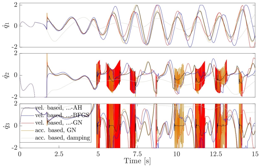
Fig. 5.16. Example 3, joint velocities. The acc. and vel. based GN algorithm leads to instabilities in the joint torques of joint 2 and 3. They occur whenever the kinematic subchain consisting of link 2 and link 3 is close to kinematic singularity. LexLSAug2AH and LexLSAug2BFGS are stable. Damping in the acceleration domain is stable but leads to the mentioned overshooting behaviour.
