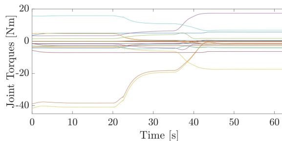
Fig. 5.31. Exp. 1, WLS, joint torques.
