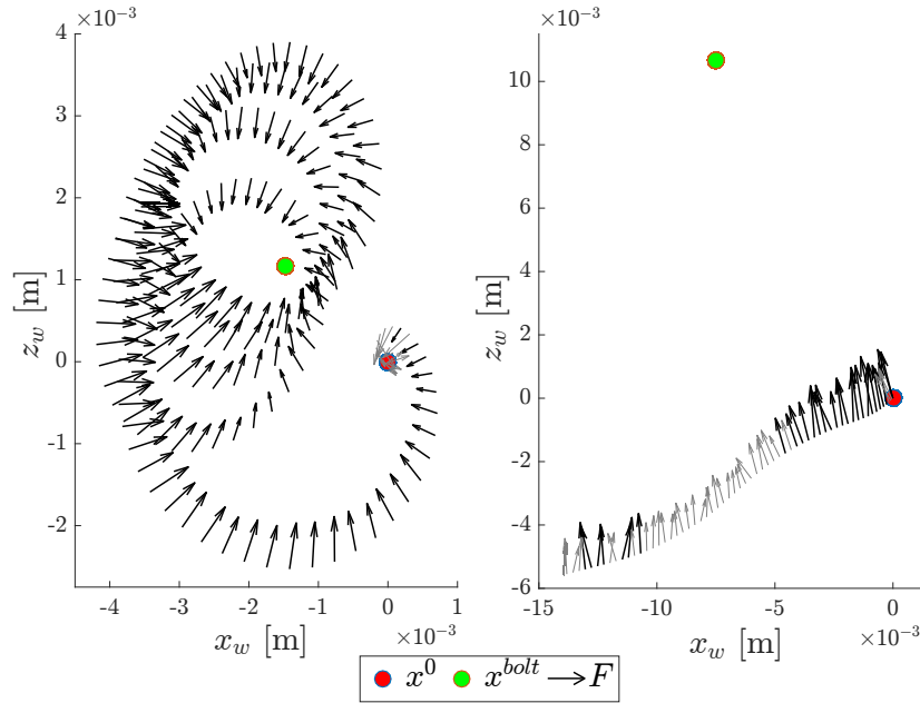
Fig. 3.6. Sensed force field for inserted (left) and non-inserted tool (right); forces with \|\mathbf{F}\| < 1 \text{ N} are coloured gray.
