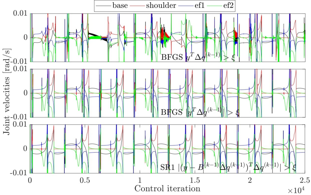
Fig. 4.5. Joint velocities for test 1. The upper graph shows the unstable behaviour for positive definite BFGS updates of the approximation of the second order derivatives. This is in contrast to the indefinite BFGS and SR1 updates which both result in stable joint velocities.
