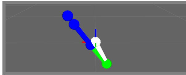
Fig. 5.17. Example 3. The robot managed to come to the target as close as possible ( LexLSAug2BFGS ). However, some swaying motion remains due to the freely swinging joint 1 (white ball) with zero commanded torque. Note how the kinematic subchain of the green and blue link is in kinematic singularity.
