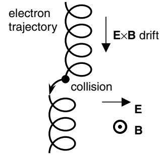
Figure 1. Electron drift in an E \times B configuration.
