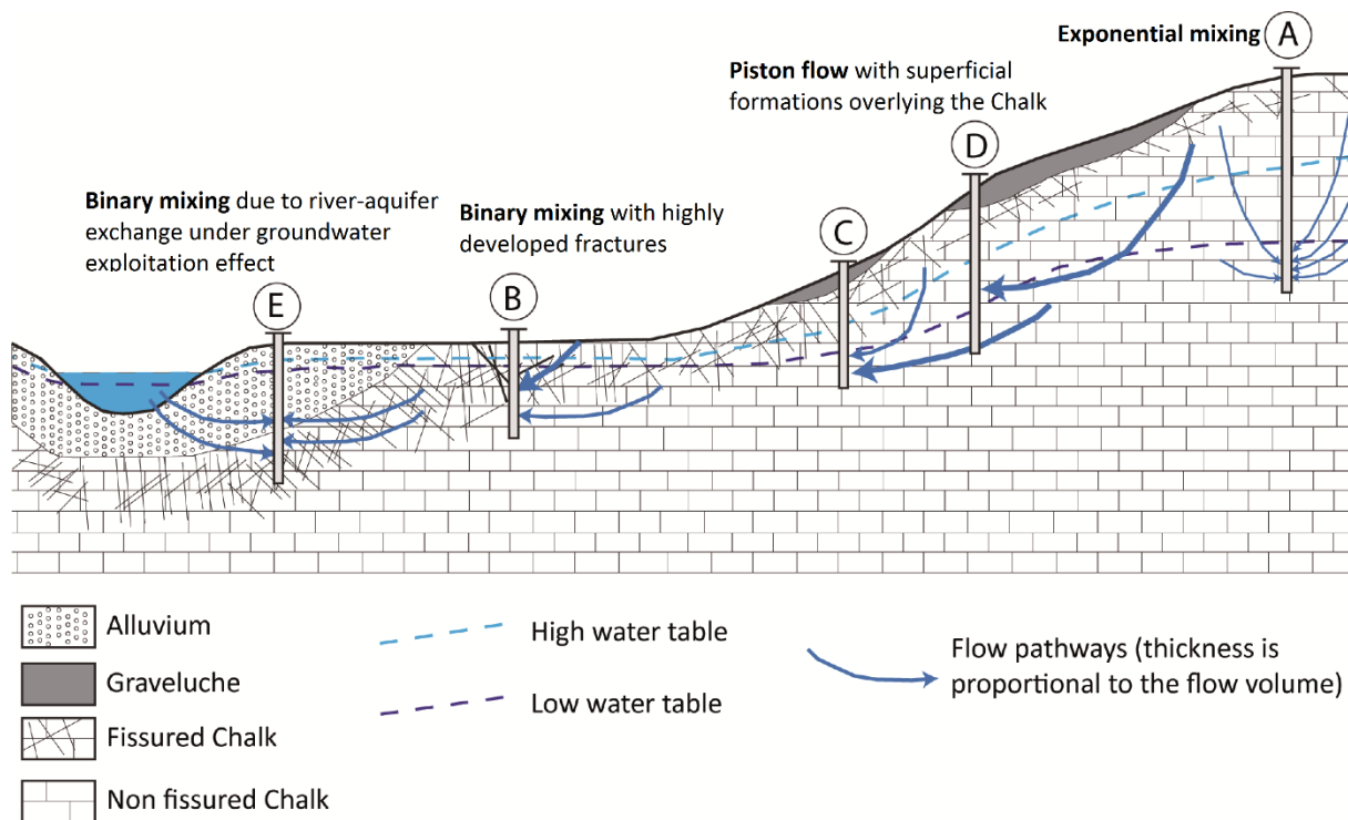
Figure III-25 : Schematized hydrogeological functioning of unconfined Chalk aquifers
