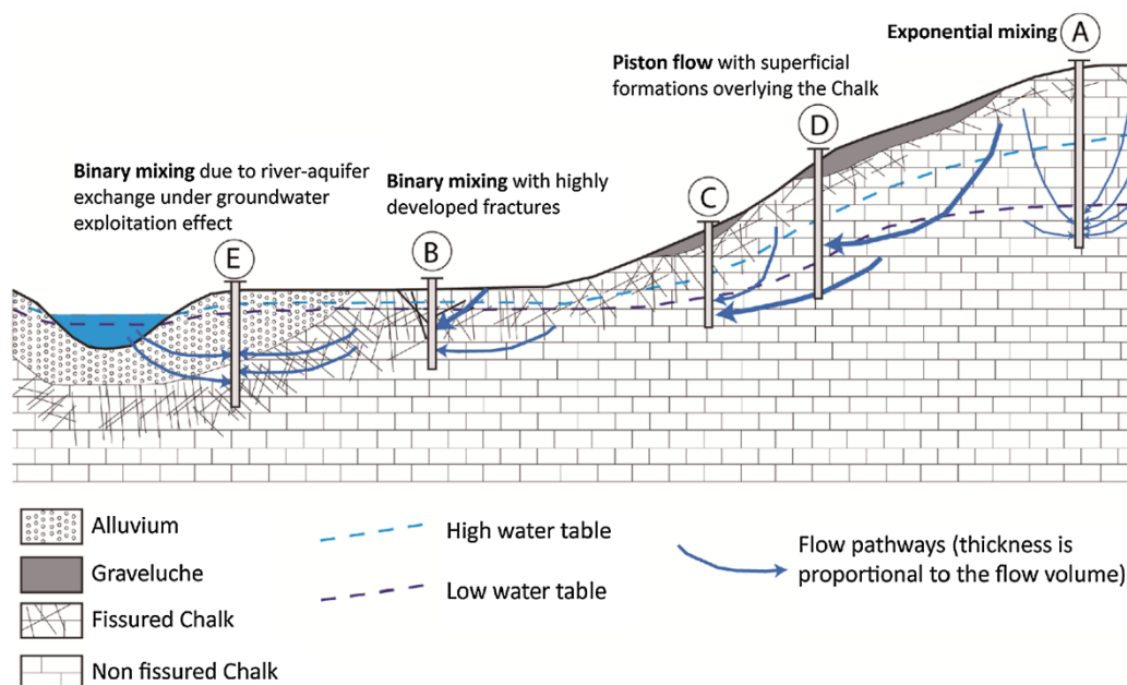
Fig. 7. Schematized hydrogeological functioning of unconfined Chalk aquifers.
