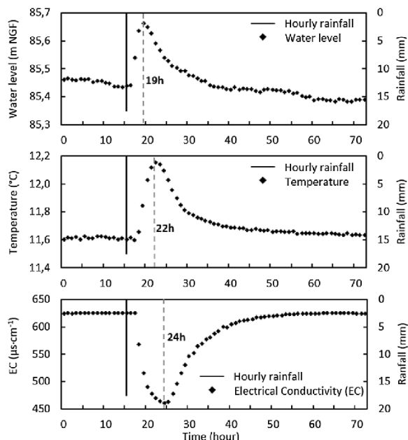
Fig. 3. Response of groundwater level (hourly data), temperature (hourly data) and EC (hourly data) to a rainfall event (17 mm at the 15th hour) at FAP from 5 July to 8 July 2018.
