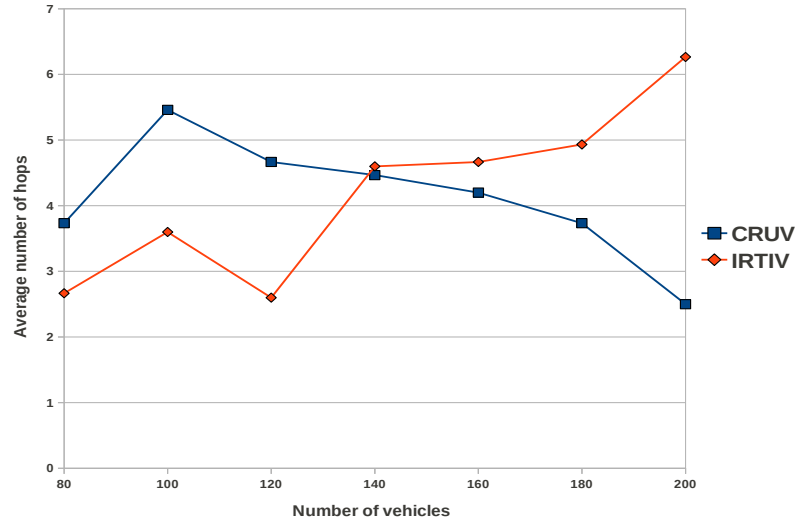
Figure 4.13: Average number of hops vs. vehicle density
