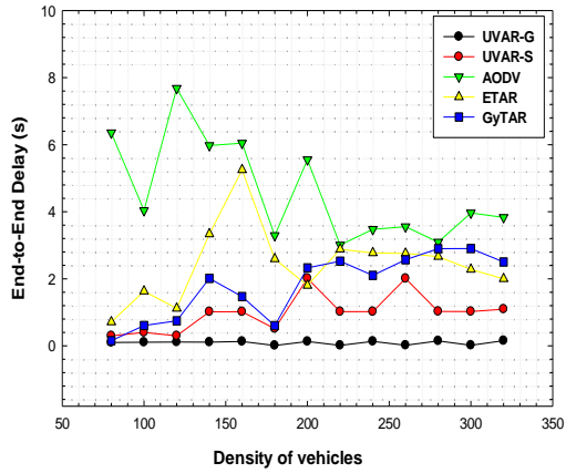
(a) EED vs. Density of vehicles (UAVs=16).
