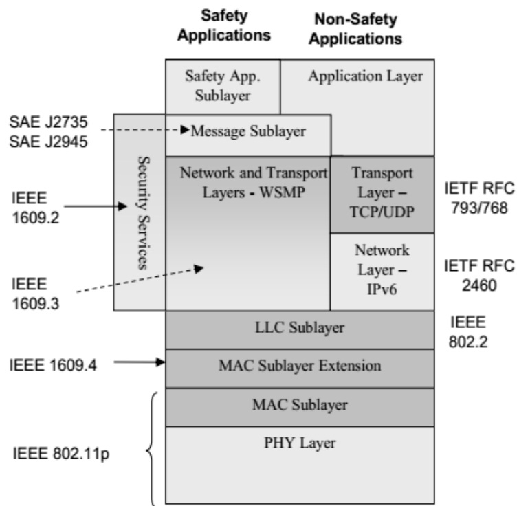
Figure 2.5: Wave architecture [1, 2].
