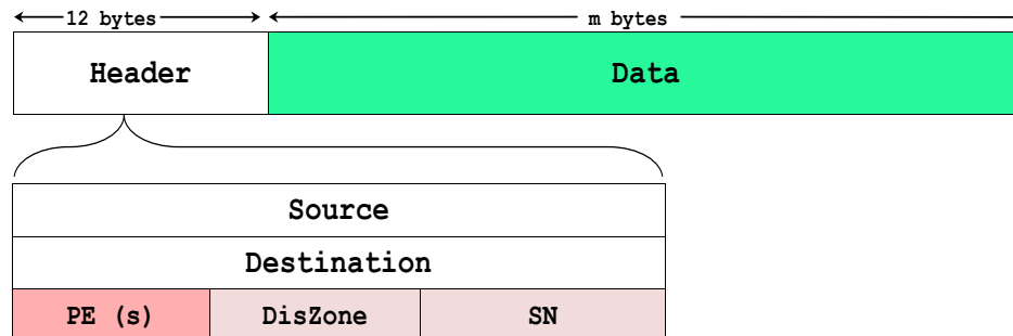
Figure 6.12: Data packet Format.
