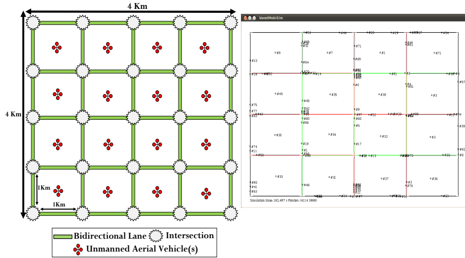
Figure 5.10: Network topology.
