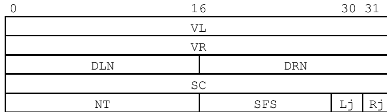
Figure 4.3: Additional fields in the Hello packets.
