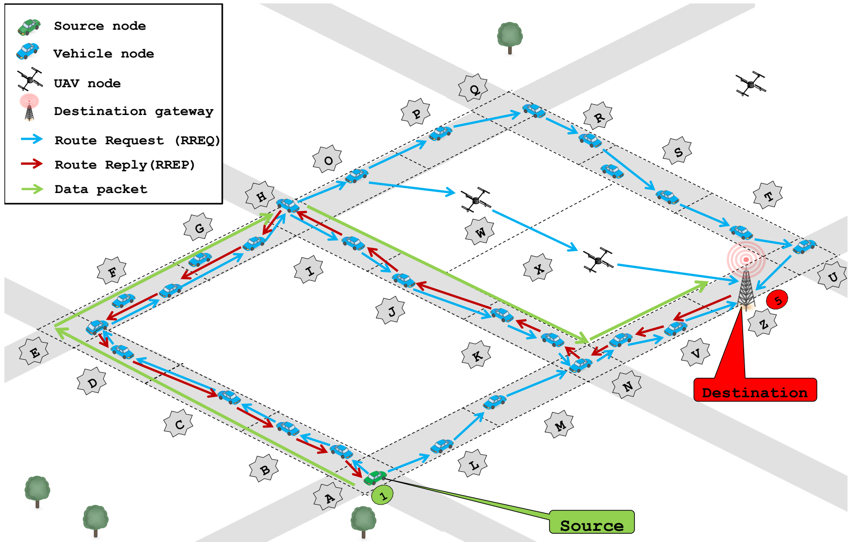
Figure 6.5: Principle of functioning of the discovery phase.
