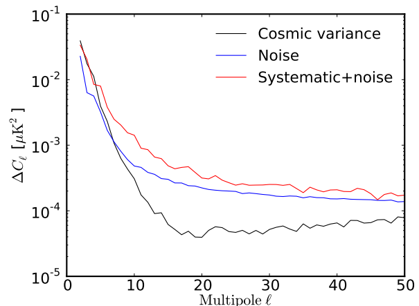
Figure 9.2: Variance of the 100×143 EE cross-power spectrum for simulations, including instrumental noise and noise plus systematic effects, compared to cosmic variance.
