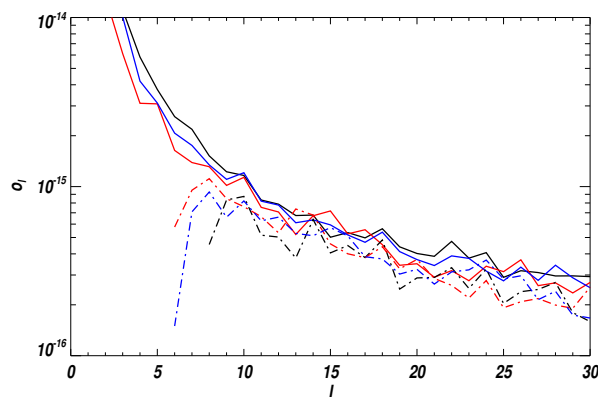
Figure 5.7: The offset functions \sigma_\ell^{A \times B} of the oHL likelihood for the Planck-HFI×Planck-143 B-modes cross-spectra (solid) and the E-modes cross-spectra (dashed). The different colors refers to the different fiducial models used in the simulations: black is the early reionization scenario without tensor modes (model 1), red is the late reionization scenario with tensors (model 2) and blue is the Planck 2015 best fit with r=0.1 .
