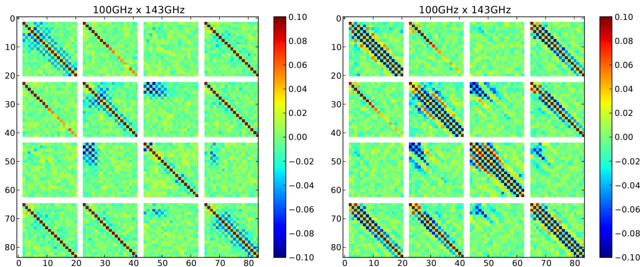
Figure 5.3: Correlation matrix for the cross-power spectra 100x143 with two different sky coverage: 80% (left) and 50% (right). Each block corresponds to TT , EE , BB , TE spectra respectively. \ell=0 and \ell=1 are not defined and set to zero.
