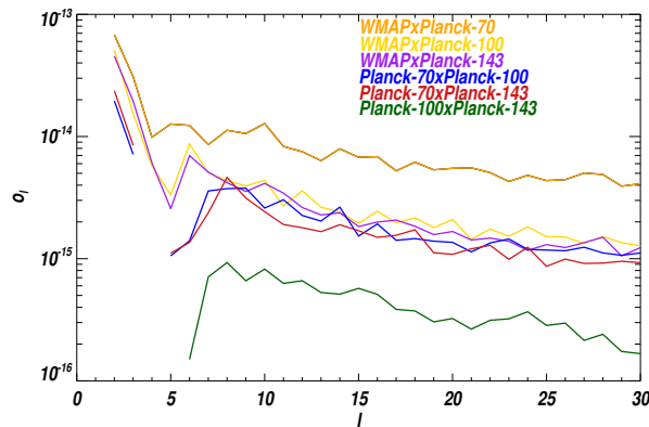
Figure 5.6: The offset functions \sigma_\ell^{A \times B} of the oHL likelihood for the E-modes cross-spectra and for the six different combinations of noise levels.
