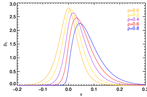
Figure 5.1: Examples of the full-sky cross-spectra distributions p_N^{A \times B}(x \equiv \hat{C}_\ell^{A \times B}) for N=5 modes ( \ell=2 ) with \sigma_A \sigma_B=0.1 and varying the degree of correlation (cf. Eq. 5.2).
