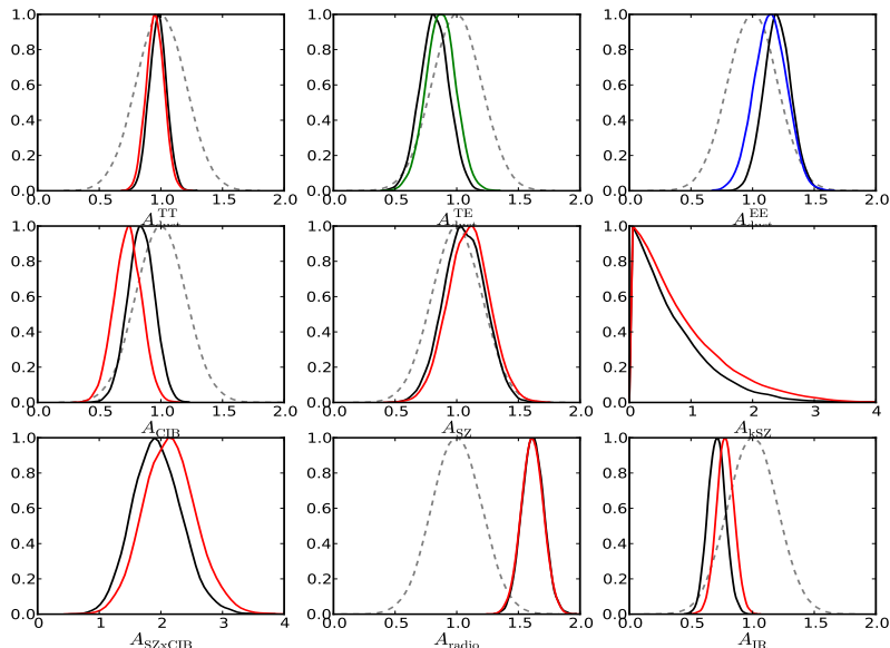
Figure 7.3: Astrophysical foreground amplitude posterior distributions for the HiLLiPOP likelihoods: HillipopTXE (black), HillipopT (red), HillipopE (blue) and HillipopX (green). Priors are plotted in grey dashed line.
