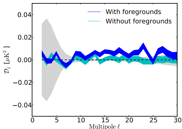
Figure 9.1: Bias in the 100×143 cross-power spectrum computed from simulations, including instrumental noise and systematic effects, with or without foregrounds (dark blue and light blue), compared to the cosmic variance level (in grey).
