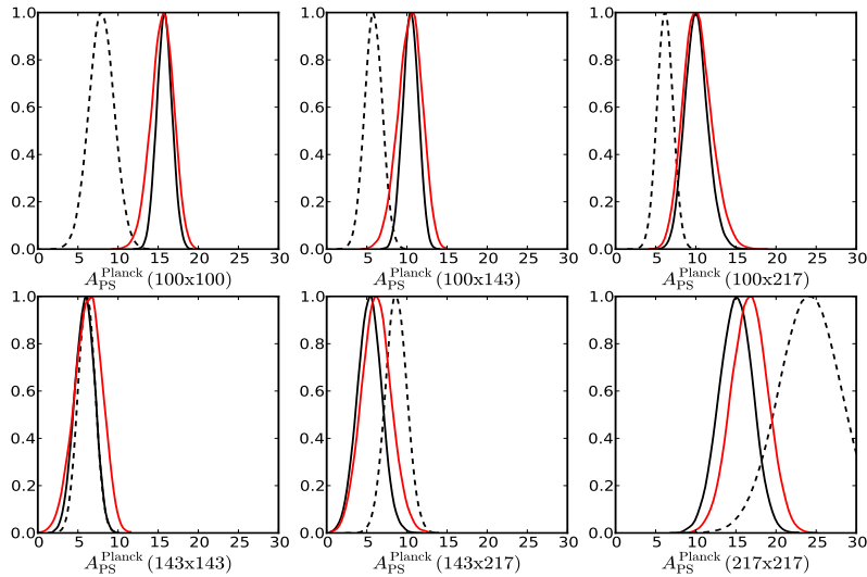
Figure 7.4: Posterior distributions for the six point sources amplitudes for HillipopTXE ( black line ) and HillipopT ( red line ) compared to model prediction ( dashed line ). Units: \text{Jy}^2 \cdot \text{sr}^{-1} ( \nu I_\nu = cte ).
