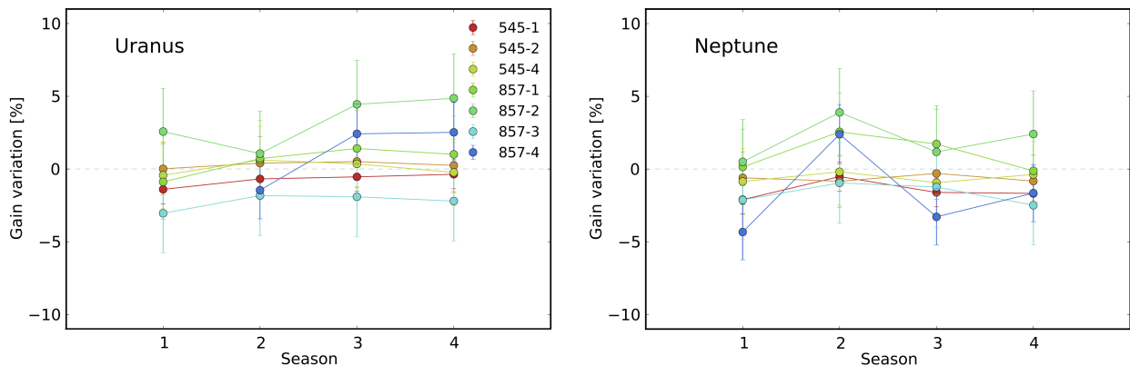
Figure 3.2: Dispersion of the planet-derived calibration factor per season around the planet calibration estimates for Uranus (left) and Neptune (right).
