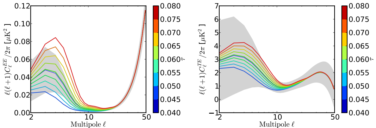
Figure 9.3: EE and TE power spectra for various \tau values ranging from 0.04 to 0.08. The ionization fraction is modelled using a redshift-symmetric tanh function with \delta z = 0.5 . Grey bands represent the cosmic variance (full-sky) associated with the \tau = 0.06 model.
