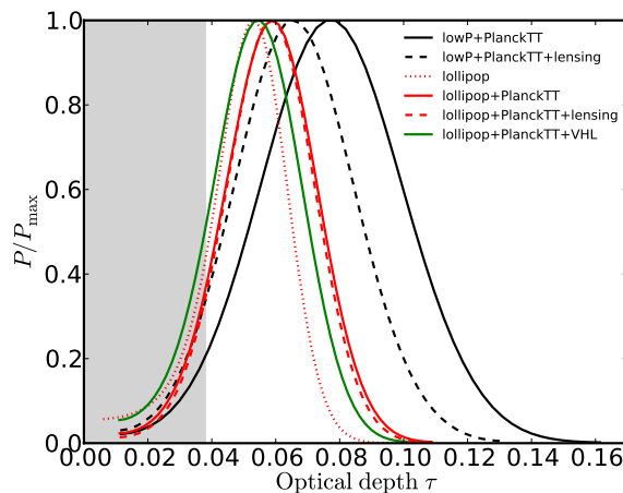
Figure 9.5: Posterior distribution for \tau from the various combinations of Planck data. The grey band shows the lower limit on \tau from the Gunn-Peterson effect.
