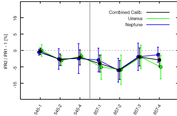
Figure 3.3: Comparison of the 2015 Planck release calibration to the 2013 release. We show the relative difference in percent per bolometer for Uranus (green), Neptune (blue), and both calibrators combined (black).
