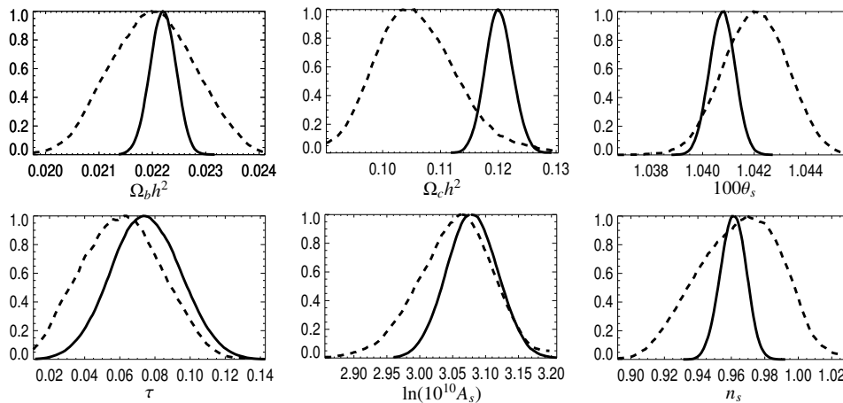
Figure 8.7: Posterior distributions of the cosmological parameters obtained by sampling the Hillipop (solid line) and ACT+SPT (dashed) likelihoods independently. A prior of \tau=0.07\pm 0.02 is used in both cases. For clarity, we only show the cosmological parameters, but all nuisances are sampled.
