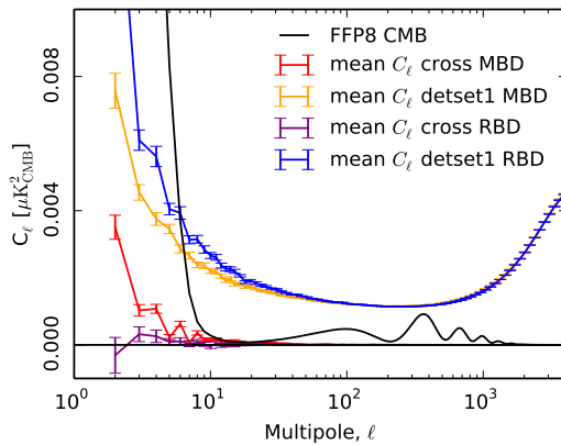
Figure 3.17: Average EE spectra obtained from 100 simulations of detector-set noise maps. The maps were produced using either the full-mission baseline destriping (MBD) or the destriping run on each subset independently (run baseline destriping or RBD). Both the increased low- \ell noise in the RBD case and the increased cross-spectrum noise bias in the MBD case are apparent.
