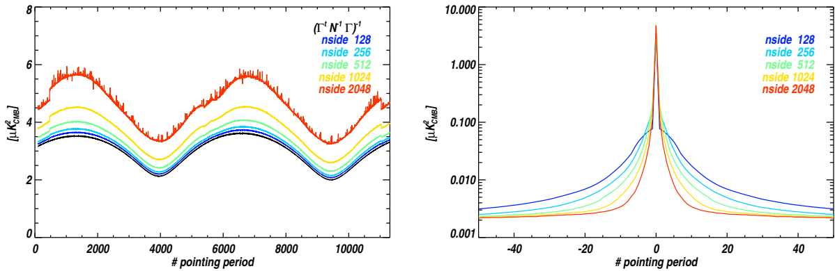
Figure 1.6: Left : Diagonal of the offset covariance matrix for various internal sky resolutions used for the offset recovery. Black line shows the first term of Eq. 1.25. Right : Offset covariance matrix profiles centered on the diagonal showing the ring-to-ring covariance for various internal sky resolution.
