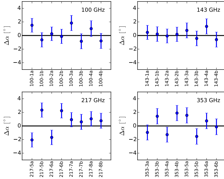
Figure 3.20: Estimated angular offset from comparison of the single bolometer, single detector maps with the IRAM Crab nebula maps, combining the first four surveys.
