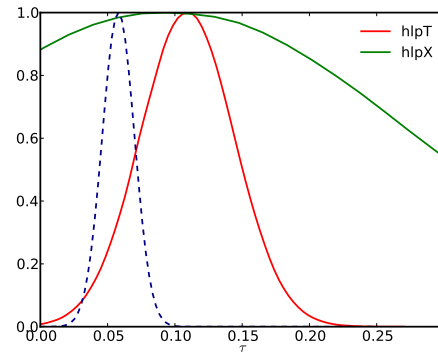
Figure 7.6: Posterior distribution for the reionization optical depth \tau for HillipopT ( red line ) and HillipopX ( green line ) compared to the prior from Planck Collaboration Int. XLVII (2016) used throughout this analysis ( dashed darkblue line ).
