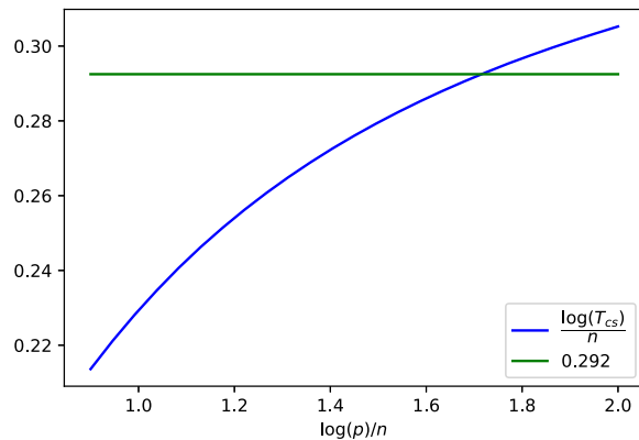
Figure 1.1 – Solving SVP using cylindrical sieving for n -dimensional prime volume lattices of the volume 2^{cn} . p denotes the volume of the lattice (i.e., c = \frac{\log(p)}{n} ), the blue line represents the complexity of the cylindrical sieving, the green line represents the complexity of the current fastest heuristic algorithm for solving SVP [BDGL16].
