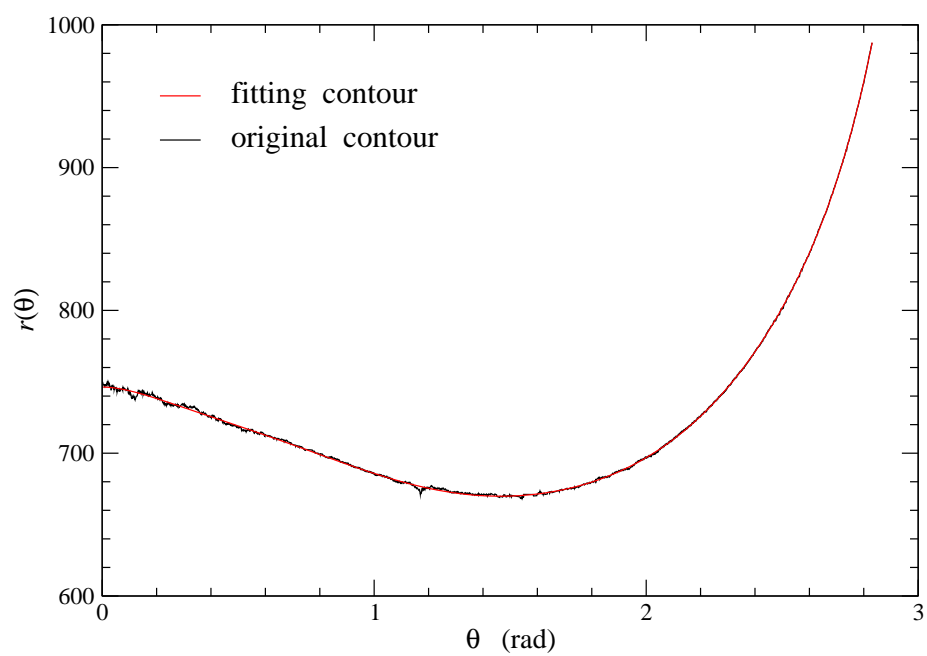
Figure 4.7: Half of the pendent droplet profile before and after fitted by Least Squares Fitting-Polynomial
