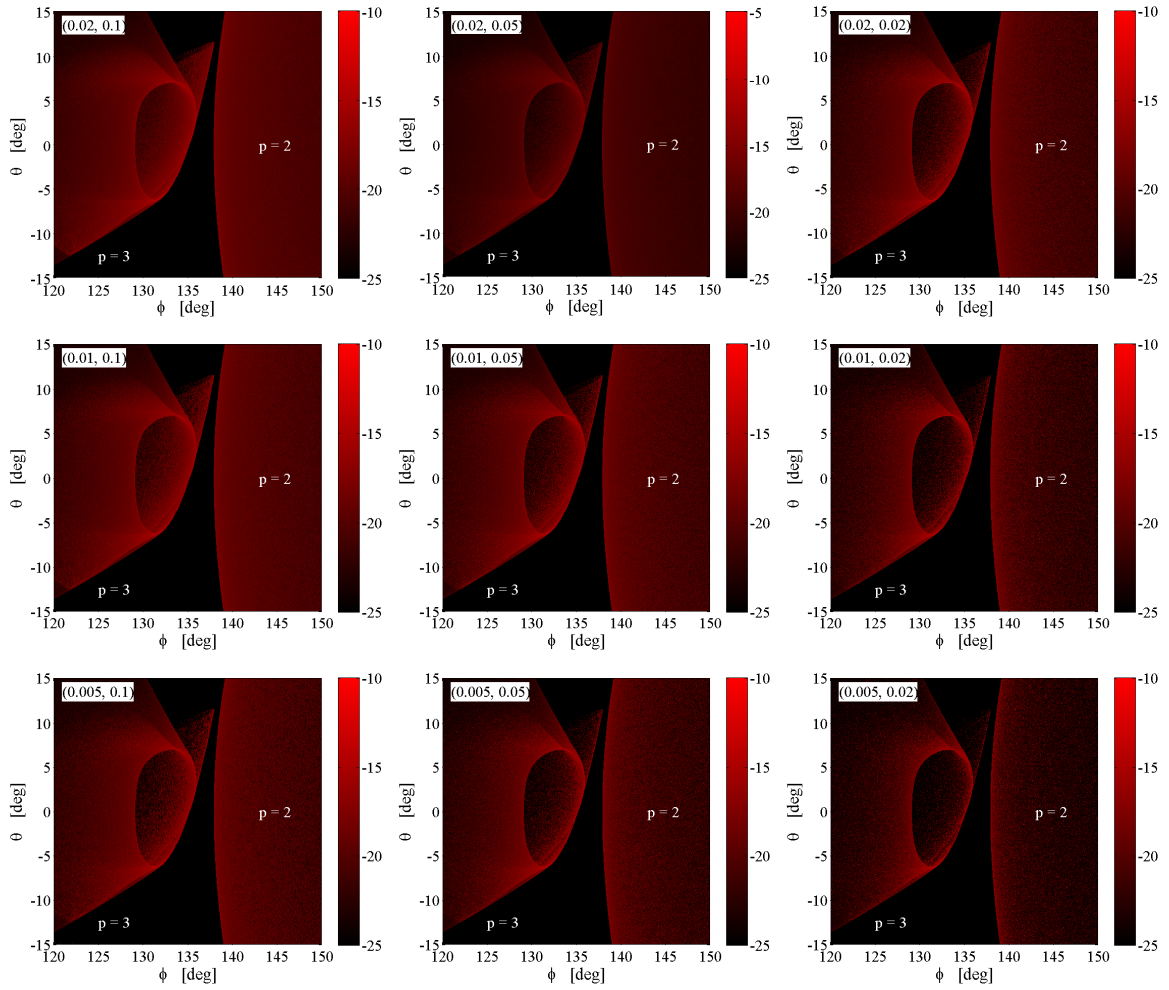
Figure 5.13: Same as Fig. 5.11 but for the droplet \mathbf{d} with R_e = 671.16 \mu\text{m} and H = 1707.68 \mu\text{m}
