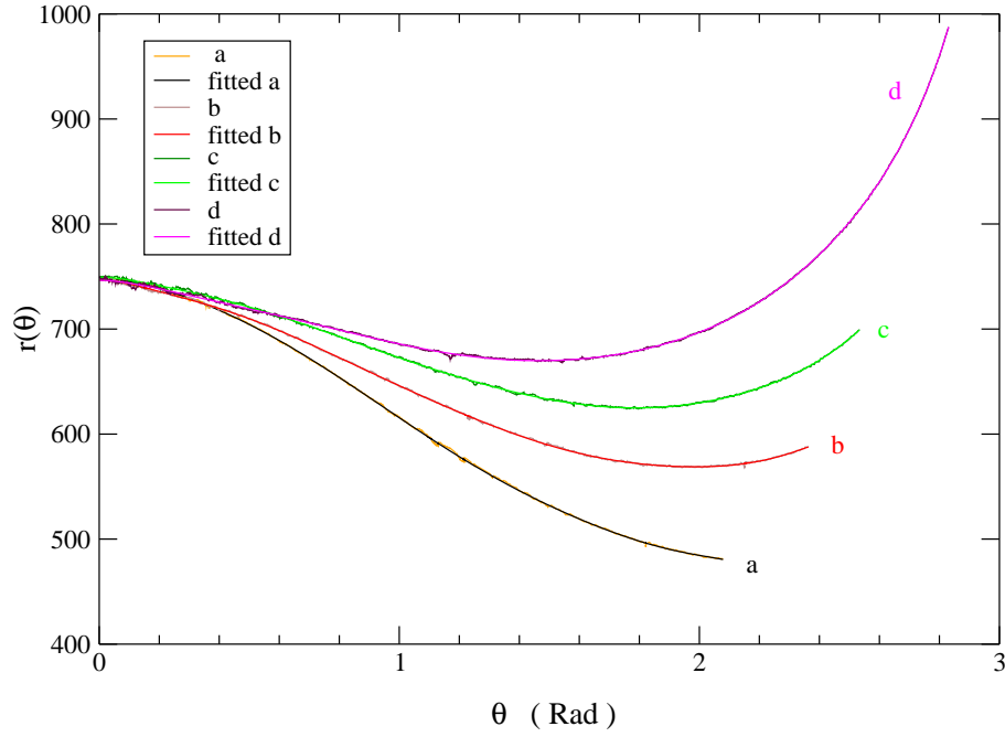
Figure 4.9: Profiles of droplets in polar coordinate system
