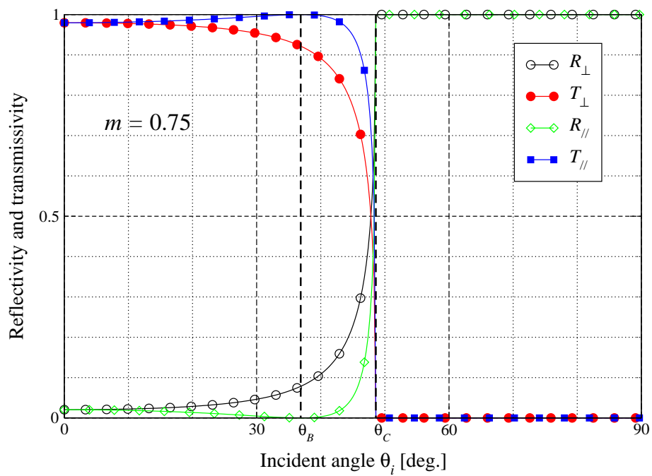
Figure 2.5: Reflectivity and transmissivity as function of incident angle \theta_i for two relative relative refractive indice.
