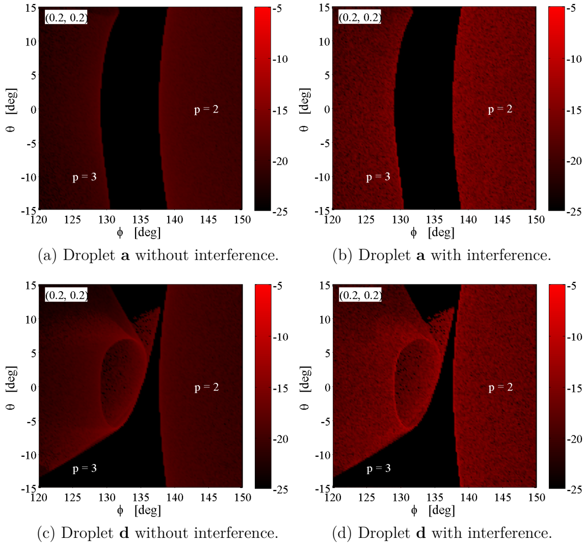
Figure 5.2: Scattering patterns of a pendent droplet near rainbow angles simulated by SVCRM with the parameters in Tab. 5.1 and the number of emitted photons N = 4 \times 10^7 .
