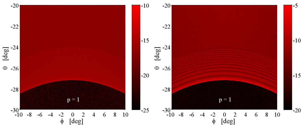
Figure 5.26: Scattering patterns without interference (left) and with interference (right) in the forward direction of the droplet \mathbf{d} . The detection region is \phi \in [-10^\circ, 10^\circ] and \theta \in [-30^\circ, -20^\circ] .
