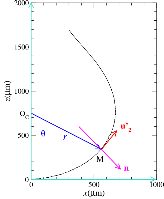
Figure 4.11: Half of the pendent droplet profile in polar coordinates
