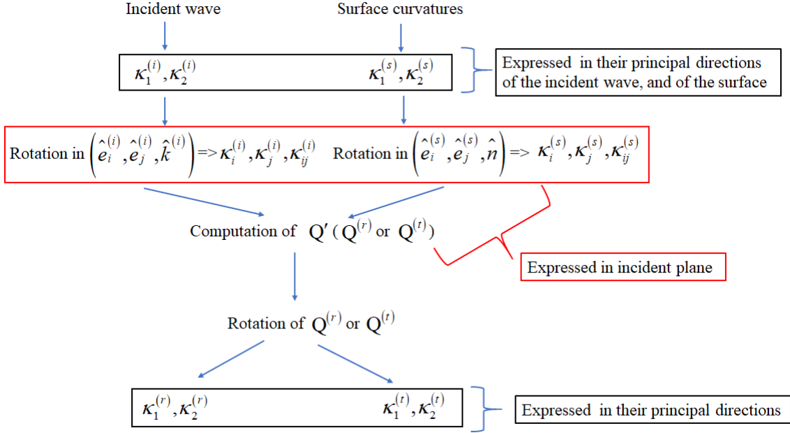
Figure 3.5: Conversion of matrices between different bases
