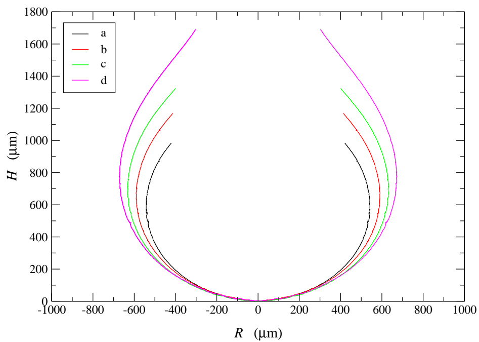
Figure 4.8: Contours of shaped droplets in Cartesian coordinate system
