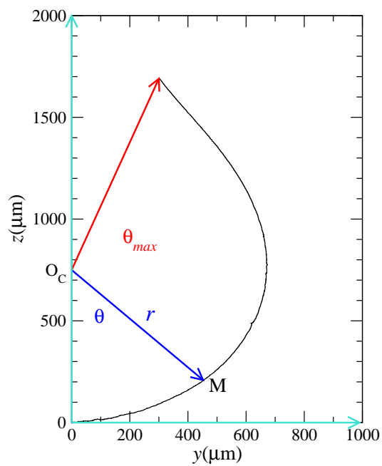
Figure 4.6: Half of the pendent droplet profile in Cartesian coordinate systems.
