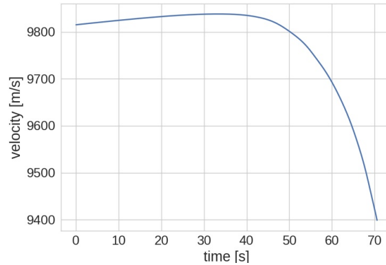
Figure B.3: Time evolution of the Upper Stage velocity before breakup
