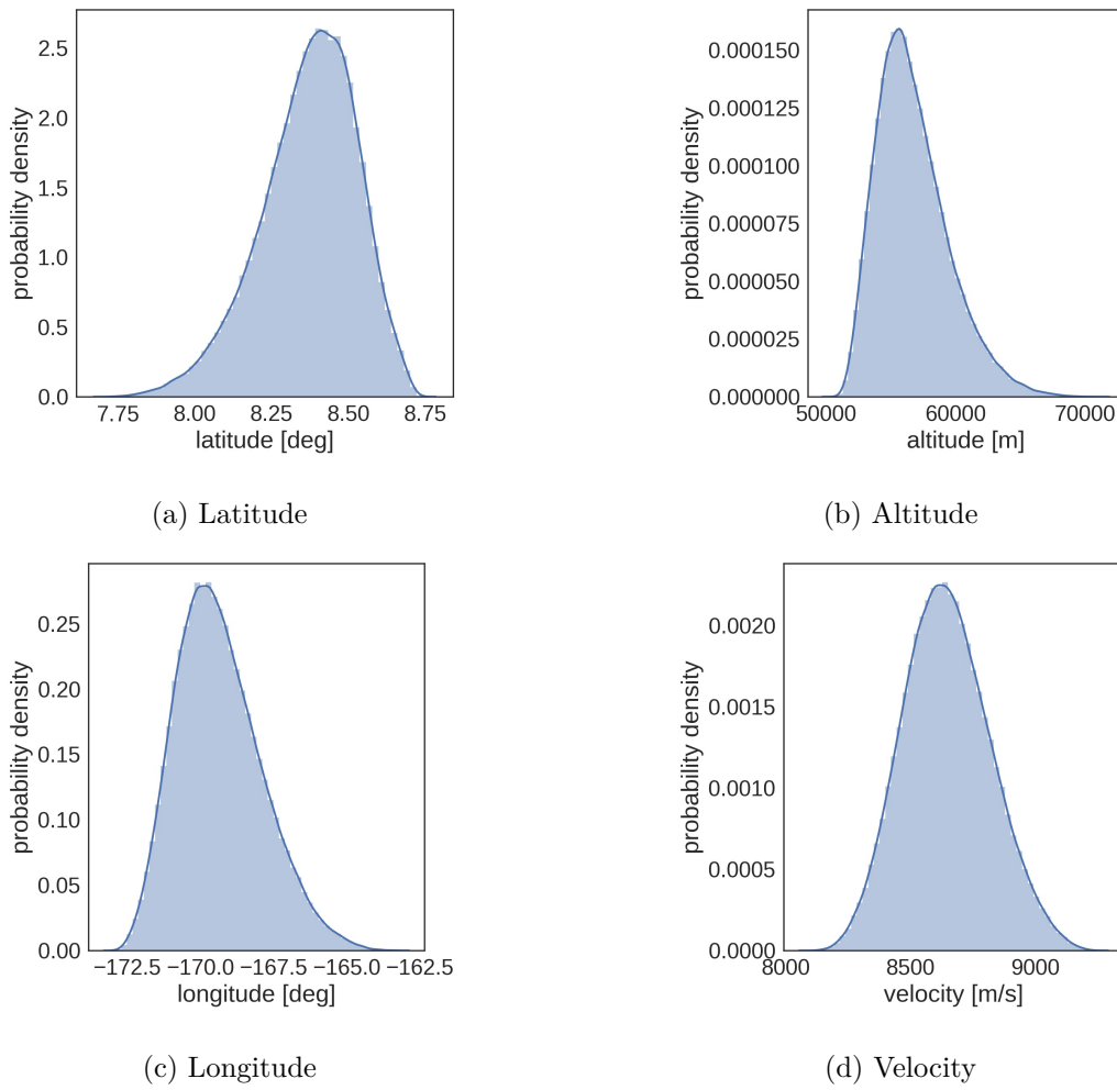
Figure 5.6: Flight conditions distributions at t_{end}
