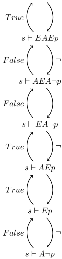
Figure 3.22. Answer's scheme, i.e. sequence of sessions of the running example of the main procedures for the Naive parallel algorithm for CTL* model checking.
