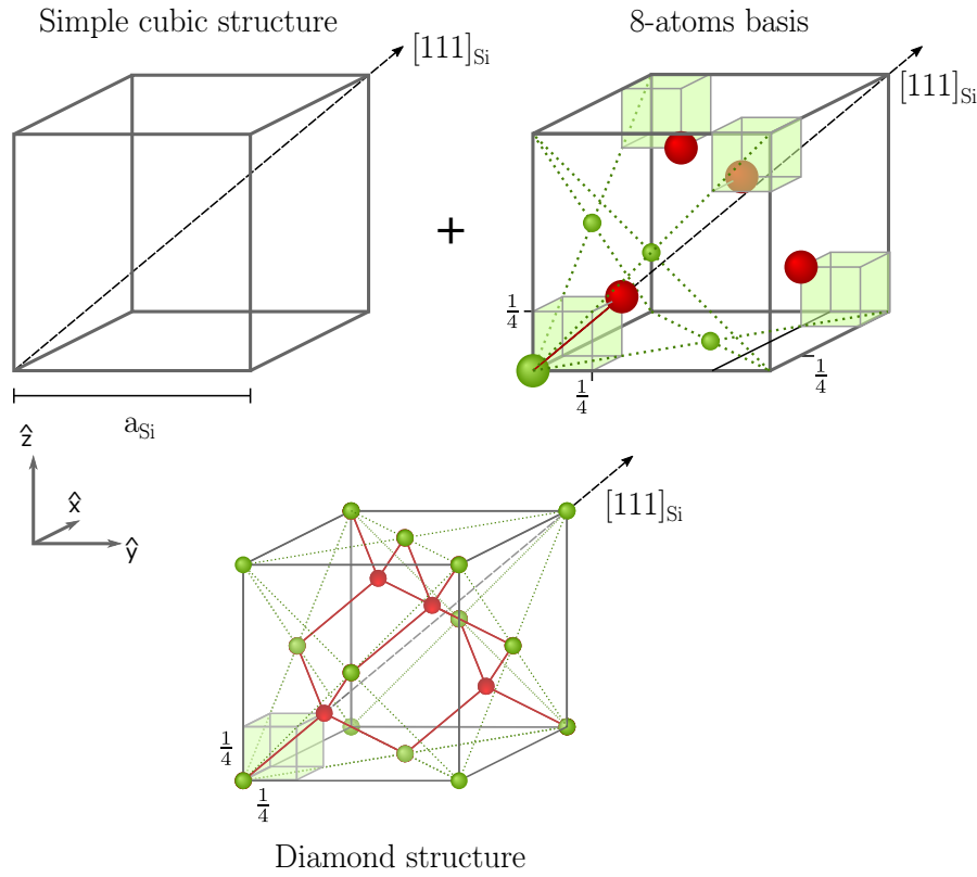
FIGURE 5.3: Unit cell of the monoatomic diamond lattice (bottom), depicted as a simple cubic Bravais lattice with 8-atoms basis (top).
