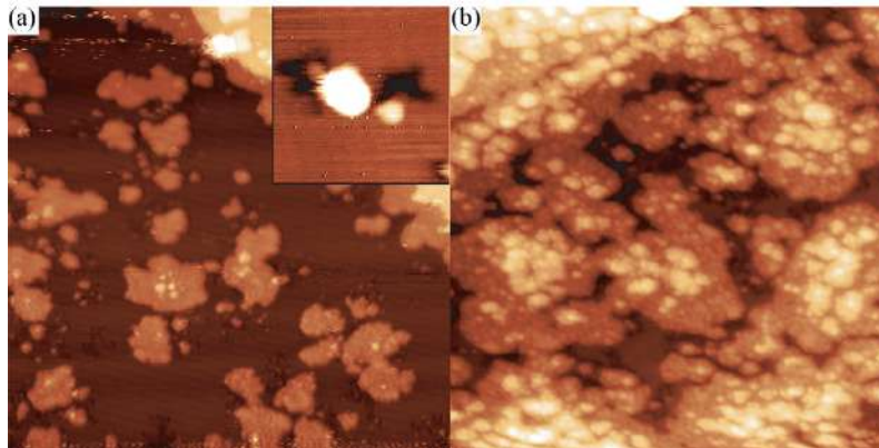
FIGURE 1.14: STM images showing Si growth on Ag(111) at 200 K for increasing Si coverage. (a) 86 \times 86 nm 2 and 21 \times 21 nm 2 (inset); (b) 43 \times 43 nm 2 . Figures reproduced from ref. [78].
