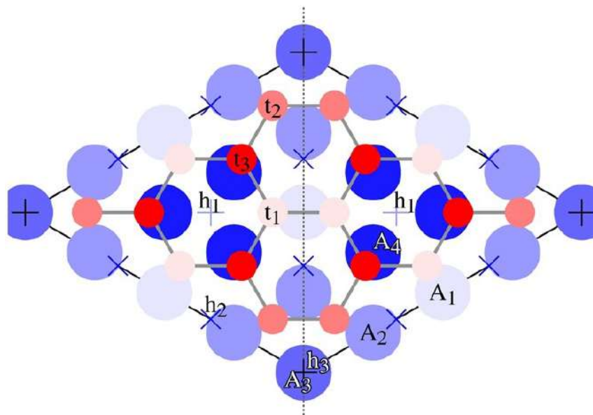
FIGURE 6.18: Adsorption sites for Si atoms on the ( 4 \times 4 ) reconstruction (top view). Labels are defined in the text. Bluish disks are Ag atoms of the outermost layer, while reddish ones are Si atoms of the surface reconstruction. The black line represents the ( 4 \times 4 ) unit cell. The system has C_3 symmetry around the sites labeled as h_1 and h_3 . To simplify the notation I assume a mirror symmetry for the plane vertical to the surface and passing through the dotted line. There are four inequivalent Ag sites labeled as A_1 , A_2 , A_3 , A_4 . Using the same notation, there are three inequivalent Si sites: t_1 , t_2 and t_3 . The crosses indicate the centers of the Si hexagons formed in the reconstruction and they are labeled as h_1 , h_2 , and h_3 .
