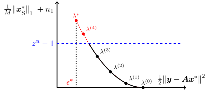
Figure 3. Set of optimal solutions \left(\frac{1}{2}\|\mathbf{y} - \mathbf{A}\mathbf{x}^*\|_2^2, \frac{1}{M}\|\mathbf{x}_S^*\|_1 + n_1\right) as a function of \lambda , and illustration of a stopping criterion of the homotopy algorithm for \mathcal{Q}_{1/2} . The algorithm can be stopped (and the corresponding node is pruned) as soon as \frac{1}{M}\|\mathbf{x}_S^*\|_1 + n_1 \geq z^u - 1 , where z^u is the cardinality of the best known feasible solution to \mathcal{P}_{0/2} at a given iteration of the branch-and-bound procedure.
