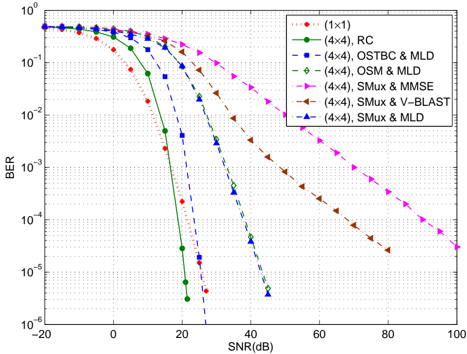
Figure 6.4 — Contrasting BER performance of different ST schemes for a (4 \times 4) MIMO FSO system. L = 5 Km, D_R = 200 mm. Uncoded OOK, thermal noise limited receiver.
