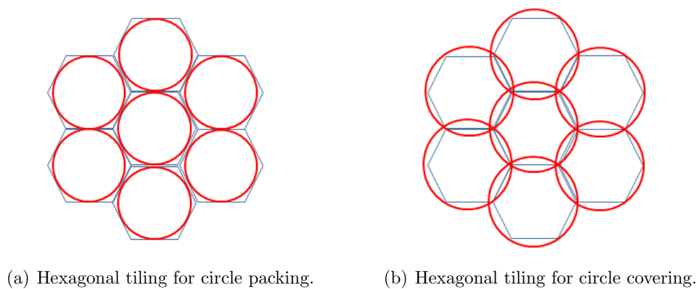
Figure 6.5: Hexagonal tilings.
