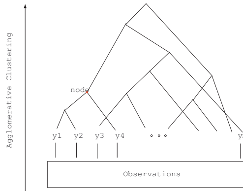
Figure 4.3: Agglomerative hierarchical clustering.
