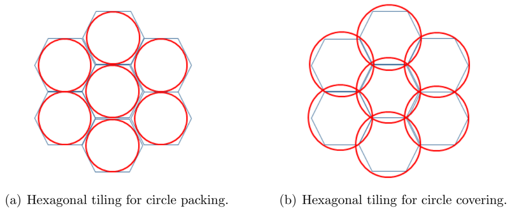
Figure 6.5: Hexagonal tilings.
