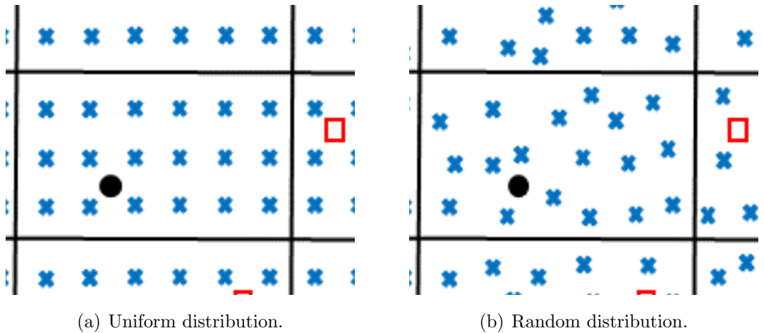
Figure 3.1: Illustration of fingerprinting configuration - \times designates reference positions, \square designates WiFi Access Points, and \bullet designates a MN.
