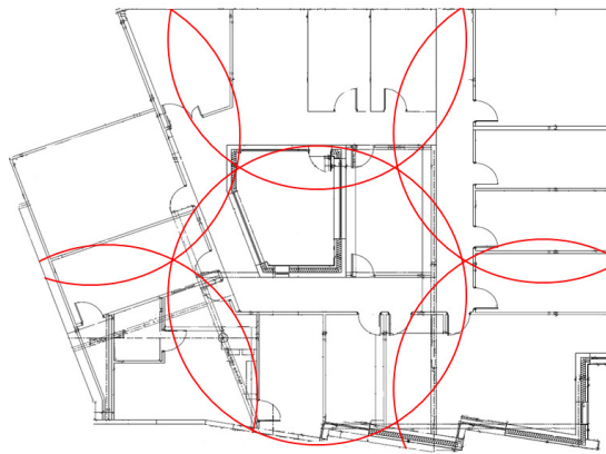
Figure 6.6: The Living Lab of the University of Troyes, France; A section area of 22m \times 25m covered by calculators with MNs of sensing range \delta = 6m .
