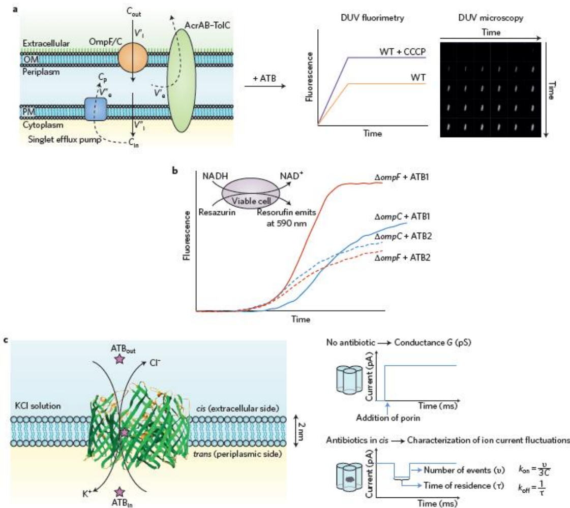
Figure 20: Methods for measuring intracellular accumulation and porin-mediated uptake of antibiotics. (a) DUV methods. Deep Ultraviolet (DUV) methods were developed for studying translocation of fluoroquinolones, which are intrinsically fluorescent, across the envelope of Gram-negative bacteria. Fluoroquinolone accumulation can be investigated in whole cells after cell lysis, or in intact cells by DUV microspectrofluorimetry or DUV fluorescent imaging (265). Fluoroquinolone (ATB, antibiotic) is added to intact cells at a concentration of C_{out} . The drug crosses the two membranes at the net rate V_i , which is a combination of V'_i and V''_i corresponding to the influx rates across OM through porins and IM, respectively. This influx is also balanced by two processes: (1) efflux into the external medium through the major transmembrane AcrAB–TolC pump at the rate V'_e ; and (2) efflux into the periplasm by several minor inner membrane ‘singlet’ pumps at the rate V''_e . In this model, C_{in} can be measured from the maximum fluorescence intensity. Using mutants and addition of CCCP (cyanide m-chlorophenyl hydrazone, an inhibitor of proton transport), the contribution of efflux by acrB or tolC has been determined (266, 267, 268). Similar approaches can be used to evaluate the role of specific OM porins on fluoroquinolone influx, assuming that drug diffusion across the inner membrane is not a limiting factor to reach maximal C_{in} . These approaches have shown that the drug resistance characteristics of E. aerogenes clinical
