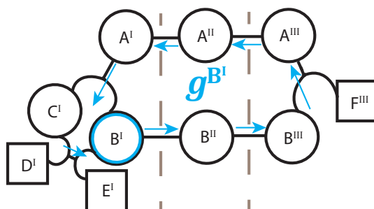
Figure 5.10: Autocatalytic transport with two different compartments I and III.
