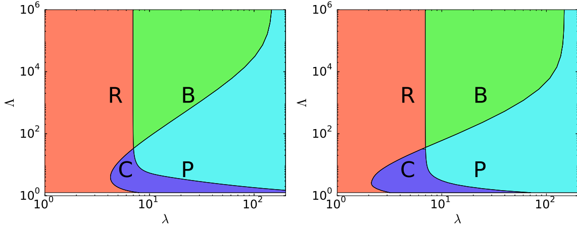
Figure 8.3: Left: Phase diagram of the transient compartmentalization dynamics with the linear selection function f_{lin}(\bar{x}) = 0.0067 + \bar{x} in the (\lambda, \Lambda) plane. Right: idem with the sigmoidal selection function f(\bar{x}) . Phases are R: pure Ribozyme, B: Bistable, C: Coexistence and P: pure Parasite.
