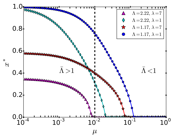
Figure 8.9: Steady state composition x^* as function of \mu , \alpha = 0.99, \gamma = 1.0 . Critical rates \mu^* corresponds to separation between P and C phases in Fig. 8.10. Separatrices are drawn for \mu values close to \mu^* in Fig. 8.9, corresponding to an error catastrophe.
