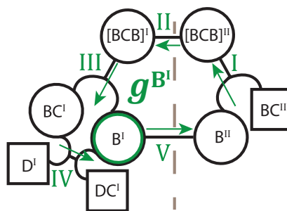
Figure 5.6: A reaction network exhibiting autocatalytic exchange. A transport barrier (dashed brown line) divides two environments. An autocatalytic submatrix is obtained by removing BC^{II} , D^I , DC^I . Arrows illustrate replication cycle \mathbf{g}^{B^I} .
