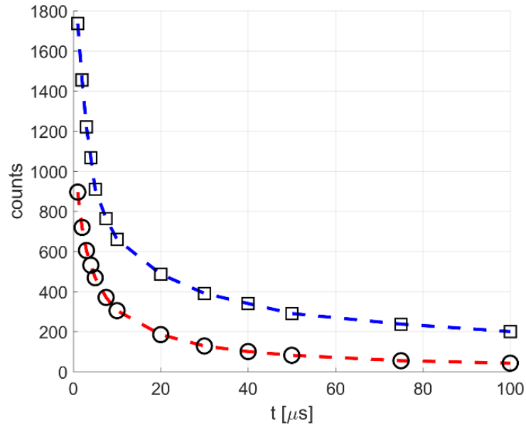
Figure 5.15. Time evolution of phosphorescence emission S_{gp}(t) for acetone (O - -) and diacetyl ( \square - -) at p = 5 kPa and T = 293 K, respectively excited at 310 and 410 nm. For all data shown in the figure, the average laser intensity is 0.08 J/cm 2 , and the recording parameters are: N_l = 100 , N_i = 10 , G = 100\% , and \Delta t_{gate} = 100 ns.
