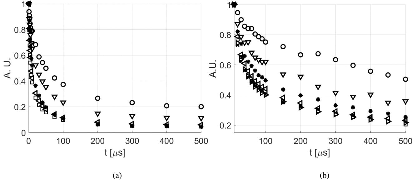
Figure 5.22. Time evolution of the TL normalized at the first time for (a) acetone vapor excited at 310 nm and (b) diacetyl vapor excited at 410 nm at different pressures: (a), p = 1 kPa (O), p = 2 kPa (▽), p = 5 kPa (*), p = 10 kPa (◁), p = 15.1 kPa (◻); (b), p = 250 Pa (O), p = 500 Pa (▽), p = 750 Pa (*), p = 1 kPa (◁), p = 1.5 kPa (◻), p = 2 kPa (▷), p = 2.5 kPa (×). The recording parameters are N_l = 100 , N_i = 10 , G = 100\% , and \Delta t_{gate} = 100 ns. For all data shown in the figure, the average laser energy density is 0.08 J/cm 2 .
