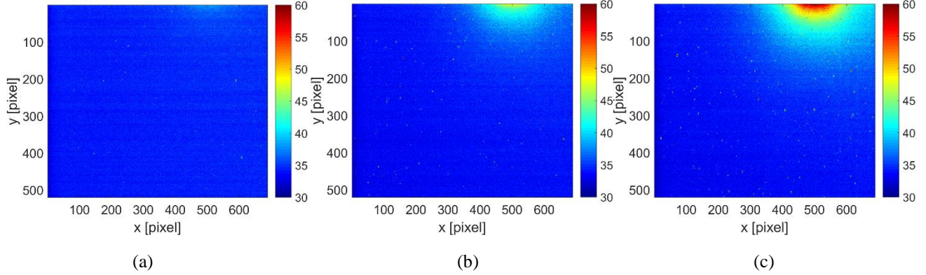
Figure 4.27. Dark images for (a) t_{CCD} = 10 \text{ s} , (b) t_{CCD} = 50 \text{ s} , (c) t_{CCD} = 100 \text{ s} . For a laser repetition rate of 10 Hz, the three exposition times correspond, respectively, to N_l = 100 , 500, and 1000.
