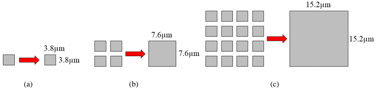
Figure 4.30. Grouping of photosites by binning: (a) 1 \times 1 , (b) 2 \times 2 , and (c) 4 \times 4 .
