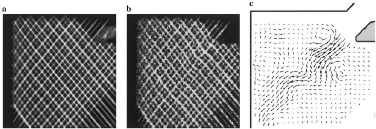
Figure 3.23. 2D-MTV applied to a nitrogen flow based on diacetyl phosphorescence: (a) Initial tagging pattern, (b) deformed tagging pattern after 50 \mu s, and (c) measured velocity vector field. Figure from Stier & Koochesfahani (1999).
