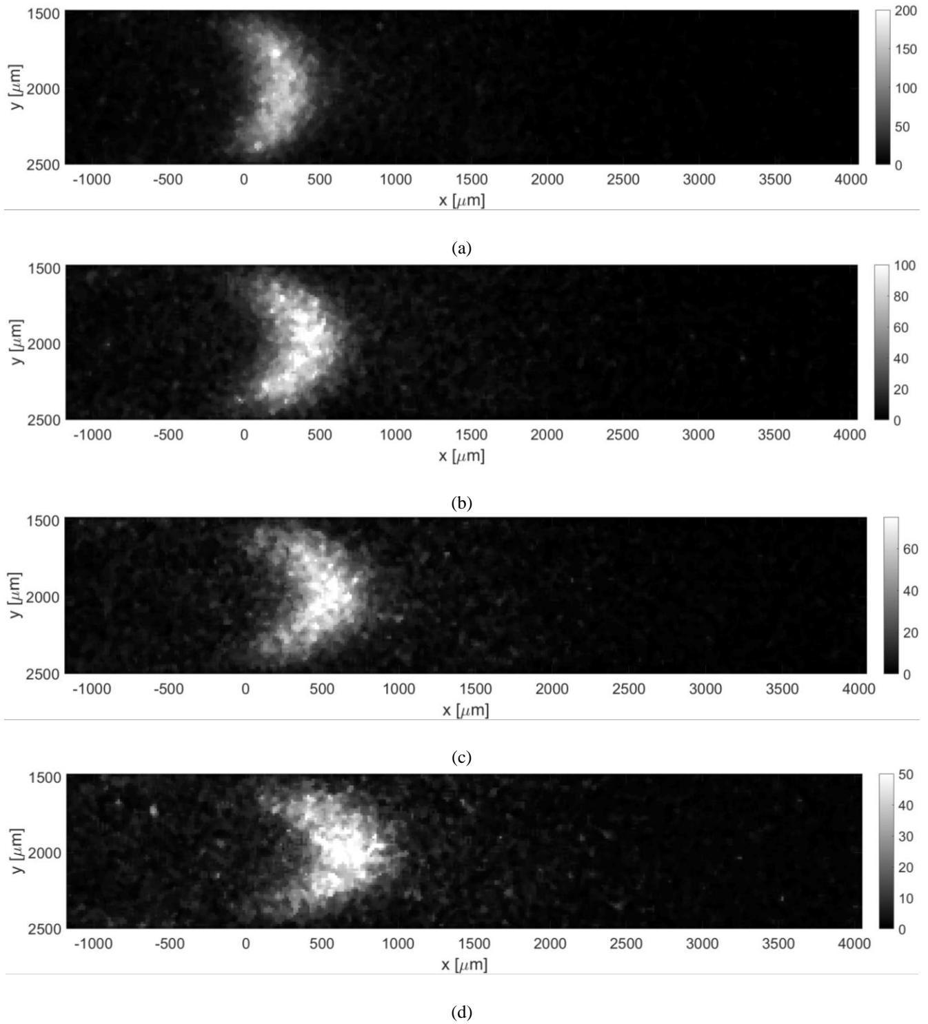
Figure 6.33. MTV acquisitions of argon-acetone flow with \chi = 20\% : (a) t = 20 \mu\text{s} , p_c = 6904 \text{ Pa} , and \Delta p = 372.7 \text{ Pa} ; (b) t = 30 \mu\text{s} , p_c = 6620 \text{ Pa} , and \Delta p = 368.4 \text{ Pa} ; (c) t = 40 \mu\text{s} , p_c = 6336.5 \text{ Pa} , and \Delta p = 364 \text{ Pa} ; (d) t = 50 \mu\text{s} , p_c = 6071 \text{ Pa} , and \Delta p = 359.5 \text{ Pa} . The recording parameters are: N_l = 100 , N_i = 20 , G = 100\% , and \Delta t_{gate} = 100 \text{ ns} . The acquisitions are made with a 4 \times 4 binning. The laser pulse energy was varying between 20 and 30 \mu\text{J} .
