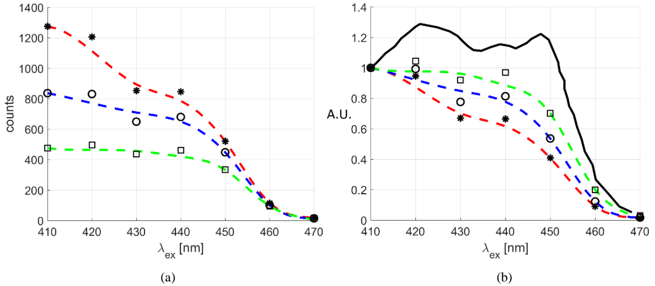
Figure 5.14. (a) Phosphorescence emission S_{gp} of diacetyl vapor at p = 5 kPa and T = 293 K as a function of the excitation wavelength and for t = 5 \mu s (*-), 10 \mu s (O--), 25 \mu s ( \square --) after the laser excitation. In (b) the same data as in (a) are normalized with respect to the light intensity emitted for an excitation at 410 nm. The average laser intensity is 0.04 J/cm 2 , and the recording parameters are: N_l = 100 , N_i = 10 , G = 100\% , and \Delta t_{gate} = 100 ns. The black solid line represents the absorption spectrum of diacetyl, taken from Stier and Koochesfahani (1999).
