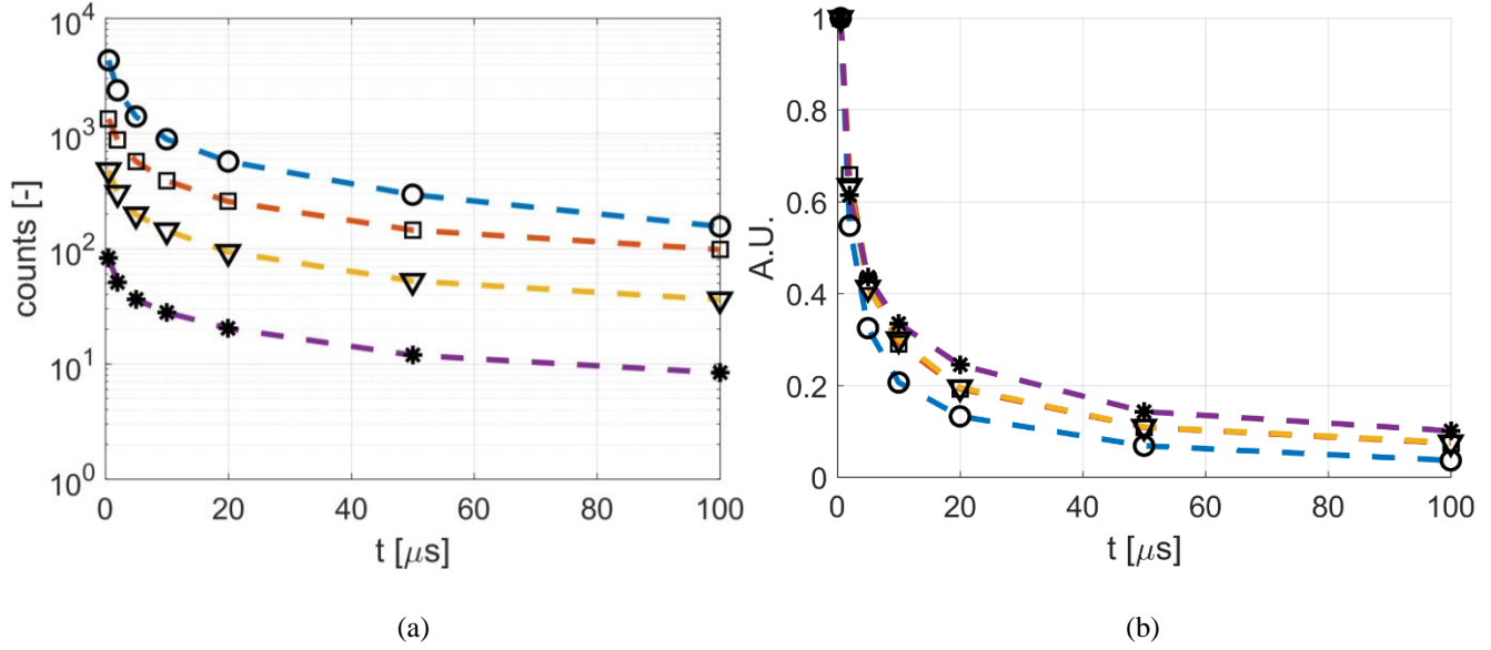
Figure 5.9. Time evolution of phosphorescence emission S_{gp}(t) for acetone vapor excited at 266 nm in helium mixture at p = 10 kPa, T = 293 K, and \chi = 100\% (O - -), 75% ( \square - -), 50% ( \nabla - -), and 25% ( \ast - -): (a) logarithmic of the signal intensity; (b) data normalized at the first delay time t = 550 ns. The average laser intensity is about \bar{I}_{in} = 0.08 J/cm 2 , and the recording parameters are: N_l = 500 , N_i = 10 , G = 100\% , and \Delta t_{gate} = 500 ns.
