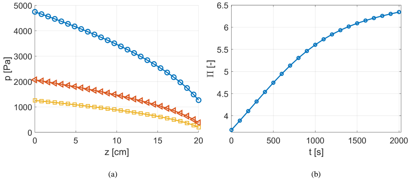
Figure 6.13. (a) Pressure distribution p(x, t) along the channel length at three different times t = 0, 1000 , and 2000 s during the experimental run, which correspond to the pressure ratios \Pi = 4 (O), 6 ( \triangleleft ), and 7 ( \square ); (b) Time evolution of the pressure ratio \Pi(t) during the experimental run.
