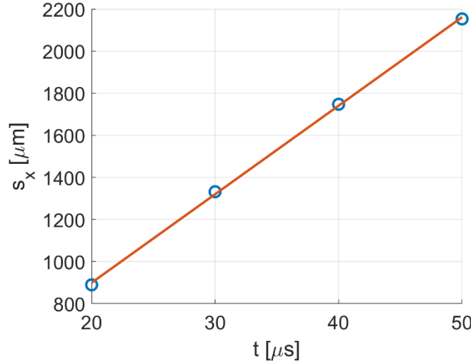
Figure 6.37. Mean molecular displacement \bar{s}_x = 889.36, 1331.77, 1747.47, 2153.04 \mu\text{m} in helium flow, respectively, at times t = 20, 30, 40 , and 50 \mu\text{s} . The red solid line represents the linear interpolation of the MTV data, which provides an average velocity \bar{u}_{MTV} = 42.07 \text{ m/s} .
