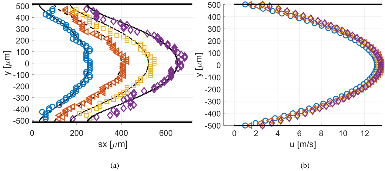
Figure 6.34. (a) Displacement data computed by applying the Gaussian fitting per line to the images of Figure 6.33; velocity reconstruction from the displacement data in (b): t = 20 \mu\text{s} (○), 30 \mu\text{s} (◁), 40 \mu\text{s} (◻) and 50 \mu\text{s} (◊).
