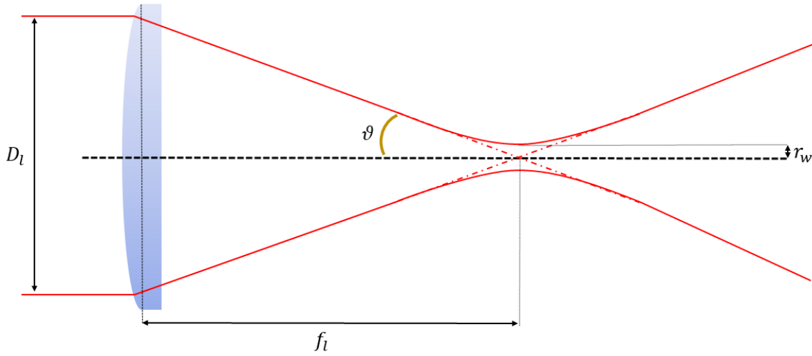
Figure 4.10. Focusing of the laser beam through the plano-convex lens.
