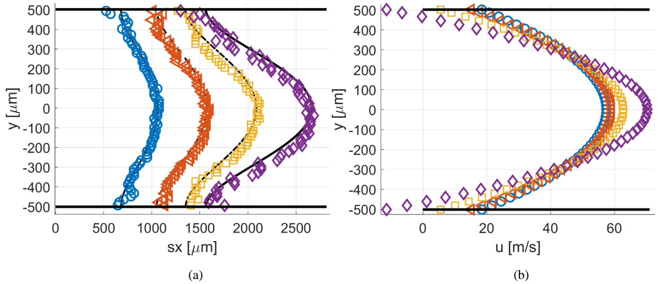
Figure 6.36. (a) Displacement data computed by applying the Gaussian fitting per line to the images of Figure 6.35; (b) velocity reconstruction from the displacement data in (b): t = 20 \mu\text{s} (O), 30 \mu\text{s} ( \triangleleft ), 40 \mu\text{s} ( \square ) and 50 \mu\text{s} ( \diamond ).
