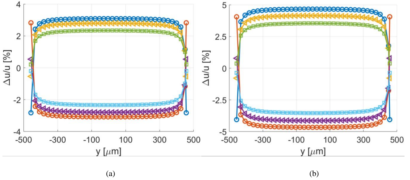
Figure 6.19. Relative variation of the velocity profile with respect to the average velocity profile (solid lines in Figure 6.18) in groups of (a) N_l = 20 and (b) N_l = 30 , and at t = 0 s (O), 1000 s (◁), and 2000 s (◻) during the experimental run.
