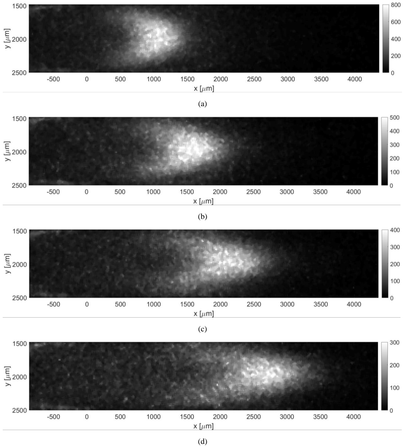
Figure 6.35. MTV acquisitions of helium-acetone flow with \chi = 20\% : (a) t = 20 \mu\text{s} , p_c = 1578.3 \text{ Pa} , and \Delta p = 1800 \text{ Pa} ; (b) t = 30 \mu\text{s} , p_c = 1582.3 \text{ Pa} , and \Delta p = 1801.6 \text{ Pa} ; (c) t = 40 \mu\text{s} , p_c = 1579.1 \text{ Pa} , and \Delta p = 1799.6 \text{ Pa} ; (d) t = 50 \mu\text{s} , p_c = 1581.2 \text{ Pa} , and \Delta p = 1800.4 \text{ Pa} . The recording parameters are: N_l = 100 , N_i = 20 , G = 100\% , and \Delta t_{gate} = 500 \text{ ns} .
