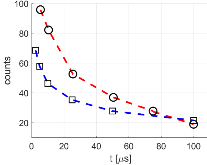
Figure 5.16. Time evolution of phosphorescence emission S_{gp}(t) in helium for acetone (O - -) and diacetyl (□ - -) at p = 1 kPa and T = 293 K. For the data on acetone emission: \lambda_{ex} = 310 nm, \chi = 5\% , N_l = 500 , N_i = 10 , G = 100\% , and \Delta t_{gate} = 500 ns. For the data on diacetyl emission: \lambda_{ex} = 410 nm, \chi = 2\% , N_l = 100 , N_i = 10 , G = 100\% , and \Delta t_{gate} = 500 ns. For all the data shown in figure, the average laser intensity is 0.08 J/cm 2 .
