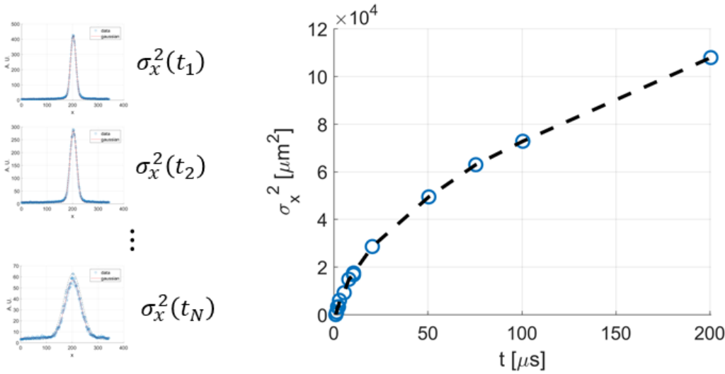
Figure 5.21. Computation of the variance \sigma_x^2 from 1D signal distribution \tilde{S}(x, t) and representation in time of the spatial distribution of the excited molecules.
