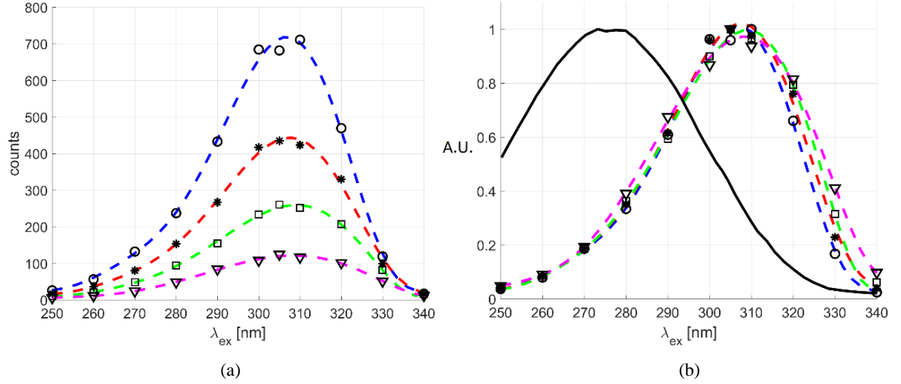
Figure 5.12. (a) Phosphorescence emission S_{gp} of acetone vapor at p = 15 kPa and T = 293 K as a function of the excitation wavelength and for t = 5 \mu s ( \bigcirc - -), 10 \mu s ( * - -), 20 \mu s ( \square - -), and 50 \mu s ( \nabla - -) after the laser excitation. In (b) the same data as in (a) are normalized with respect to the highest light intensity recorded for each delay time. The average laser intensity is 0.04 J/cm 2 , and the recording parameters are: N_l = 100 , N_i = 10 , G = 100\% , and \Delta t_{gate} = 100 ns. The black solid line is the absorption spectrum of acetone, taken from Lozano et al. (1992).
