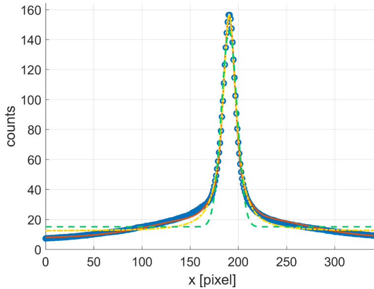
Figure B.3. Fitting of the data of Figure 2b: Gaussian fitting function (---), Lorentzian fitting function (-+), and fitting function made of a linear combination of 3 Gaussian functions (—) of the initial emission profile (○).
