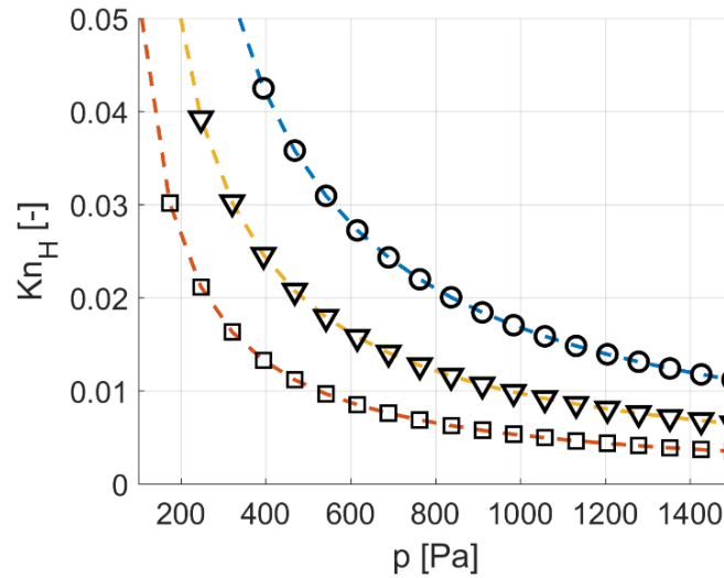
Figure 5.3. Knudsen number Kn_H as a function of the pressure p : helium (O - -), argon ( \square - -), and acetone-helium at \chi = 20\% ( \nabla - -).
