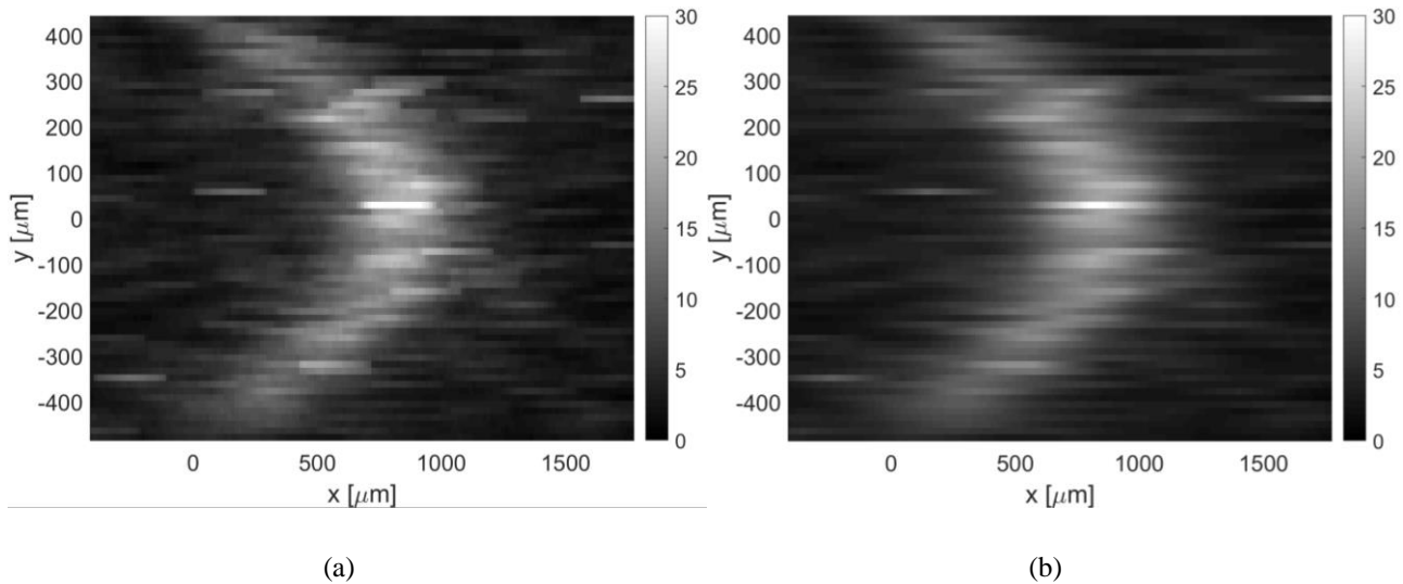
Figure 6.28. (a) Moving-average filter with a window of 20 points; (b) Gaussian filter with a window of 20 points. The filters have been applied to the image of Figure 6.27a.
