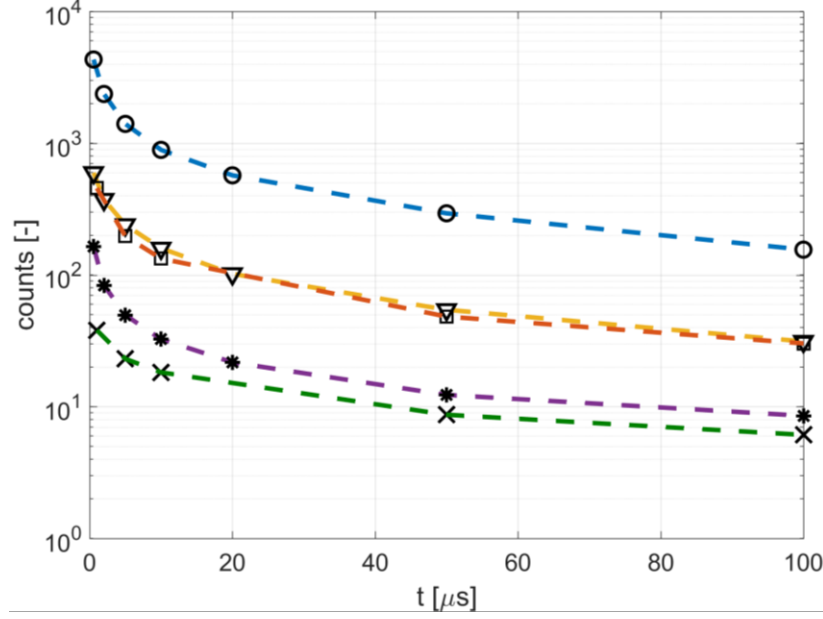
Figure 5.10. Time evolution of phosphorescence emission S_{gp}(t) for acetone vapor excited at 266 nm at T = 293 K: pure acetone at p = 10 kPa ( \circ - -), 5 kPa ( \square - -), and 2.5 kPa ( \times - -); acetone-helium mixture at p = 10 kPa and \chi = 50\% ( \nabla - -) and 25% ( * - -). The data related to acetone-helium mixture are the same of Figure 5.9. For all the data shown, the average laser intensity is about \bar{I}_{in} = 0.08 J/cm 2 , and the recording parameters are: N_l = 500 , N_i = 10 , G = 100\% , and \Delta t_{gate} = 500 ns.
