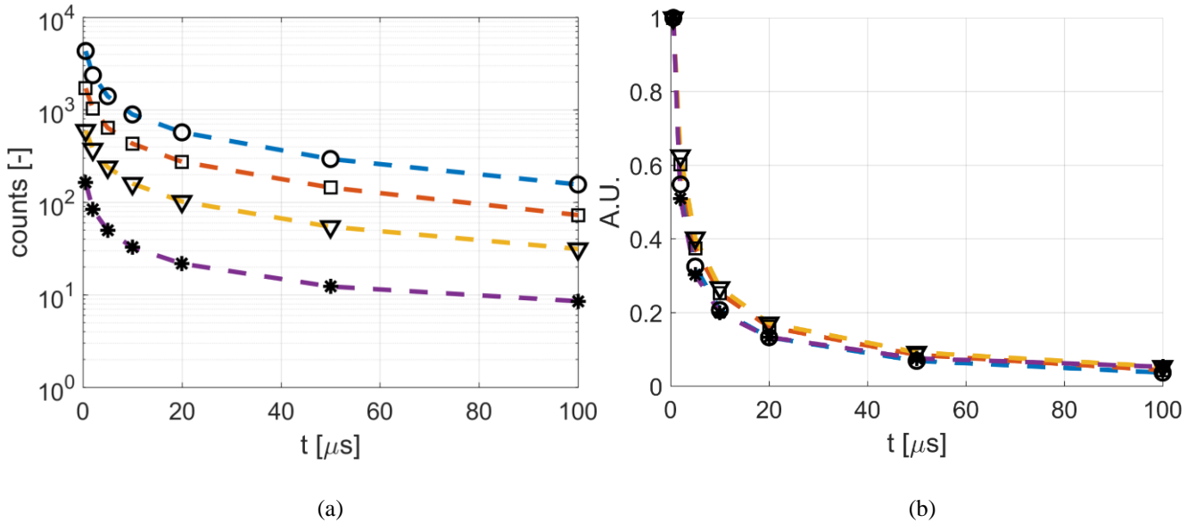
Figure 5.8. Time evolution of phosphorescence emission S_{gp}(t) for acetone vapor excited at 266 nm in argon mixture at p = 10 kPa, T = 293 K, and \chi = 100\% (O - -), 75% ( \square - -), 50% ( \nabla - -), and 25% ( * - -): (a) logarithmic of the signal intensity; (b) data normalized at the first delay time t = 550 ns. The average laser intensity is about \bar{I}_{in} = 0.08 J/cm 2 , and the recording parameters are: N_l = 500 , N_i = 10 , G = 100\% , and \Delta t_{gate} = 500 ns.
