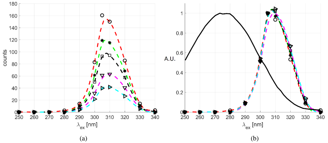
Figure 5.13. (a) Phosphorescence emission S_{gp} of acetone vapor at p = 1.5 kPa and T = 293 K as a function of the excitation wavelength and for t = 1 \mu s ( \bigcirc - -), 5 \mu s ( * - -), 10 \mu s ( \square - -), 25 \mu s ( \nabla - -), and 50 \mu s ( \triangleright - -) after the laser excitation. In (b) the same data as in (a) are normalized with respect to the highest light intensity recorded for each delay time. The average laser intensity is 0.04 J/cm 2 , and the recording parameters are: N_l = 100 , N_i = 10 , G = 100\% , and \Delta t_{gate} = 100 ns. The black solid line is the absorption spectrum of acetone, taken from Lozano et al. (1992).
