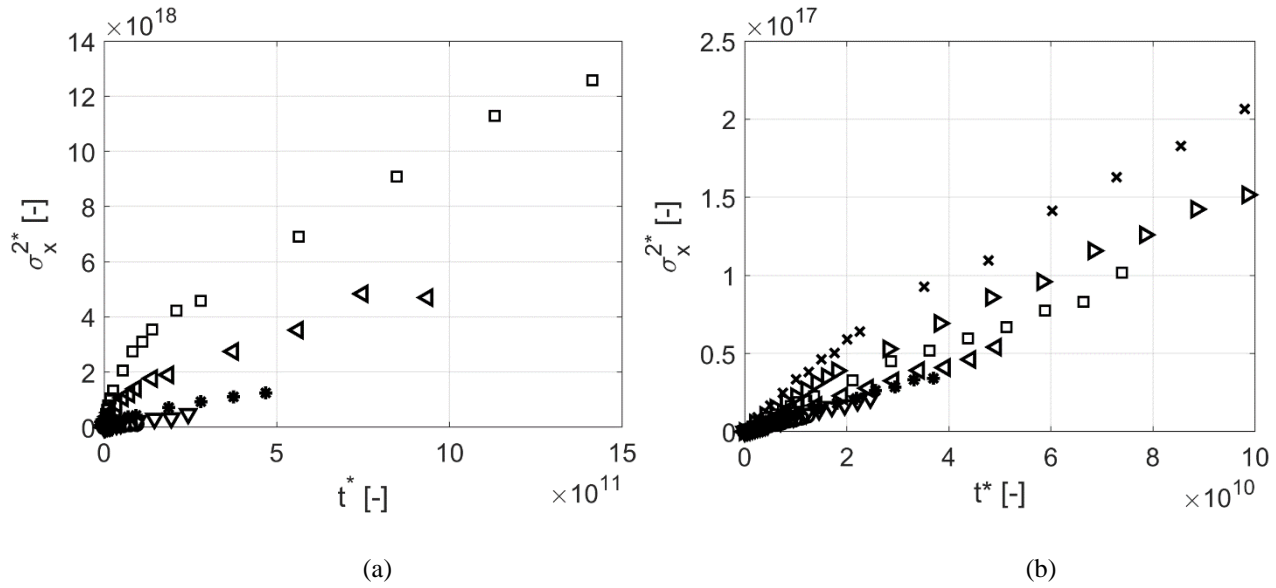
Figure 5.25. Non-dimensional variance \sigma_x^{2*}(t) as a function of the non-dimensional time t^* for (a) acetone vapor excited at 310 nm and (b) diacetyl vapor excited at 410 nm at different pressures. The reported data are the non-dimensional version of the data of Figure 5.24: in (a), p = 1 kPa (O), p = 2 kPa ( \nabla ), p = 5 kPa (*), p = 10 kPa ( \triangleleft ), p = 15.1 kPa ( \square ); in (b), p = 250 Pa (O), p = 500 Pa ( \nabla ), p = 750 Pa (*), p = 1 kPa ( \triangleleft ), p = 1.5 kPa ( \square ), p = 2 kPa ( \triangleright ), p = 2.5 kPa ( \times ).
