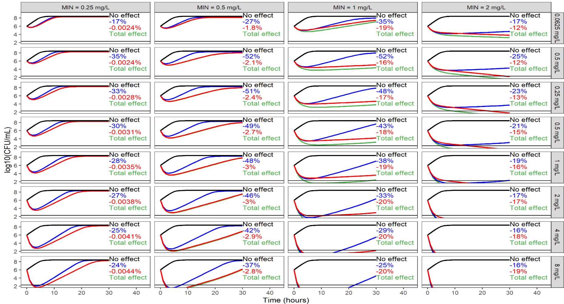
Figure S4. Simulations of CFU/mL for different model parametrisation. Simulations of expected log 10 (CFU/mL) versus time for different model parametrisations: black: absence of effect, green: under the final model; blue: under the final model with potentialization of minocycline by polymyxin B set to 0; red: under the final model with inhibition of adaptation to polymyxin B by minocycline set to 0. Percentages represent the part of the total effect imputable to the removed component. Each column corresponds to a minocycline (MIN) concentration and each line is a polymyxin B (PMB) concentration.
