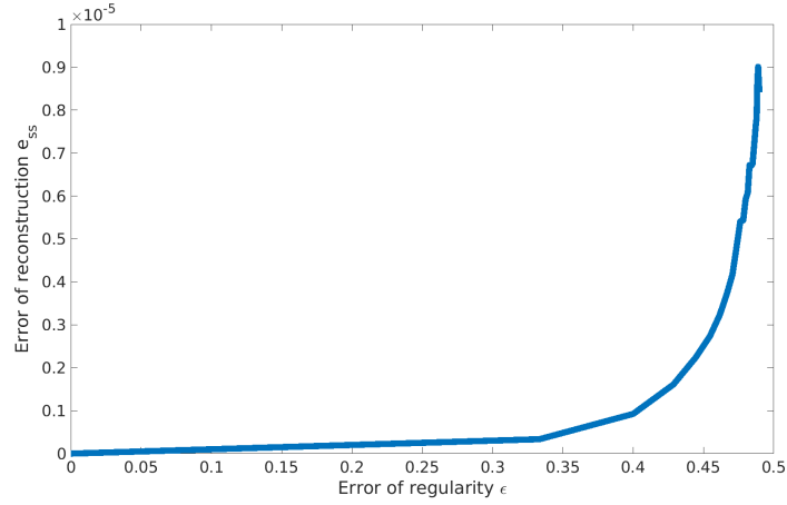
Figure 3.6: Error of reconstruction as a function of the error regularity for the family of p -reg network. For each p \in [1, \dots, 100] , 25 p -reg network are generated with different inputs. The error of reconstruction is then computed as the bias between the signal and the reconstruction at t = 1000 (which is a good approximation of e_{ss} ). This emphasizes the link between the regularity of a subgraph and the ability to reconstruct its average.
